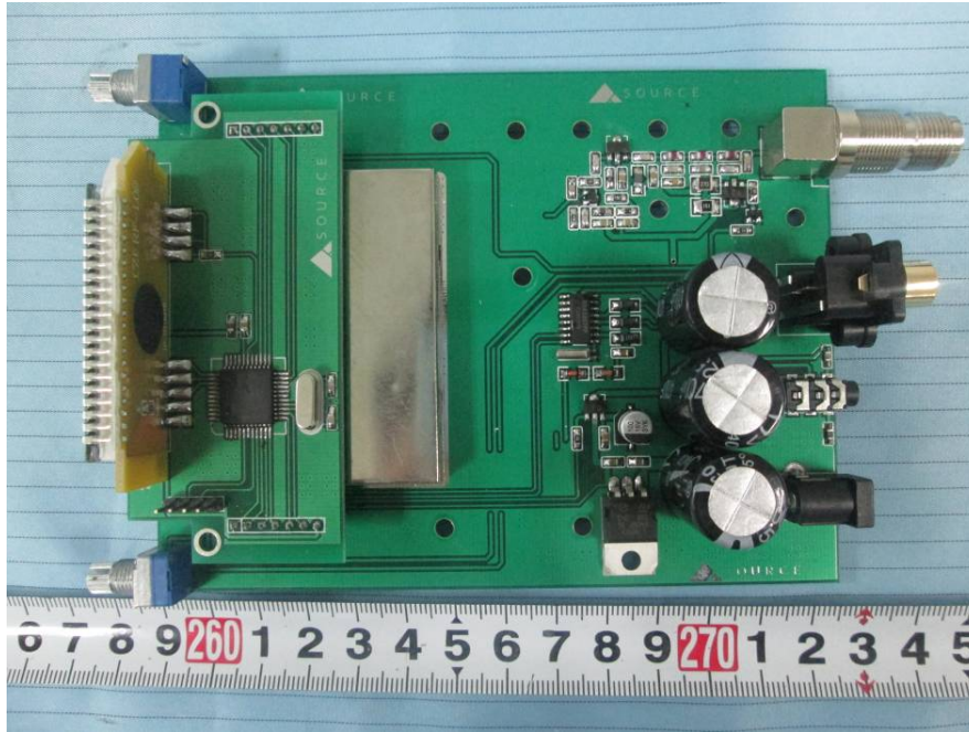
EUT – The All Board Top View
