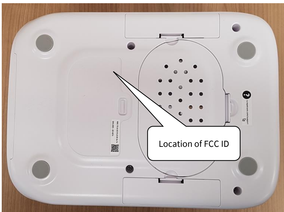
Location of FCC ID on underside of product
