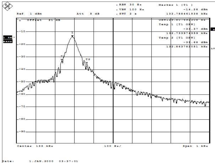
Figure 2 - Emission Bandwidth
