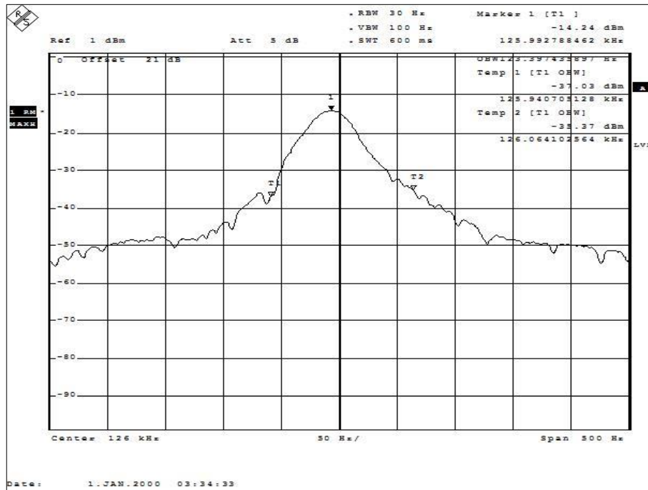
Figure 1 - Emission Bandwidth
