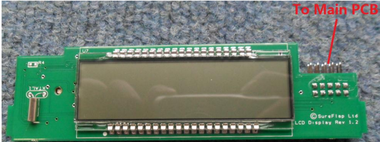
Display Board Bottom
