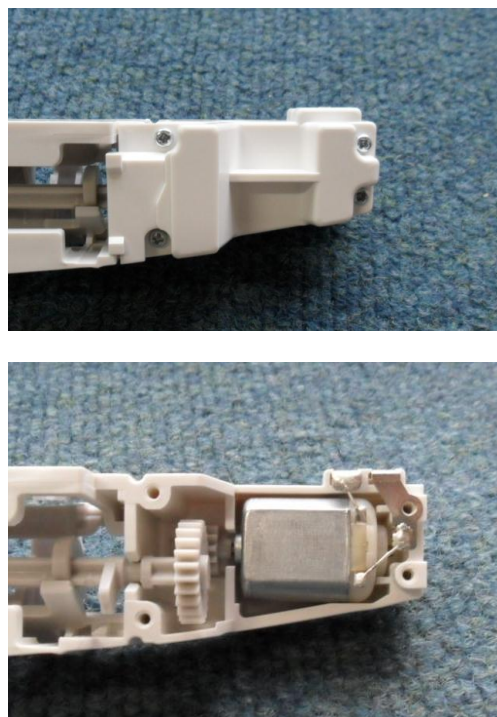
Motorised Lock (Back view)
