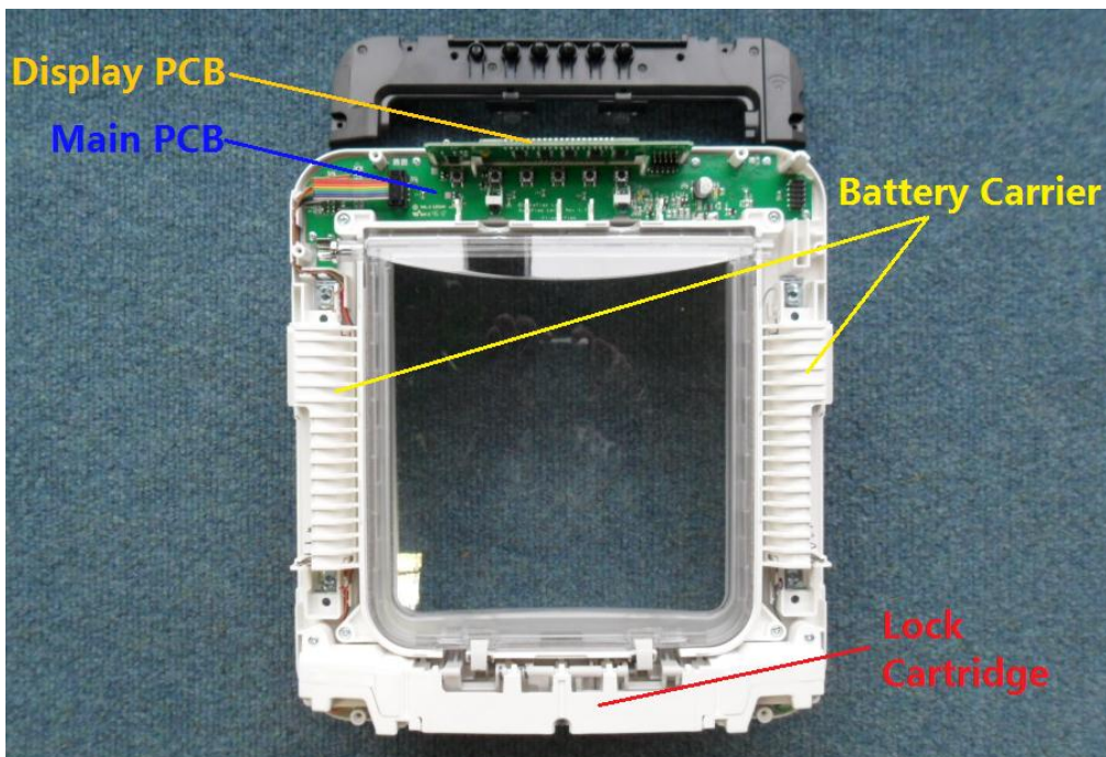
PCB cover removed
