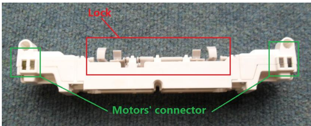
Motorised Lock (Back view)
