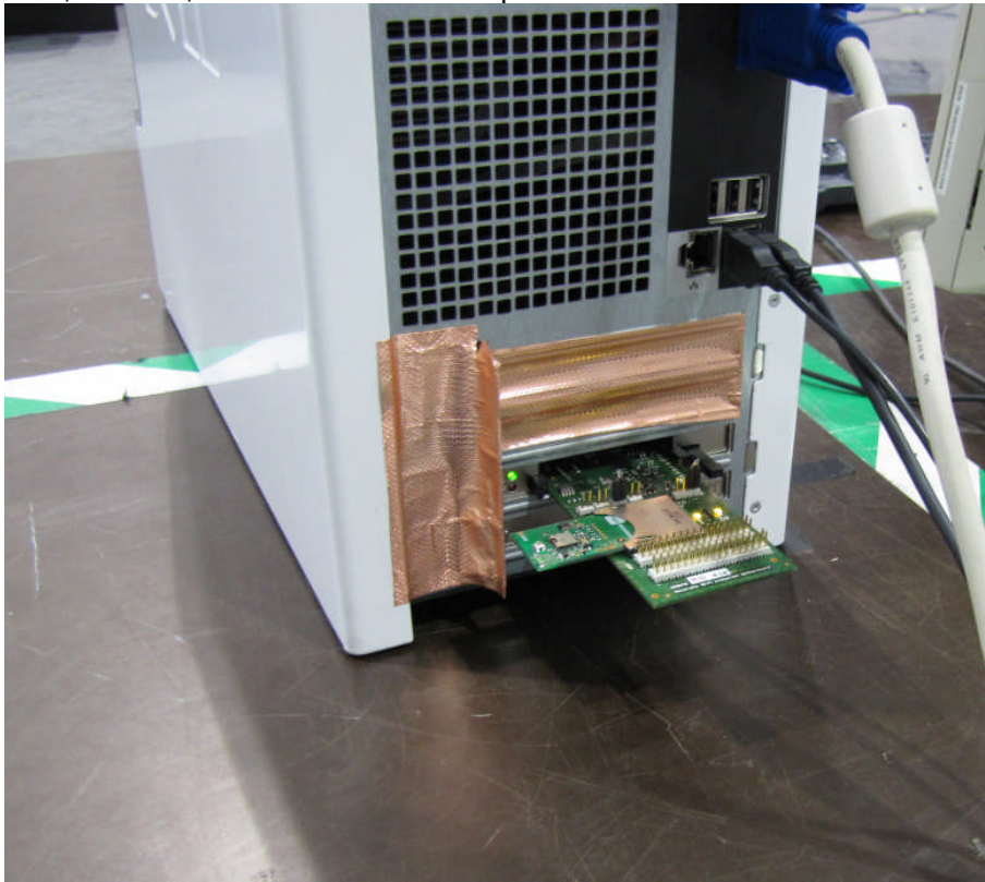
EUT, SD-card, PCMCIA-card and computer
