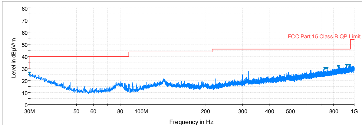
Plot 7-26. Radiated Spurious Plot below 1GHz (802.11a – U3 Ch. 157, Ant. Pol. H)
