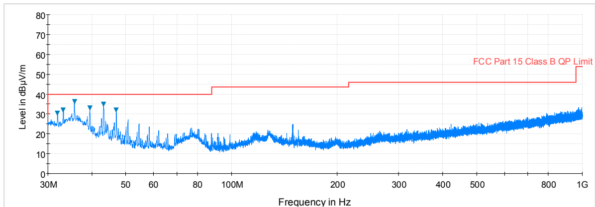
Plot 7-27. Radiated Spurious Plot below 1GHz (802.11a – U3 Ch. 157, Ant. Pol. V)
