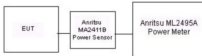
Figure 7-1. Test Instrument & Measurement Setup for Power Meter Measurements
