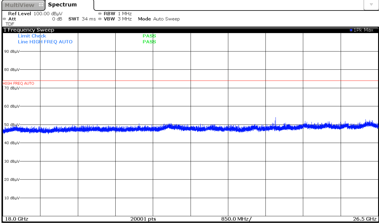
Plot 7-7. Radiated Spurious Plot above 18GHz (Pol. H)
