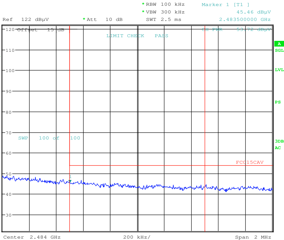
Plot 7-19. Radiated Restricted Upper Band Edge Measurement (Average)
