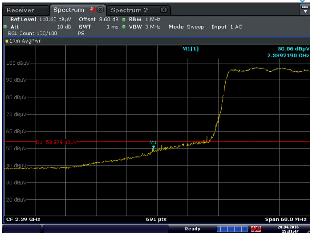
Plot 7-51. Radiated Restricted Lower Band Edge Measurement (Average)
