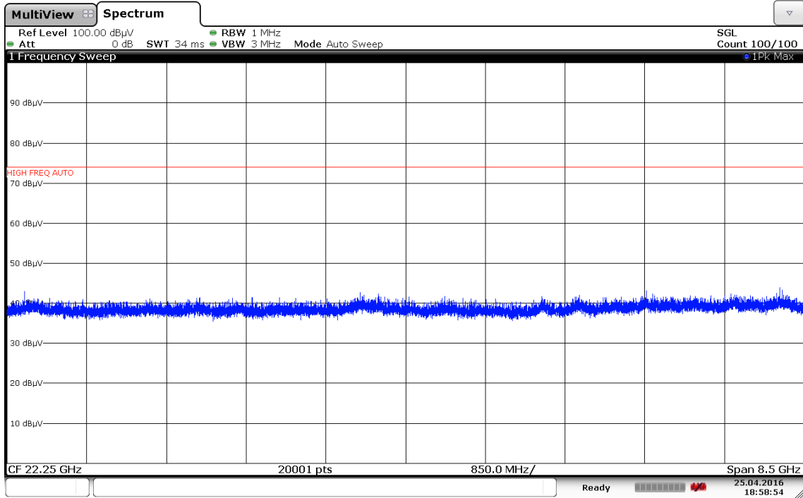
Plot 7-49. Radiated Spurious Plot above 18GHz (Pol. H)
