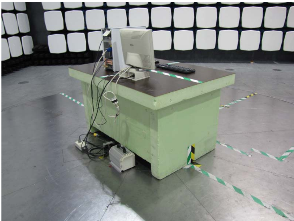
Test set-up photos 30 -1000 MHz
