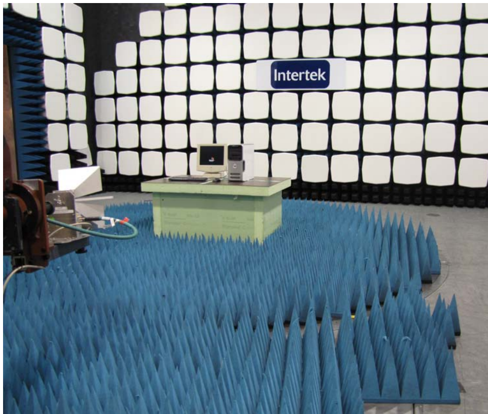
Test set-up photo above 1 GHz
