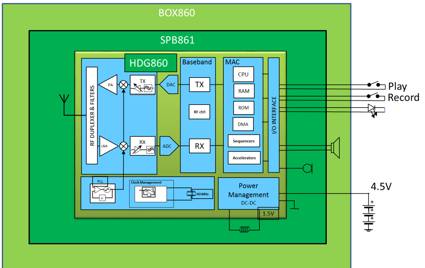
Figure 1-1 Block Diagram:
