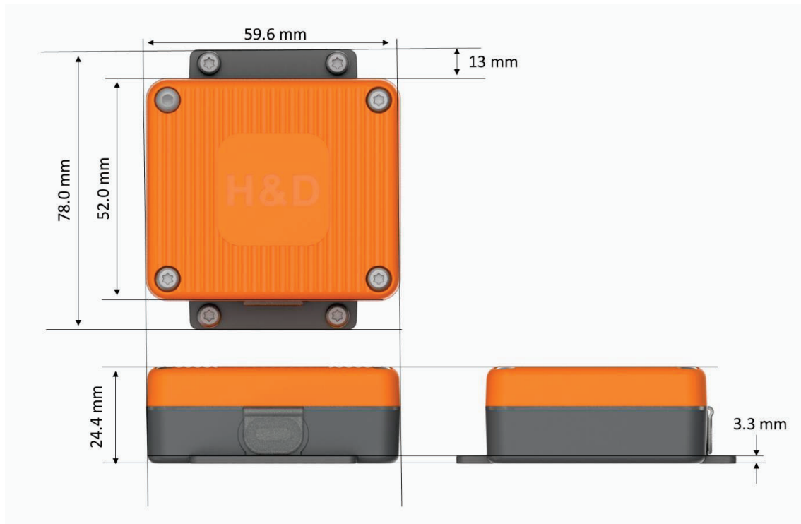
Figure 5-2: BOX827 with mounting flanges
