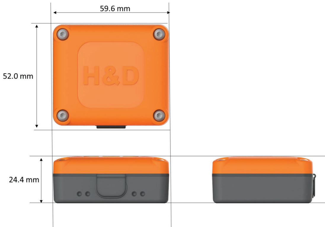
Figure 5-1: BOX827 without mounting flanges
