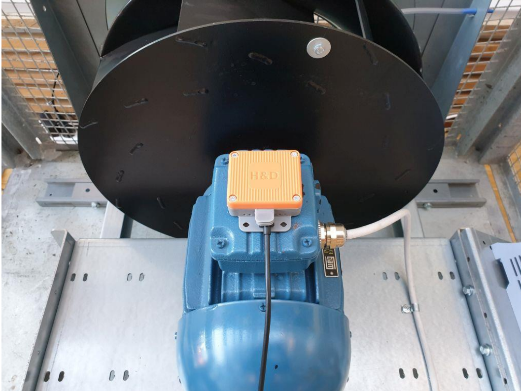
Figure 3. BOX827 mounted on an electric fan.
