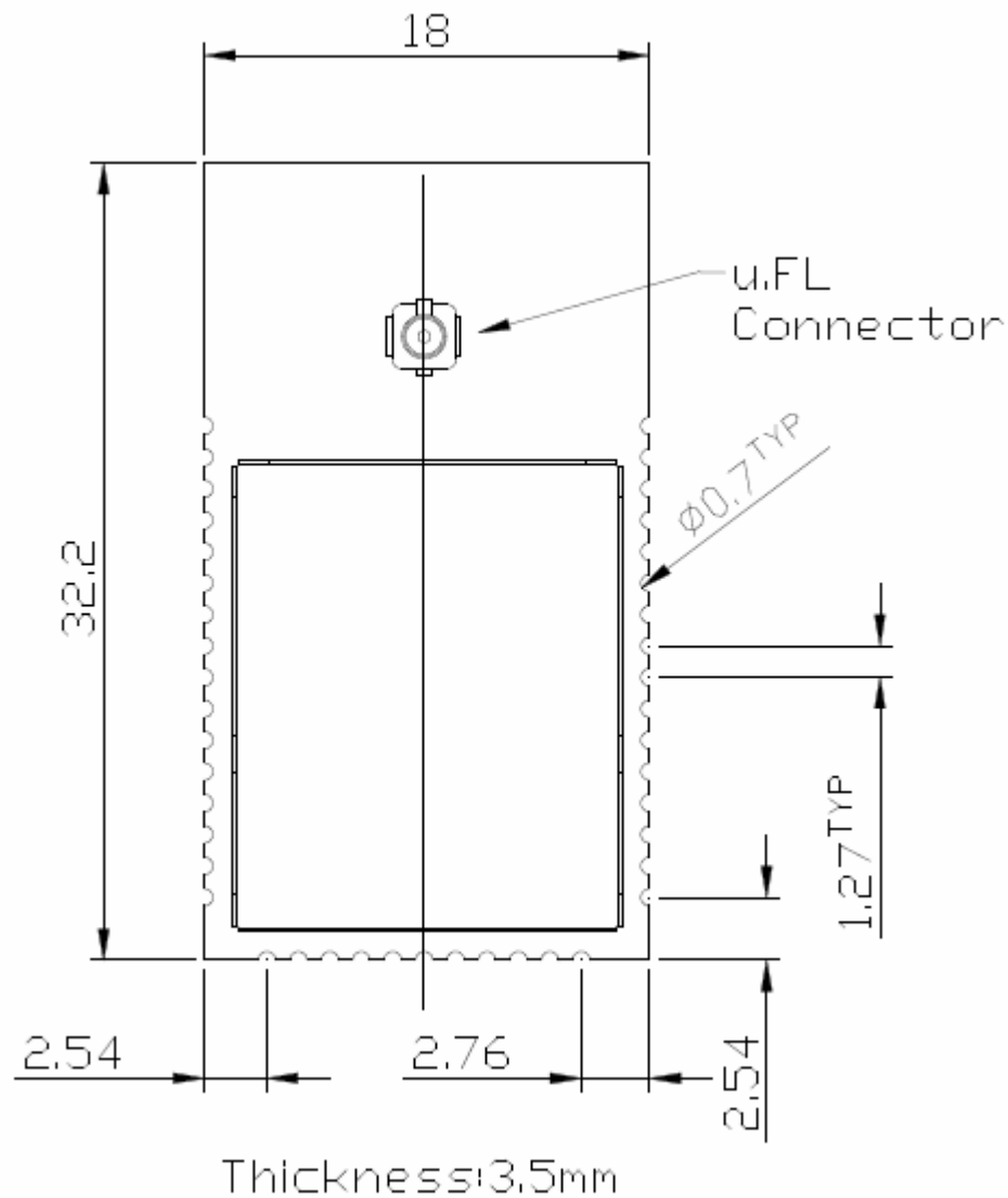
Figure : MD-102FC-5148A Outline Drawing
