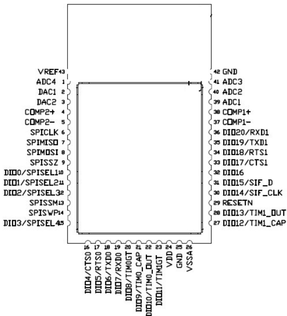
Figure : MD-102FC-5148A Pin Configuration(Top View)
