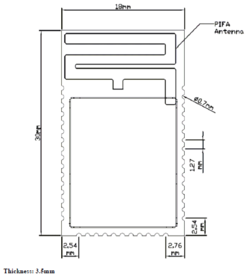
Figure: MD-102AD Outline Drawing
