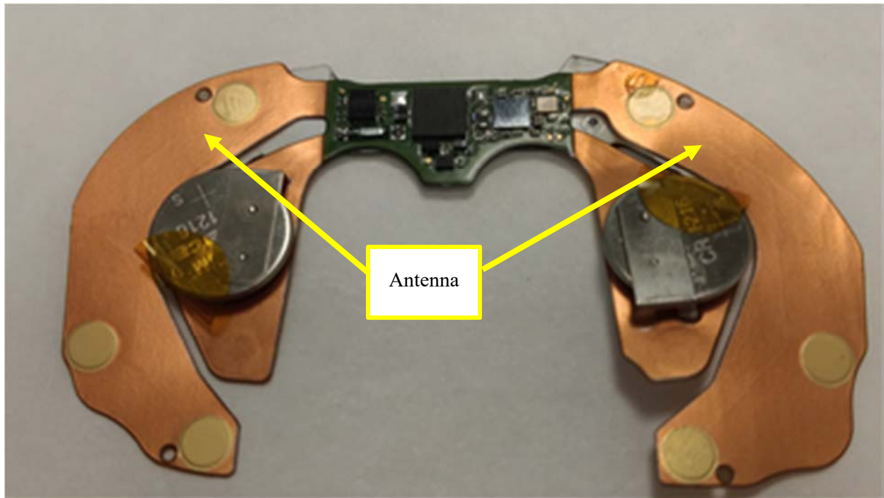
Figure 1: Top View with Case-Back in Removed.
