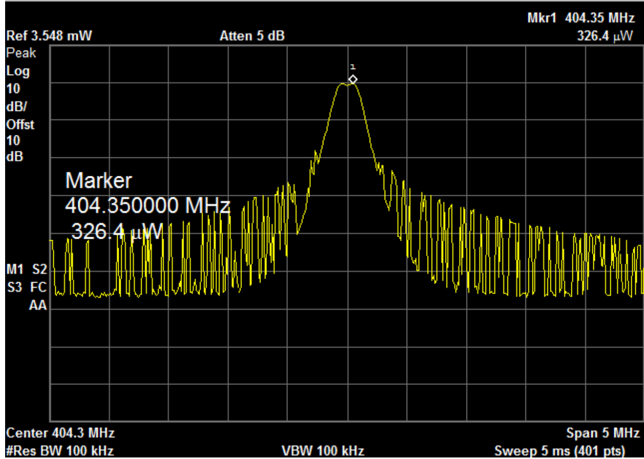
Plot 1 – Output Power
