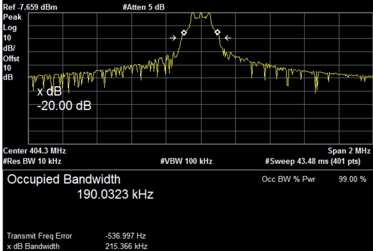
Plot 5 – Emission Bandwidth
