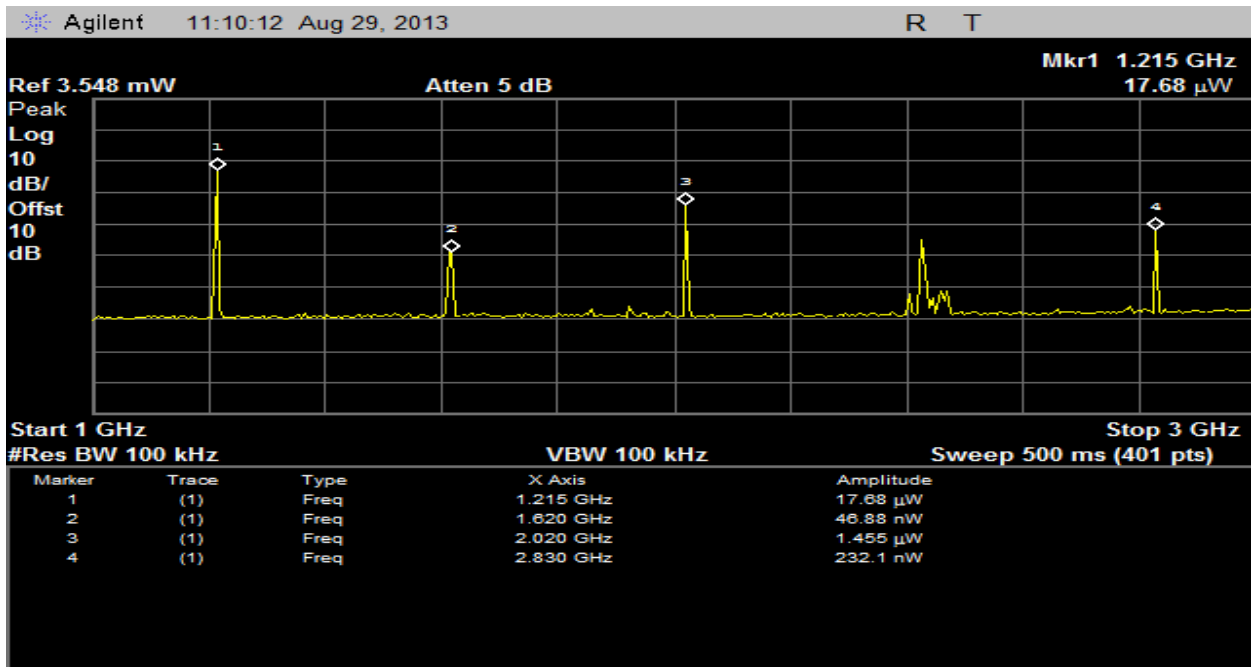
Plot 10 – 1GHz to 3 GHz
