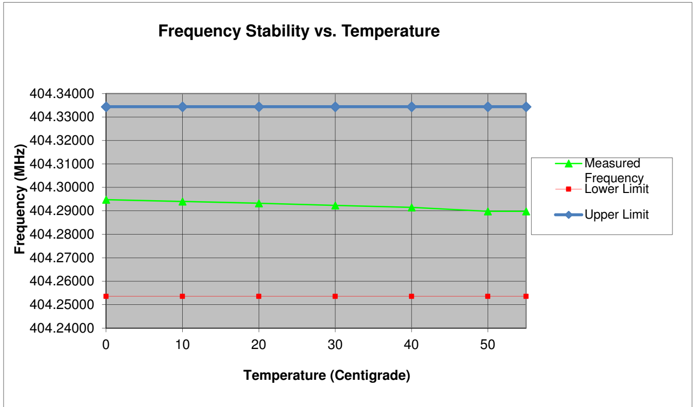
Plot 14 – Temperature vs Frequency
