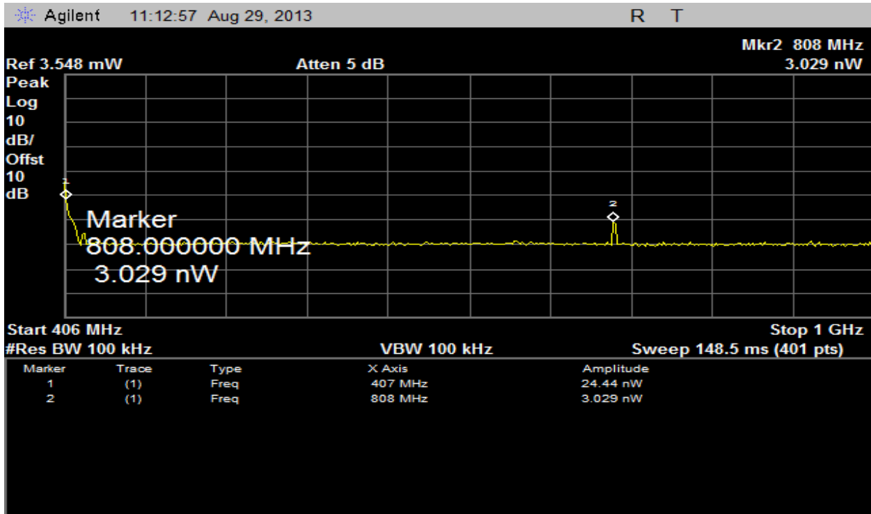
Plot 9 – 406MHz to 1GHz
