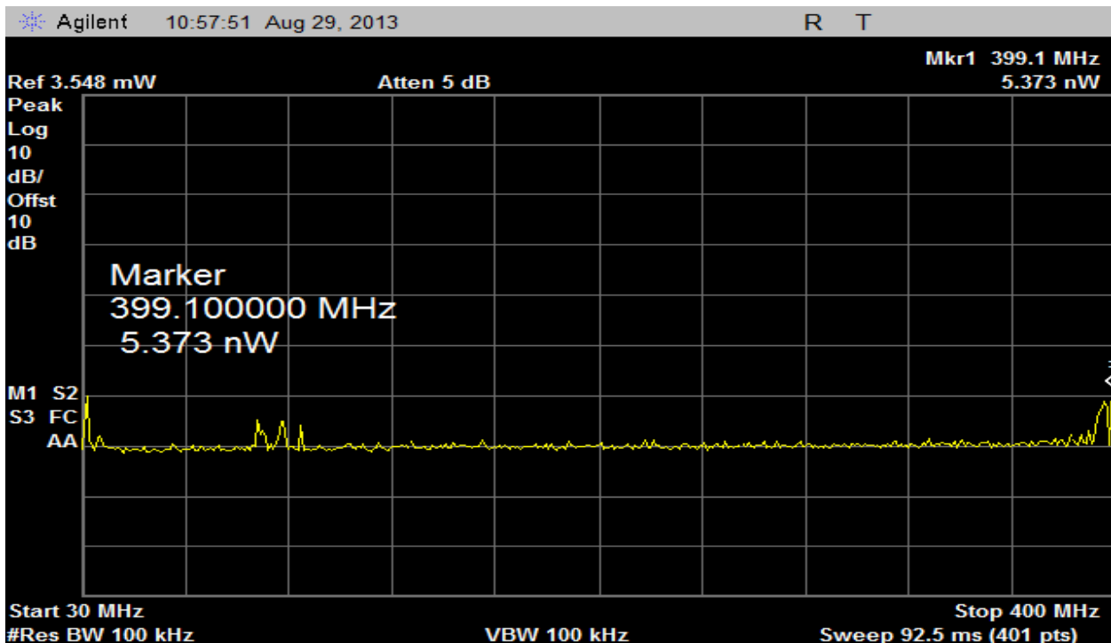
Plot 8 –30MHz to 400MHz
