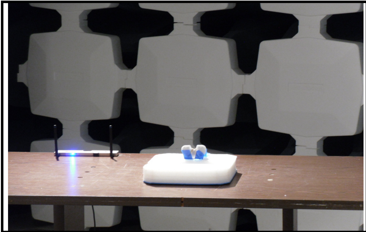
Test Setup Photo # 3 – Radiated Emissions
