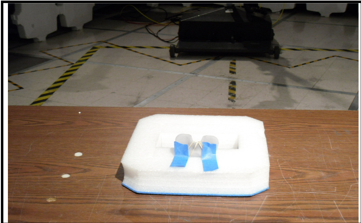
Test Setup Photo # 4 – Radiated Emissions
