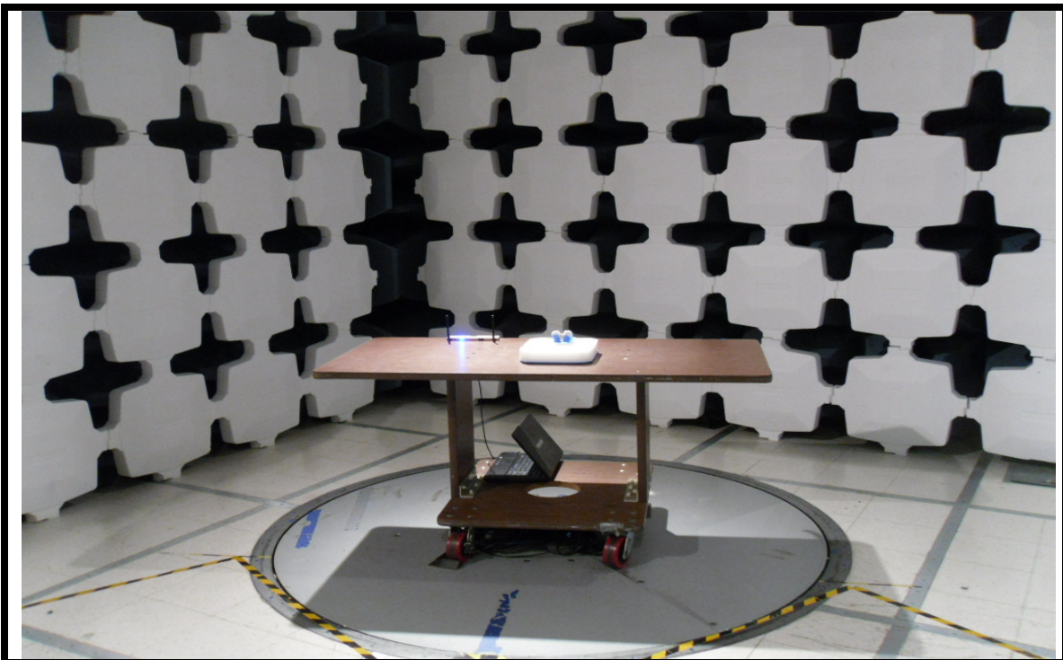
Test Setup Photo # 2 – Radiated Emissions
