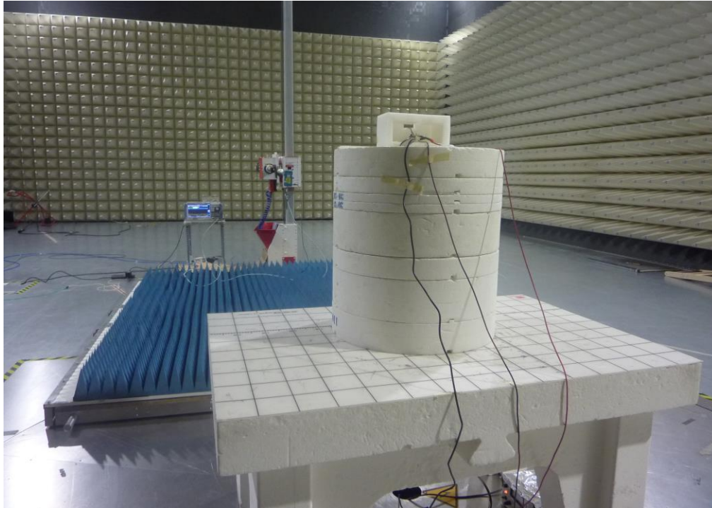
Figure 11: Test Setup for 18 GHz to 26 GHz (Rear View)
