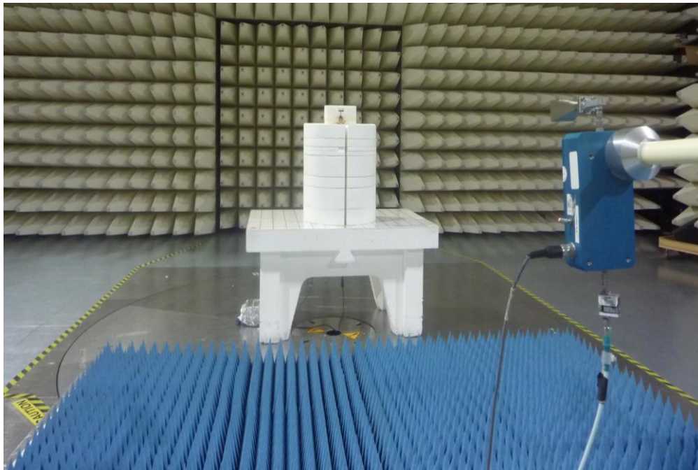
Figure 12: Test Setup for 18 GHz to 26 GHz (Front View)
