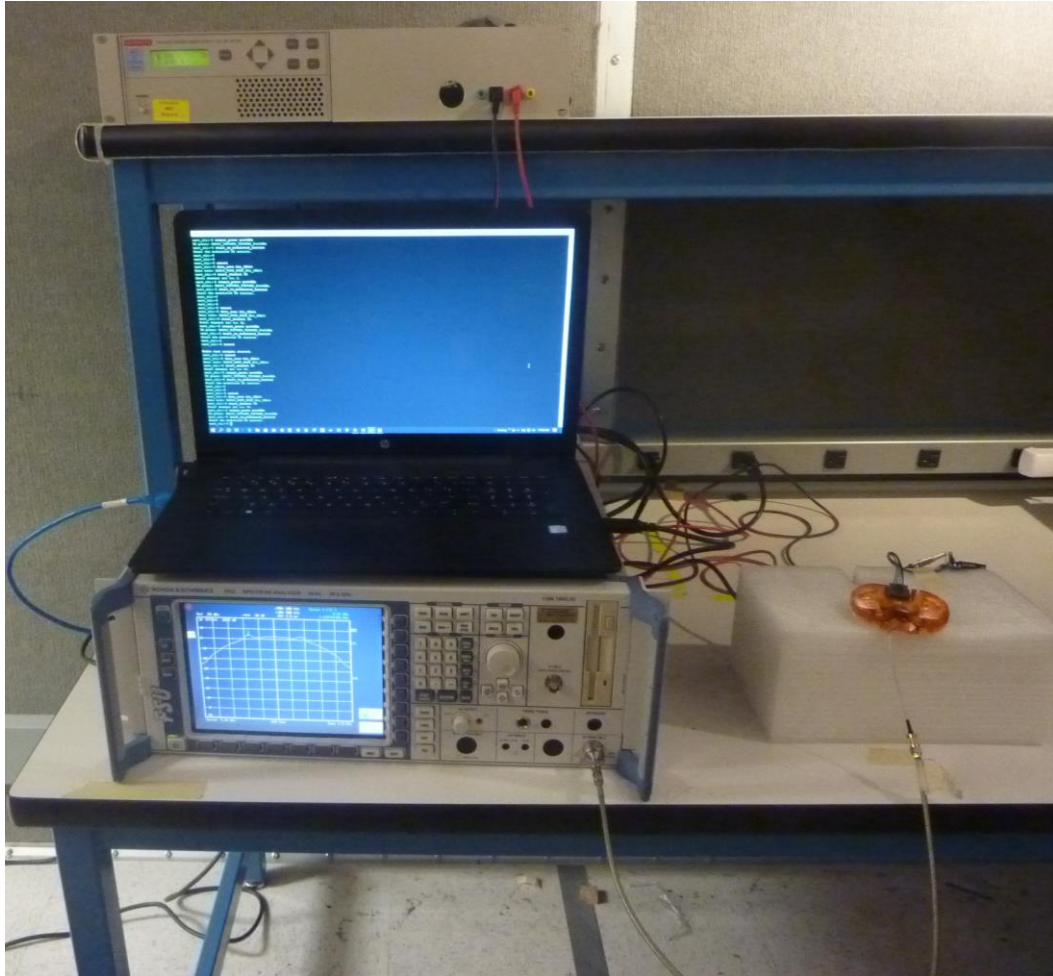
Figure 1: Test Setup for RF conducted measurements
