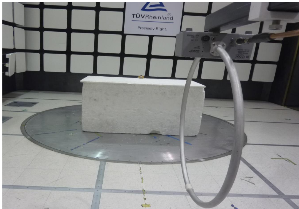
Figure 6: Test Setup for 9 kHz to 30 MHz (Front View – Antenna 90°)
