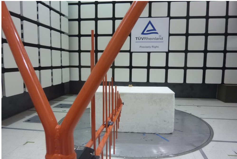
Figure 8: Test Setup for 30 MHz to 1 GHz (Front View)
