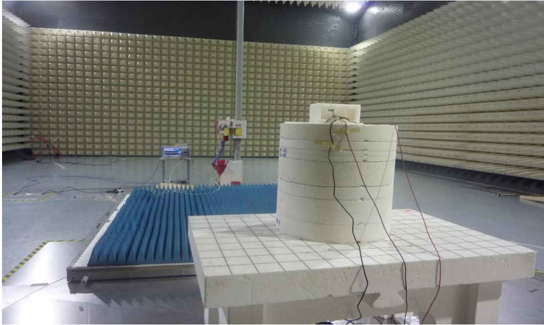
Figure 9: Test Setup for 1 GHz to 18 GHz (Rear View)
