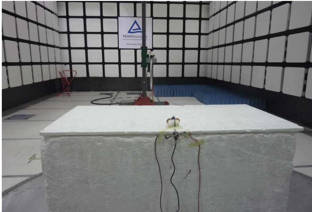
Figure 5: Test Setup for 9 kHz to 30 MHz (Rear View – Antenna 90°)
