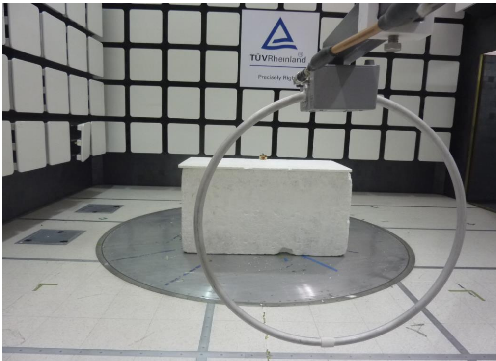
Figure 4: Test Setup for 9 kHz to 30 MHz (Front View – Antenna 0°)
