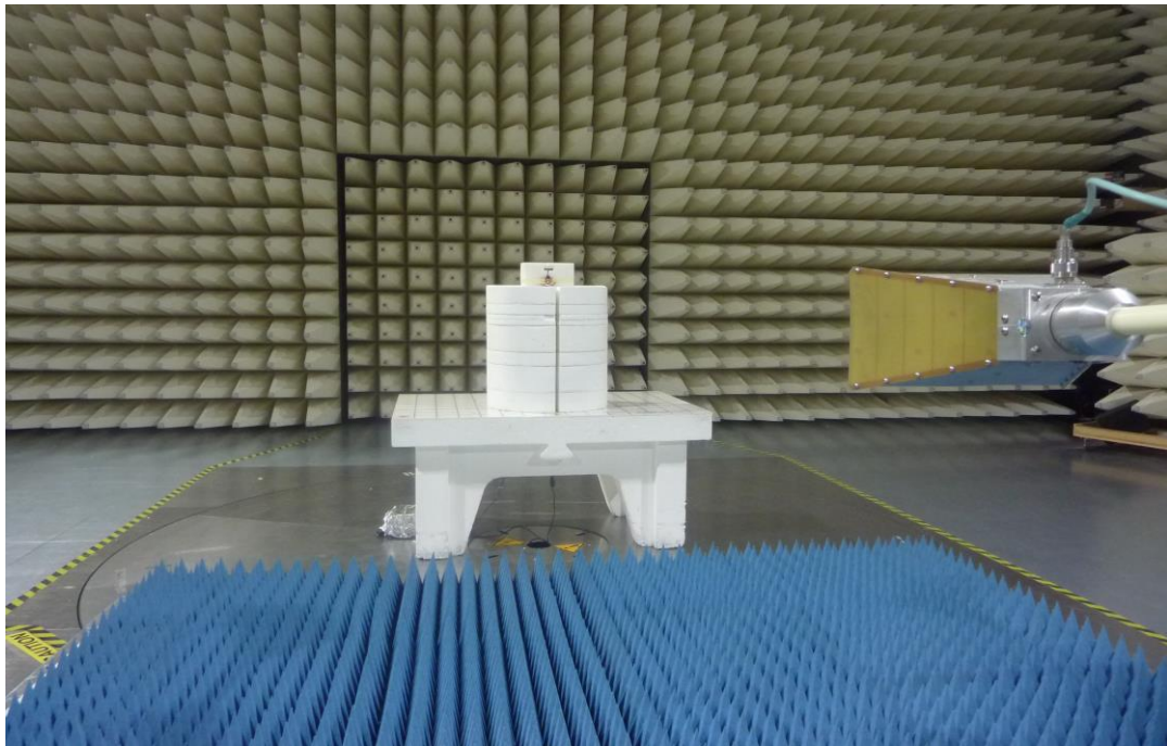
Figure 10: Test Setup for 1 GHz to 18 GHz (Front View)
