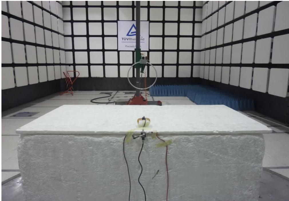
Figure 3: Test Setup for 9 kHz to 30 MHz (Rear View – Antenna 0°)
