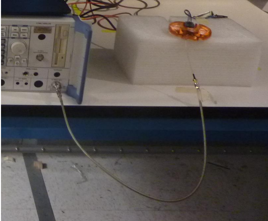
Figure 2: Test Setup for conducted measurements at connector - detail
