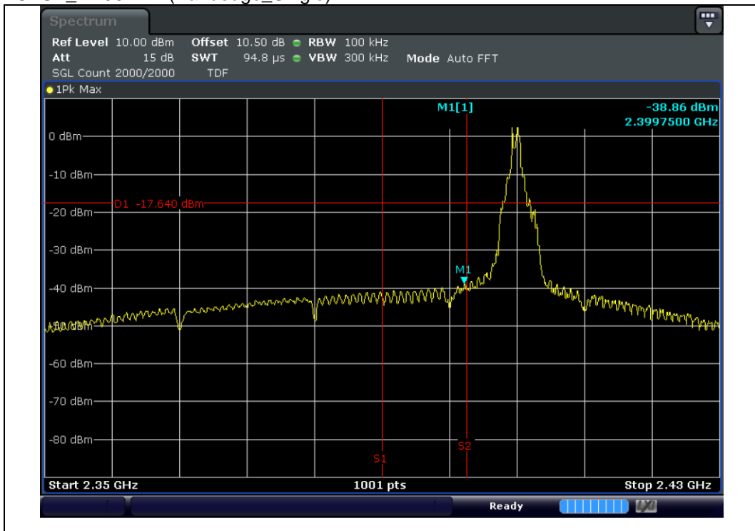
GFSK_2 406 MHz(Bandedge_Single)
