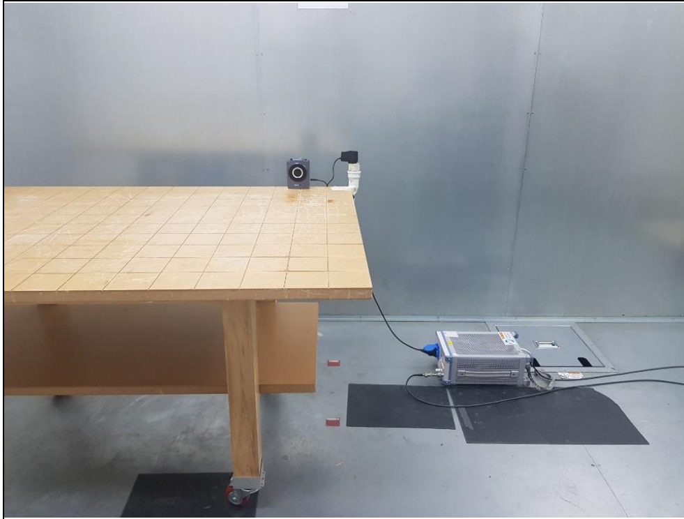
Conducted Emission
