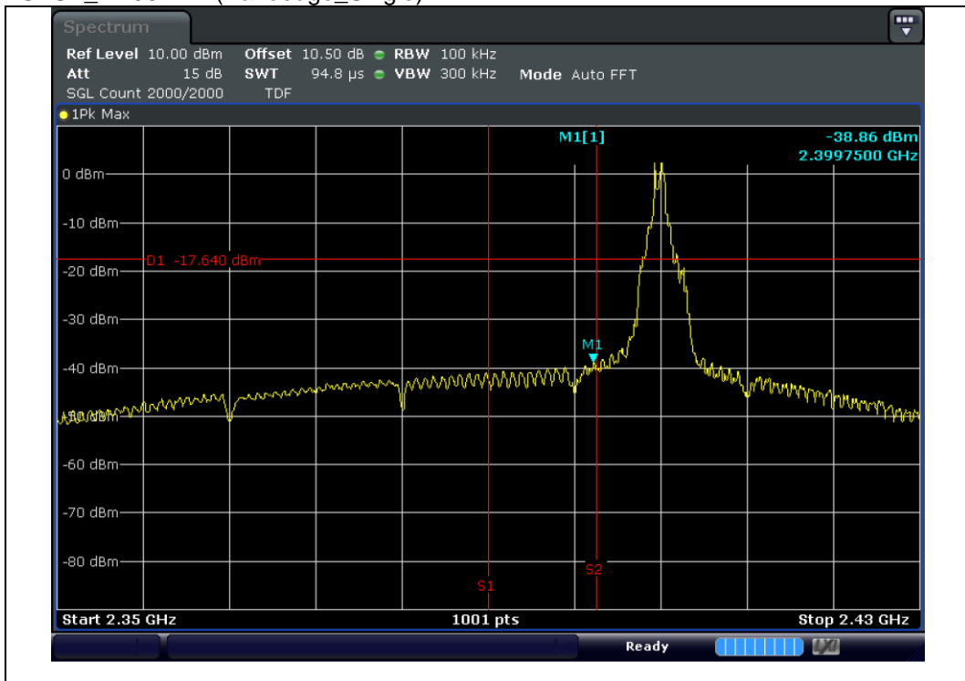
GFSK_2 406 MHz(Bandedge_Single)
