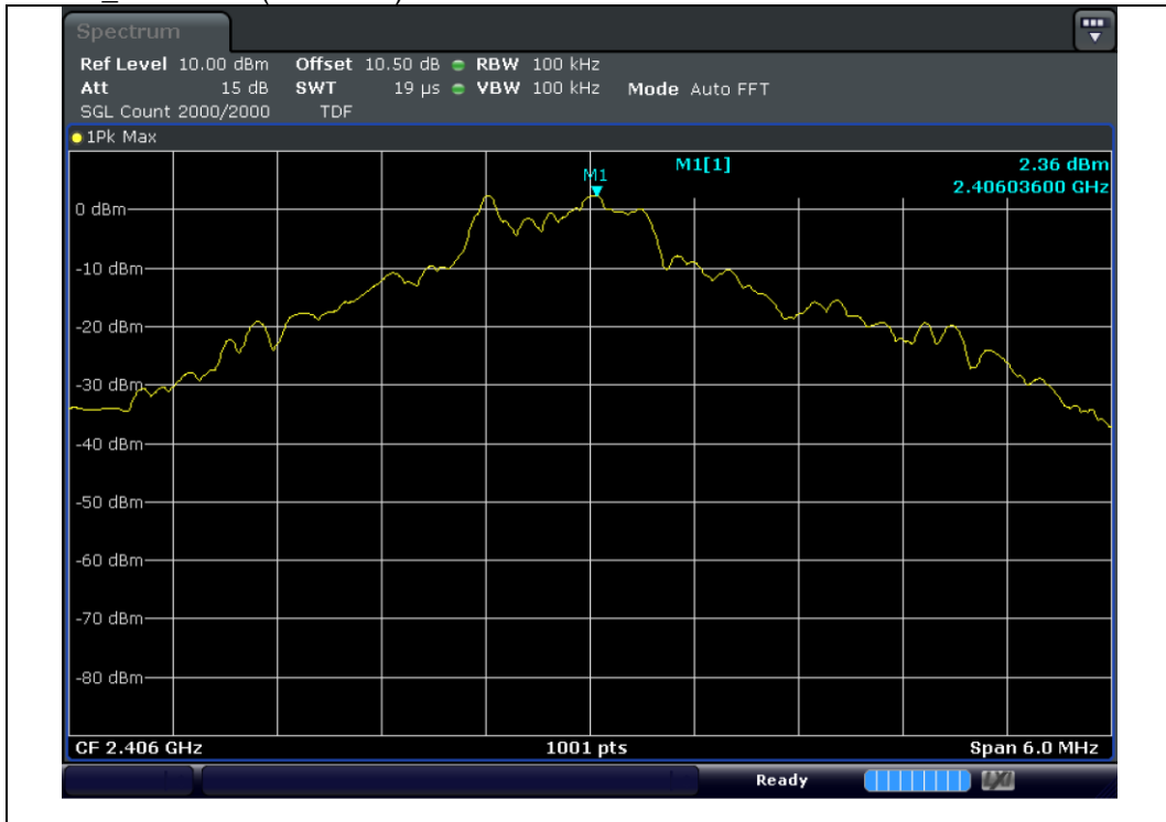
GFSK_2 406 MHz(reference)
