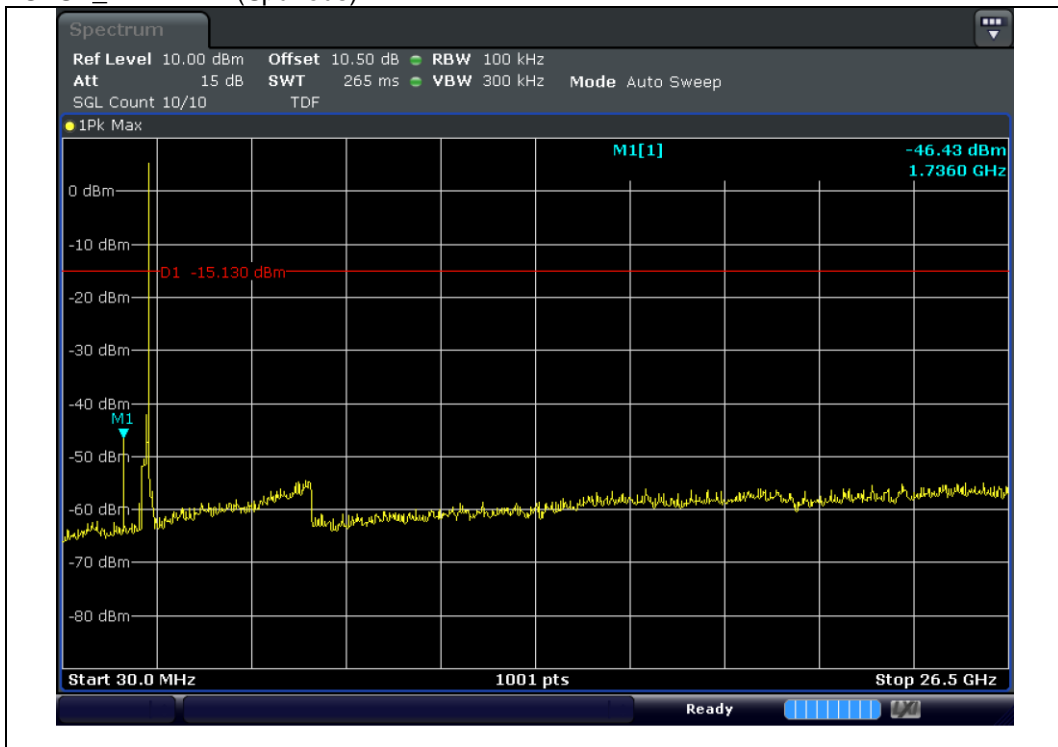
GFSK_2 442 MHz(Spurious)
