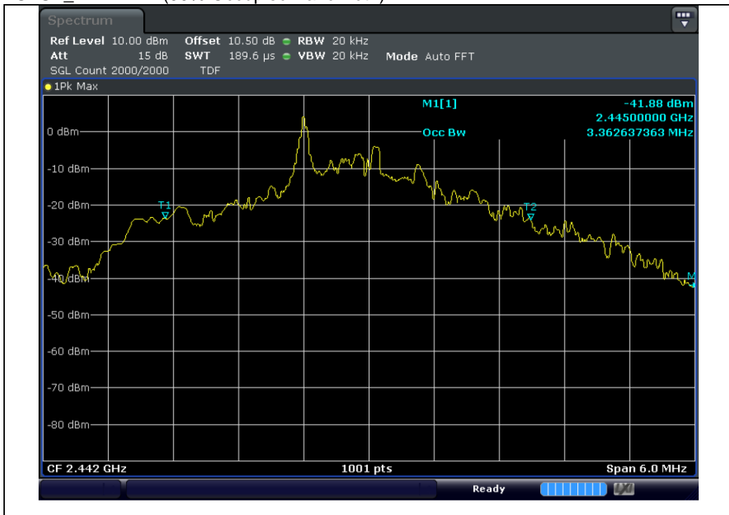
GFSK_2 442 MHz(99% Occupied Bandwidth)
