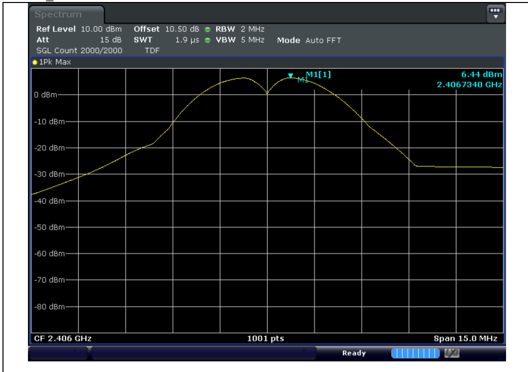
GFSK_2 406 MHz
