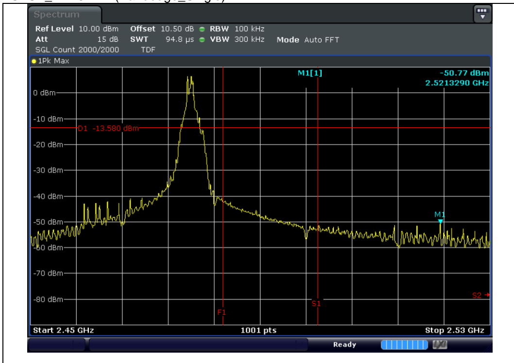
GFSK_2 478 MHz(Bandedge_Single)
