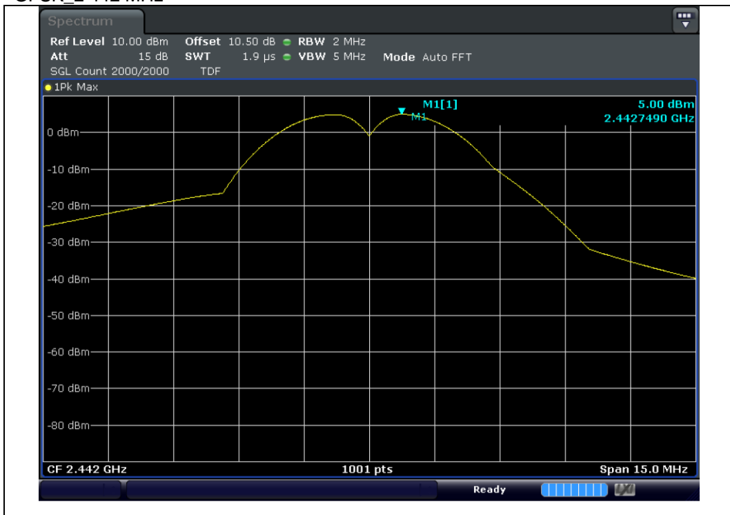
GFSK_2 442 MHz
