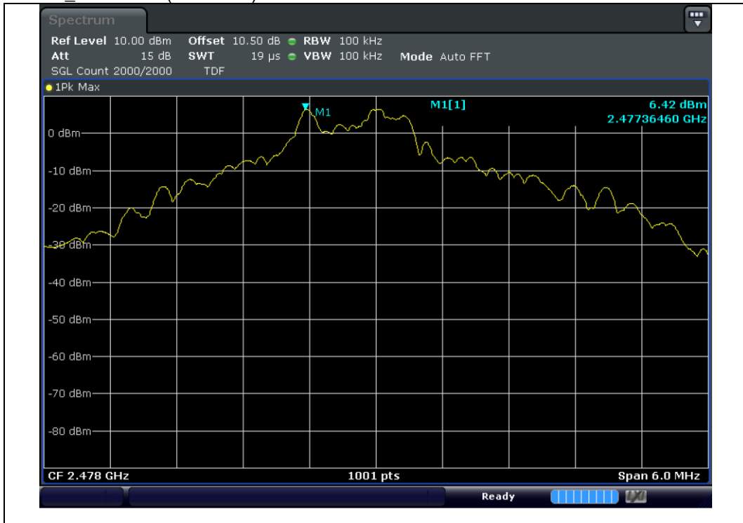
GFSK_2 478 MHz(reference)
