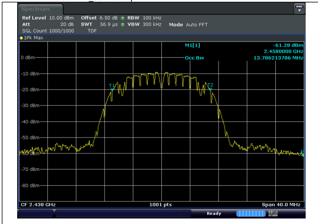
Test mode : 2 438 MHz_99% Occupied Bandwidth
