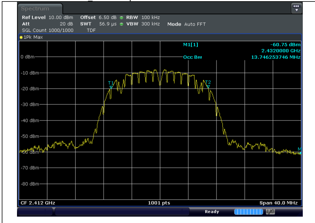
Test mode : 2 412 MHz_99% Occupied Bandwidth
