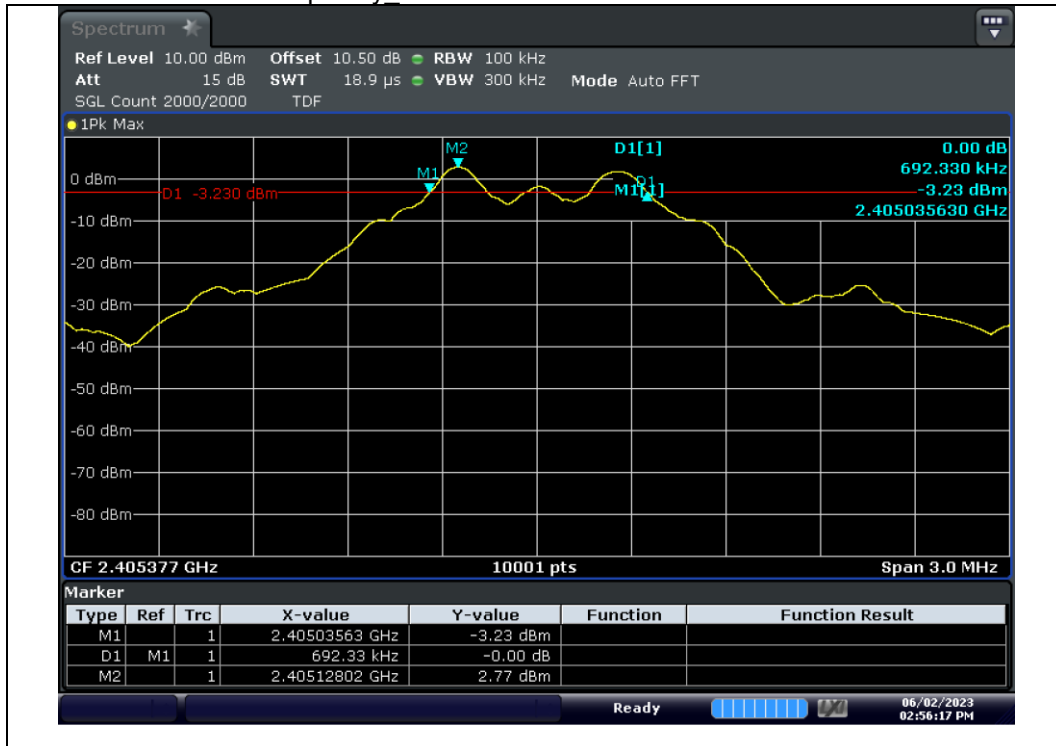
Test mode : Lowest Frequency 6 dB Bandwidth
