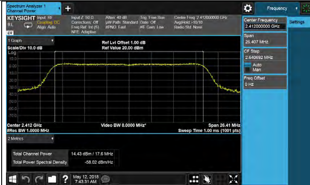
802.11n-HT20 2412MHz Chain 0
