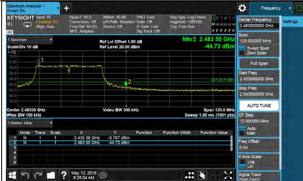
802.11n-HT40-2452MHz Chain 0
