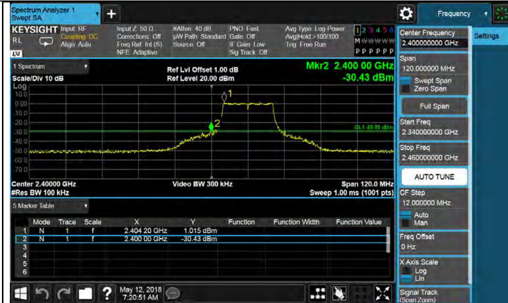
802.11g-2412MHz Chain 0
