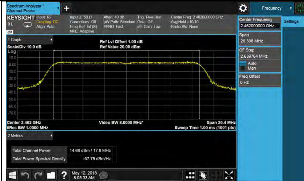
802.11n-HT20 2462MHz Chain 0
