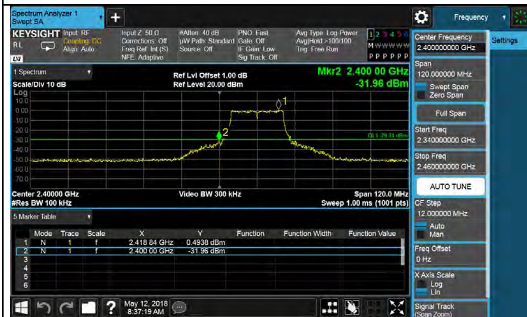
802.11g-2412MHz Chain 1
