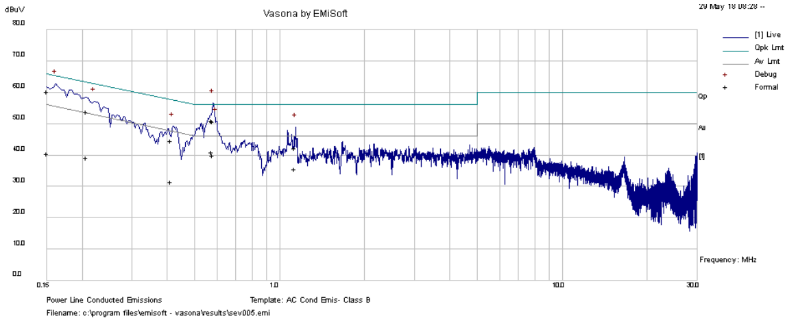
Line Plot at 120Vac, 60Hz
