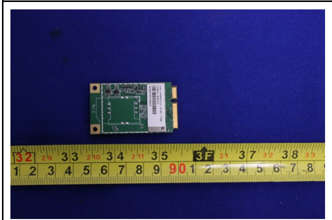
Cellular Board - rear view
