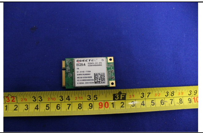
Cellular Board - Front view
