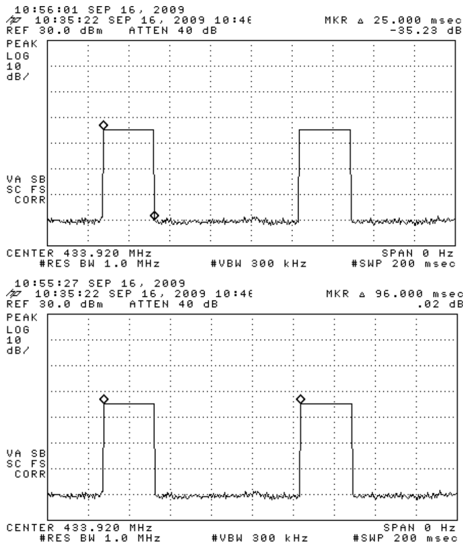
Figure 6.1. Transmission characteristics, (top) single packet length, (bottom) minimum packet period when the DUT is automatically activated for a second transmission
