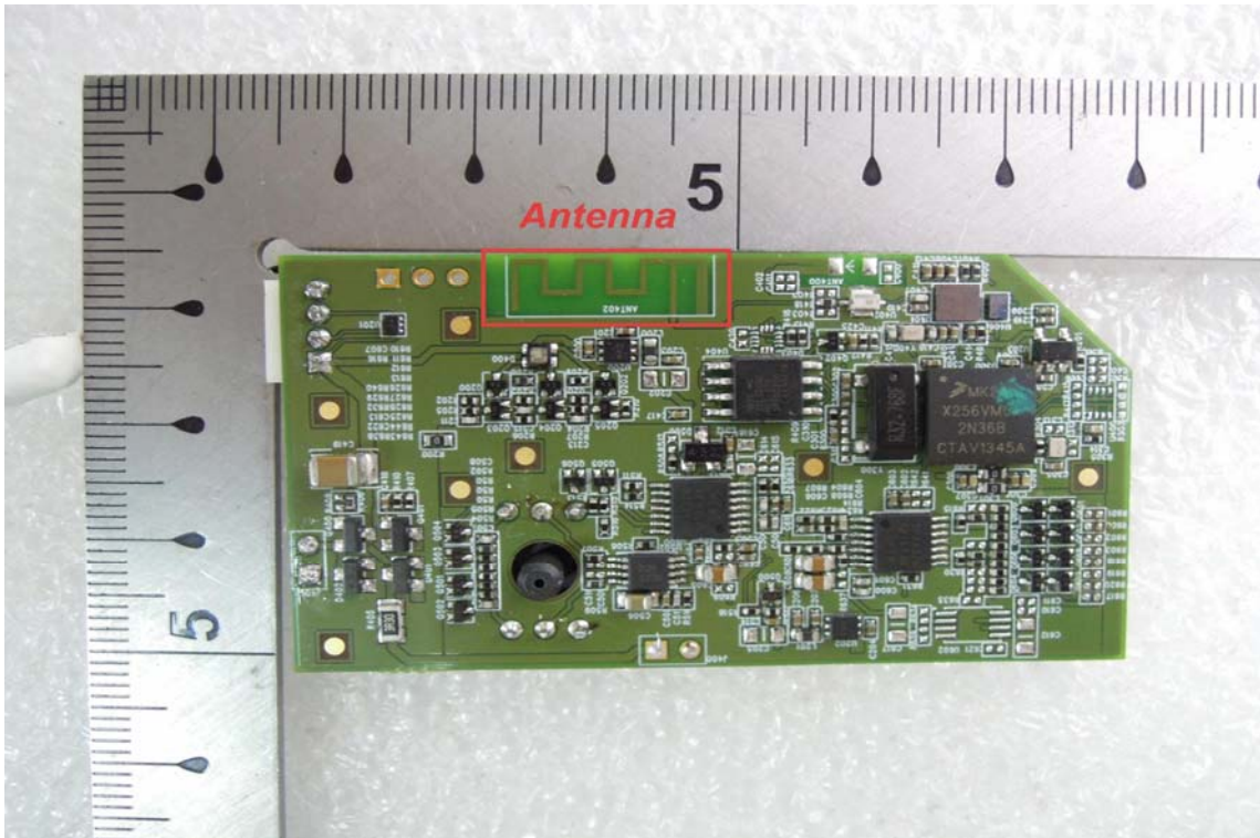
Internal View of EUT – 2 (Antenna)
