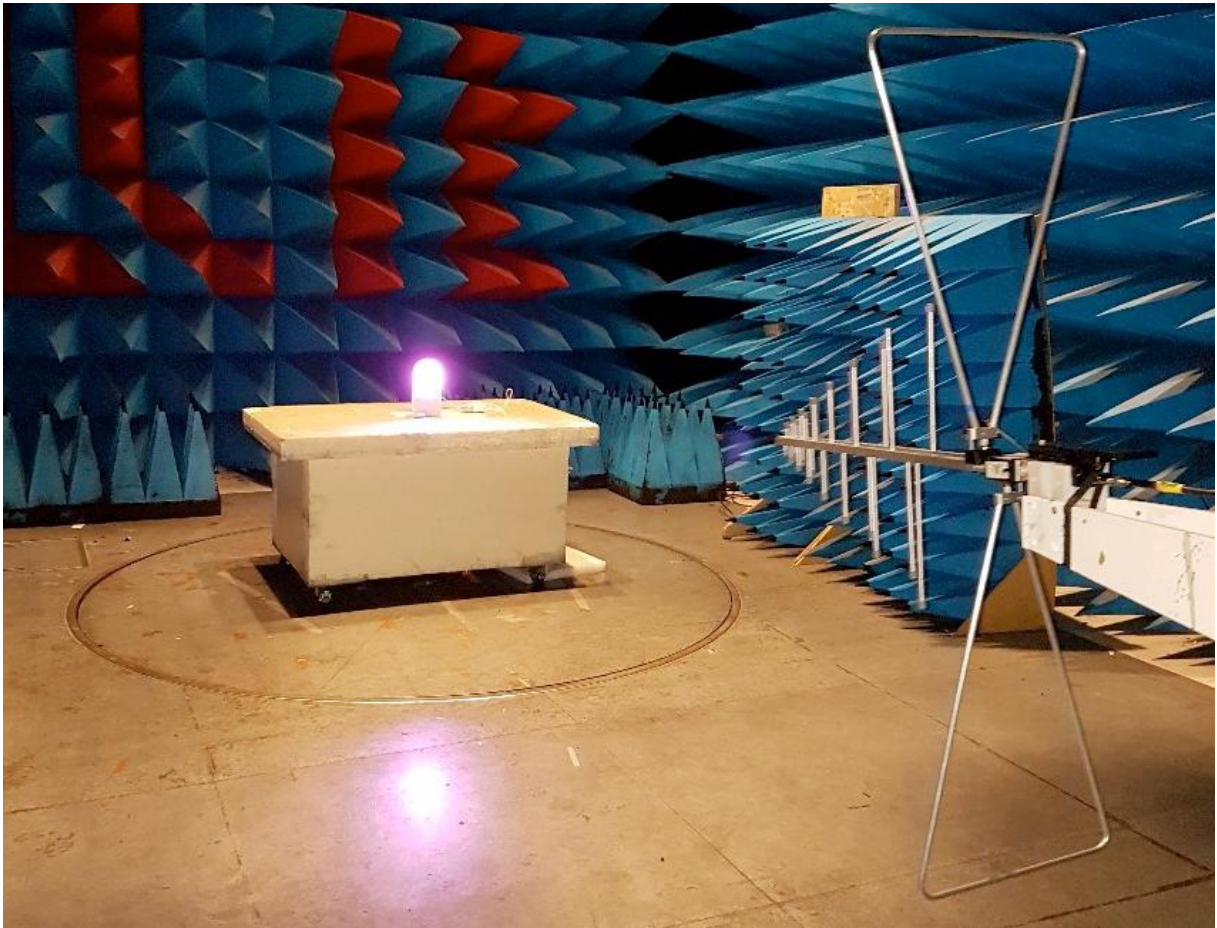
Test setup for radiated emission
