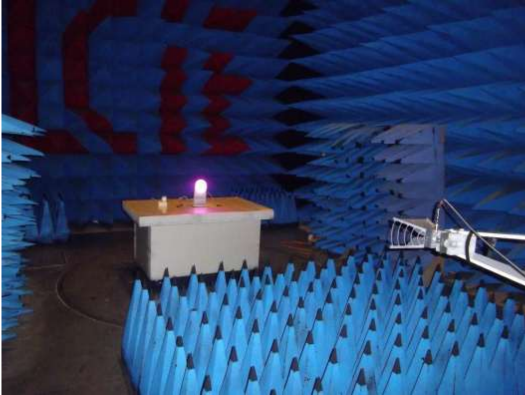
Test setup for radiated field strength
