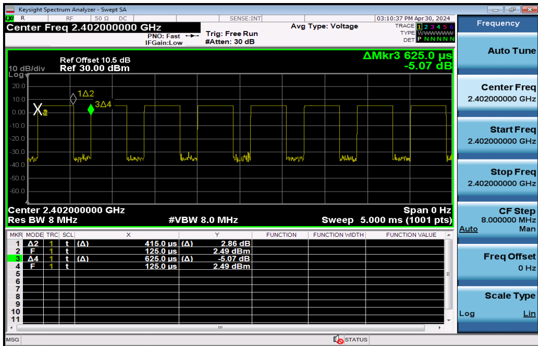
BLE_2M_LowCH00-2402
