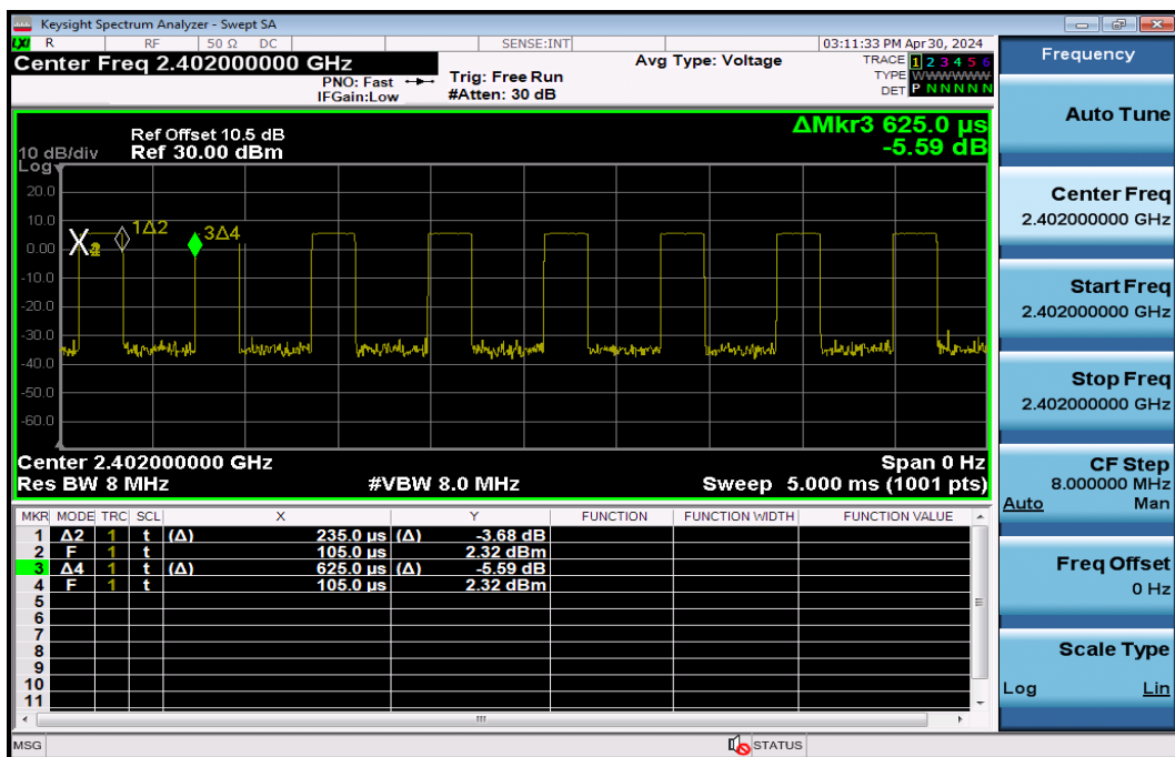
BLE_2M_LowCH00-2402
