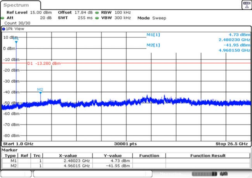
3DH5_Ant1_2480_1000~26500
