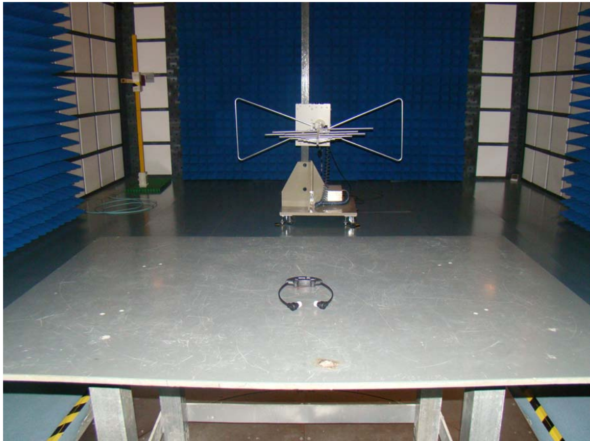
TX Radiated emissions test < 1GHz
