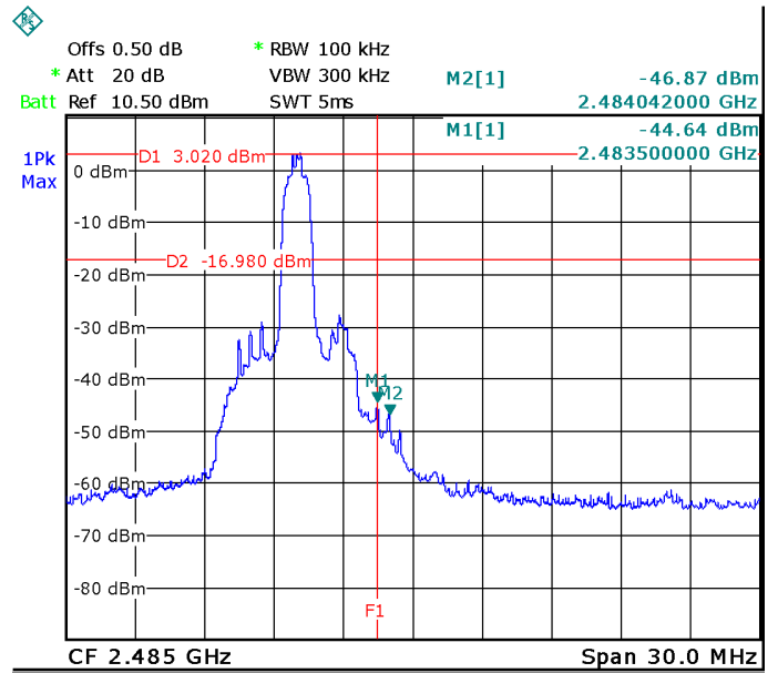
Transmitting Band edge- right side
