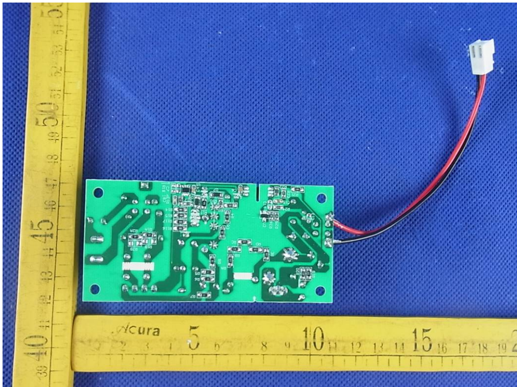
Photo 13 (Power supply board2)
