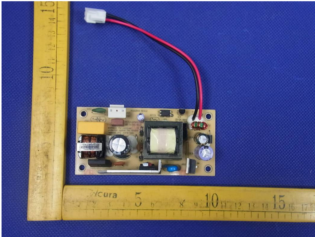
Photo 10 (Power supply board1)
