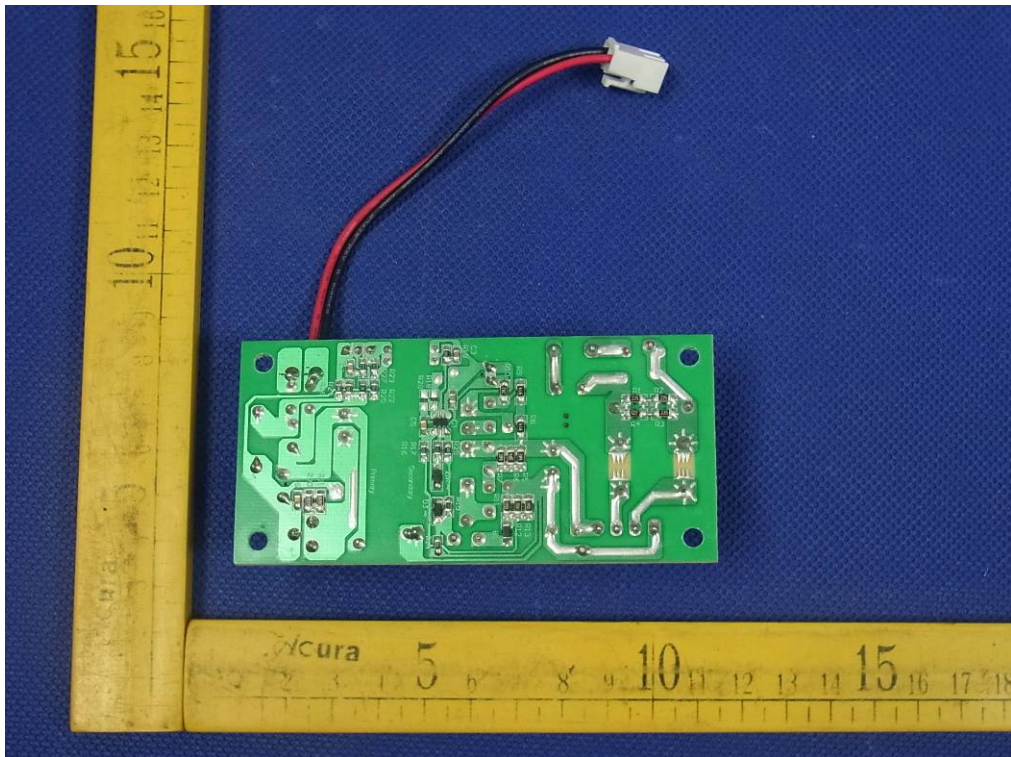
Photo 11 (Power supply board1)
