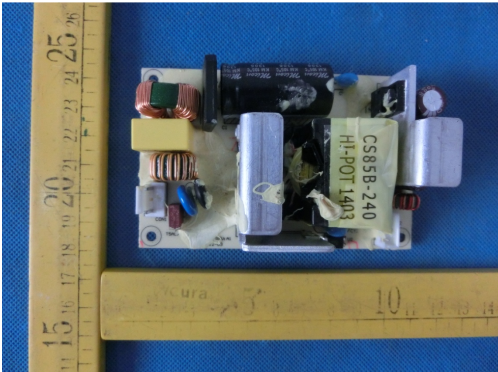
Photo 8 (Power Panel2)
