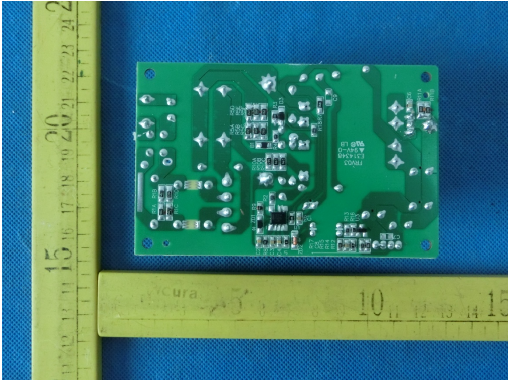
Photo 7 (Power Panel1)
