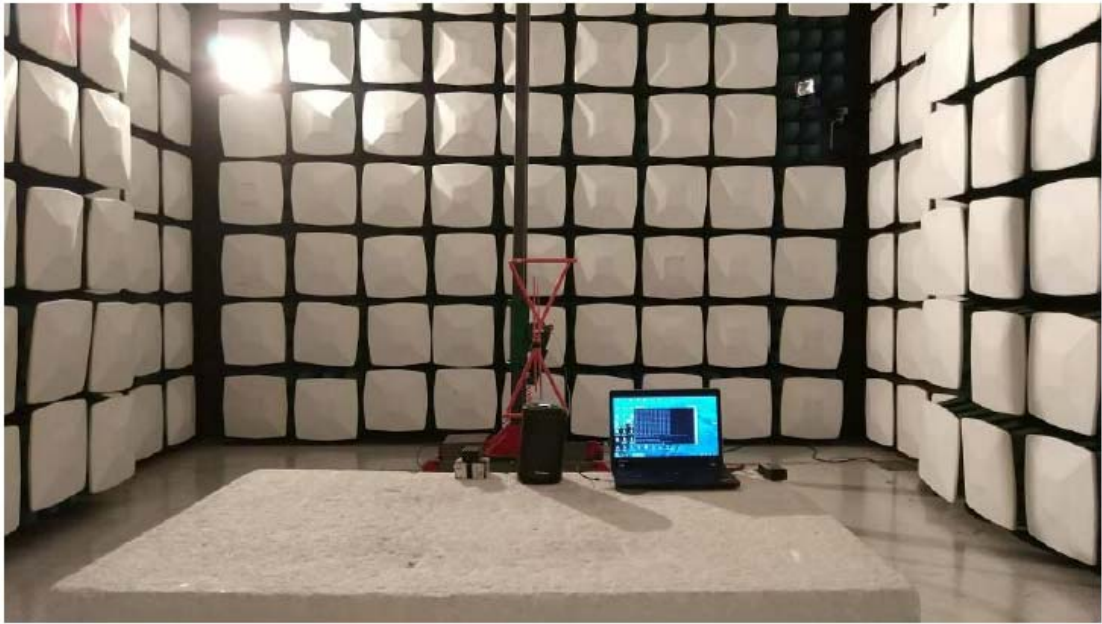
Radiated Test (30-1000 MHz)
