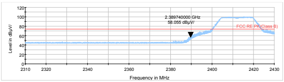
802.11g-Channel 1 Peak
