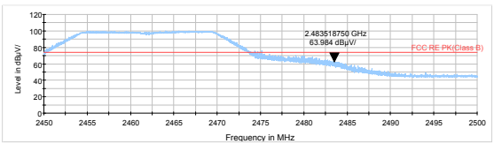
802.11g-Channel 11 Peak
