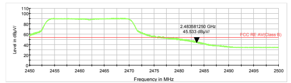
802.11g-Channel 11 Average
