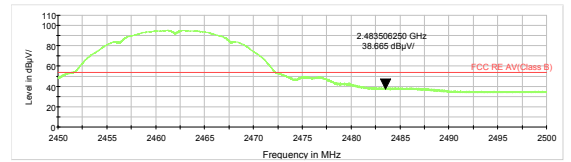
802.11b-Channel 11 Average
