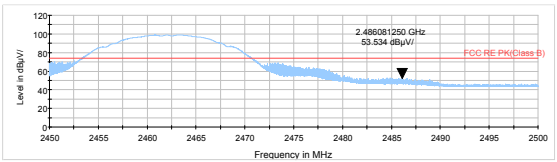
802.11b-Channel 11 Peak
