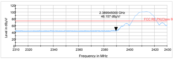
802.11b-Channel 1 Peak
