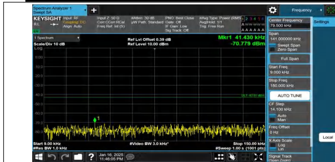
Band66-15MHz-QPSK-132047-1RB#0-0.009~0.15-PASS
