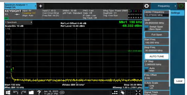
Band66-5MHz-QPSK-132322-1RB#0-0.15~30-PASS
