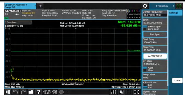
Band66-15MHz-QPSK-132047-1RB#0-0.15~30-PASS
