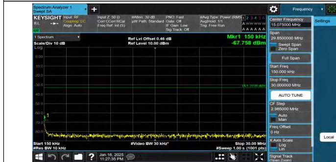
Band66-5MHz-QPSK-131997-1RB#24-0.15~30-PASS
