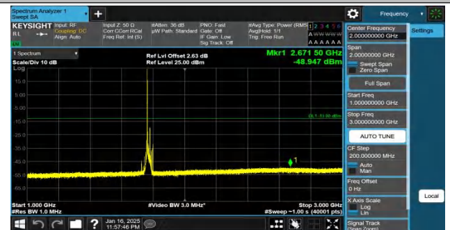
Band66-20MHz-QPSK-132572-1RB#0-1000~3000-PASS
