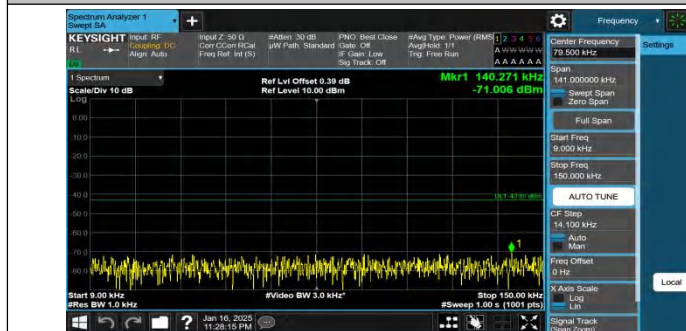
Band66-5MHz-QPSK-132322-1RB#0-0.009~0.15-PASS
