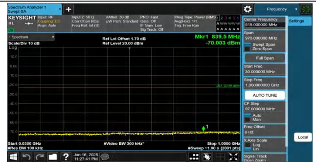
Band66-5MHz-QPSK-131997-1RB#24-30~1000-PASS
