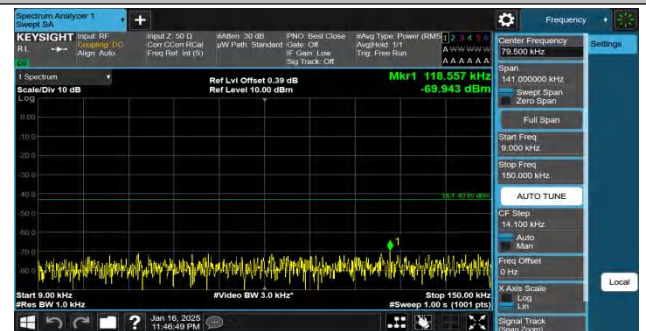
Band66-15MHz-QPSK-132047-1RB#74-0.009~0.15-PASS
