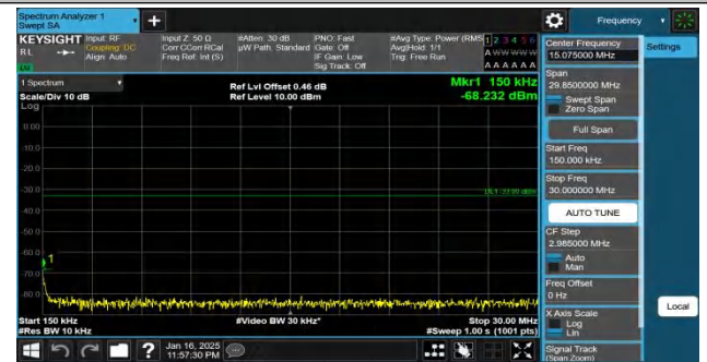
Band66-20MHz-QPSK-132572-1RB#0-0.15~30-PASS
