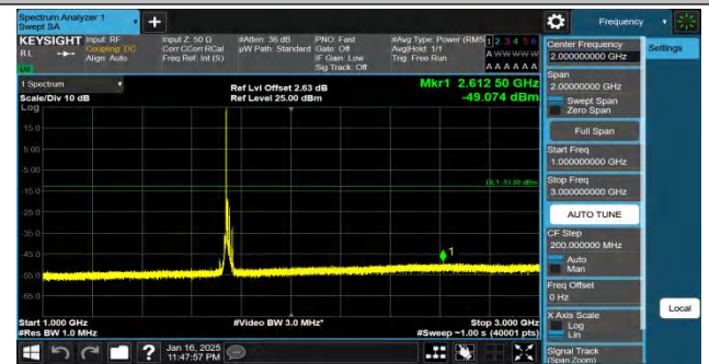
Band66-15MHz-QPSK-132322-1RB#0-1000~3000-PASS
