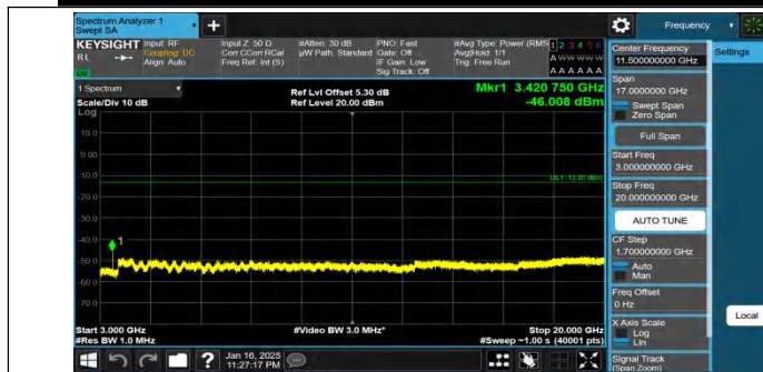
Band66-5MHz-QPSK-131997-1RB#0-3000~20000-PASS
