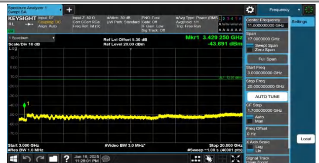
Band66-5MHz-QPSK-131997-1RB#24-3000~20000-PASS
