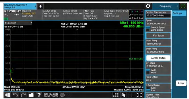
Band7-10MHz-QPSK-21100-1RB#0-0.15~30-PASS
