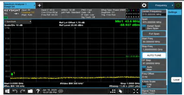
Band7-10MHz-QPSK-21100-1RB#49-30~1000-PASS
