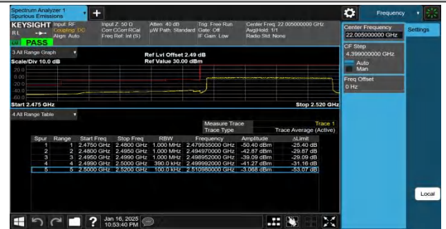
Band7-20MHz-QPSK-20850-100RB#0-PASS
