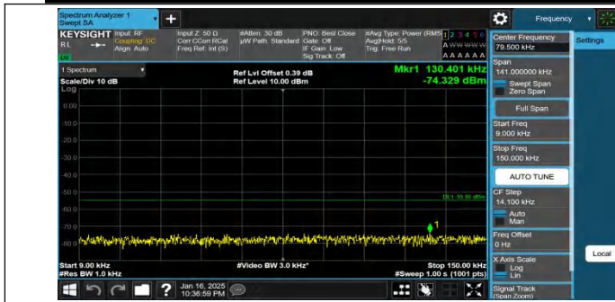
Band7-10MHz-QPSK-21100-1RB#0-0.009~0.15-PASS
