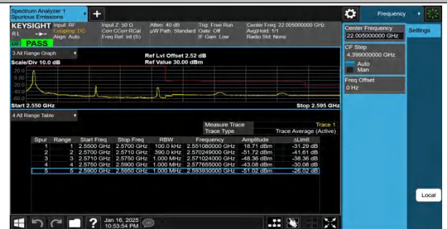
Band7-20MHz-QPSK-21350-1RB#0-PASS
