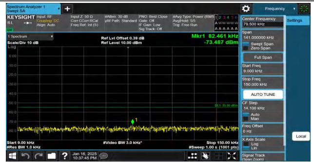
Band7-10MHz-QPSK-21100-1RB#49-0.009~0.15-PASS
