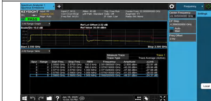
Band7-20MHz-QPSK-21350-100RB#0-PASS
