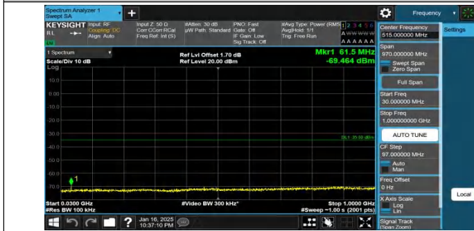
Band7-10MHz-QPSK-21100-1RB#0-30~1000-PASS
