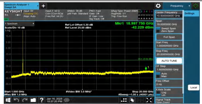
Band7-10MHz-QPSK-21100-1RB#0-1000~20000-PASS
