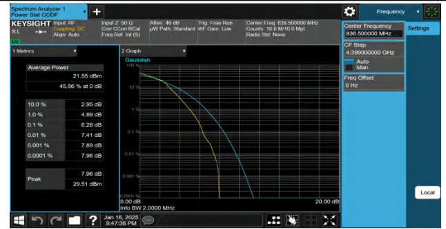
Band5-1.4MHz-16QAM-20525-6RB#0-PASS
