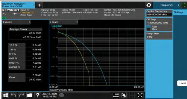
Band5-1.4MHz-QPSK-20525-6RB#0-PASS
