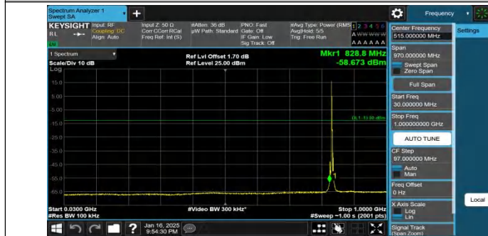
Band5-3MHz-QPSK-20525-1RB#0-30~1000-PASS
