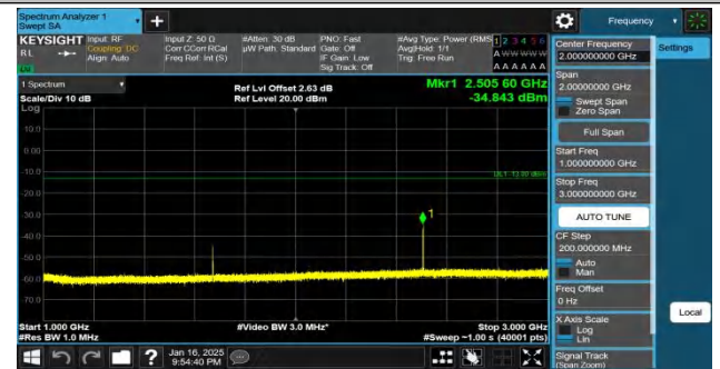
Band5-3MHz-QPSK-20525-1RB#0-1000~3000-PASS
