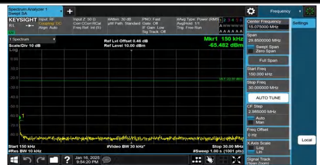
Band5-3MHz-QPSK-20525-1RB#0-0.15~30-PASS
