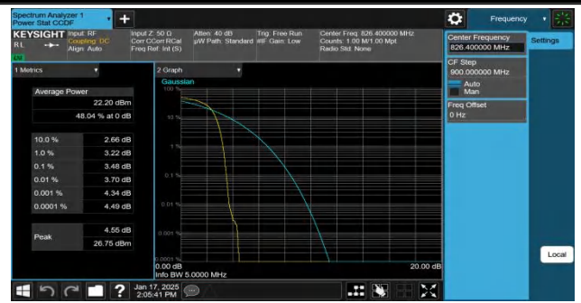
Band5-4132-2-PASS
