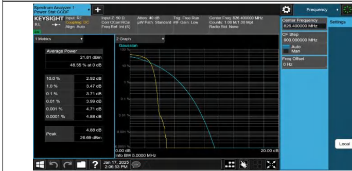
Band5-4132-3-PASS
