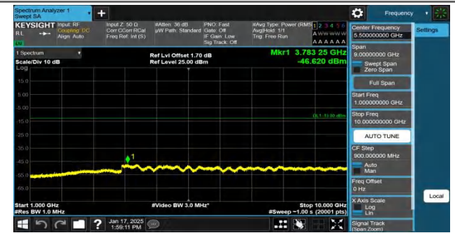
Band5-4233-1000~10000MHz-PASS
