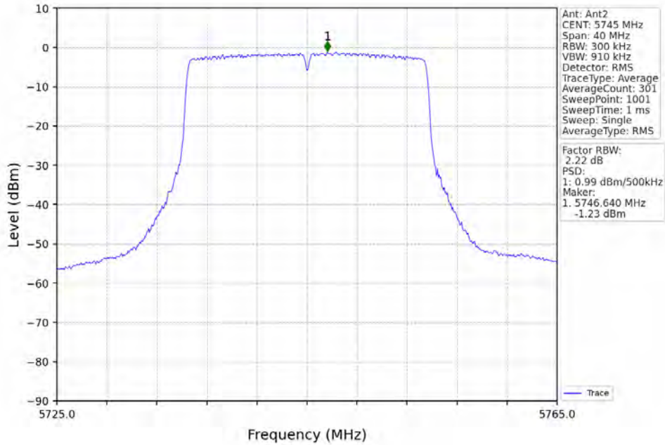
802.11ax(HE20)_LCH_5745MHz_RU242_Left_MIMO_NTNV
