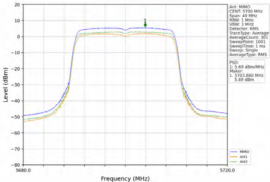
802.11ax(HE20)_HCH_5700MHz_RU242_Left_MIMO_NTNV
