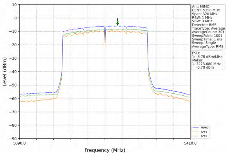
802.11ax(HE160)_MCH_5250MHz_2xRU996_Left_MIMO_NTNV
