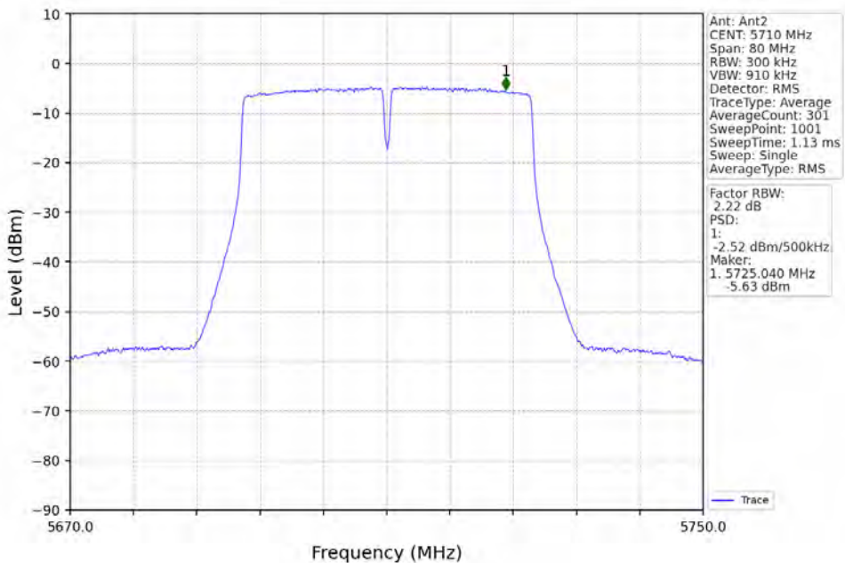
802.11n(HT40)_HCH_5710MHz_Ant2_NTNV
