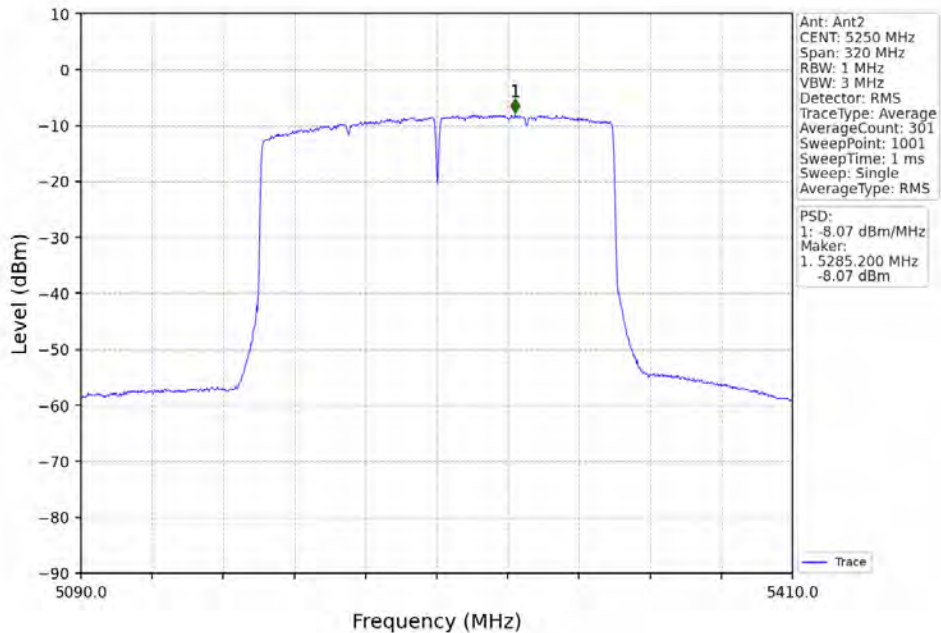
802.11ax(HE160)_MCH_5250MHz_2xRU996_Left_MIMO_NTNV
