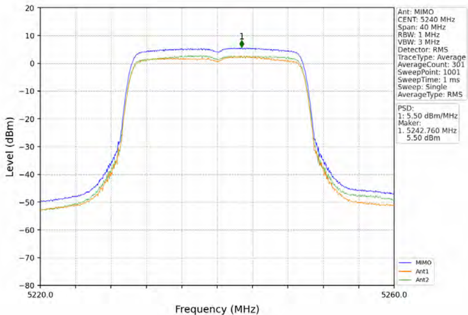
802.11ax(HE20)_HCH_5240MHz_RU242_Left_MIMO_NTNV
