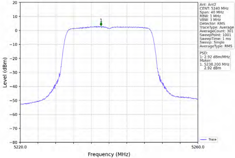
802.11ax(HE20)_HCH_5240MHz_RU242_Left_MIMO_NTNV
