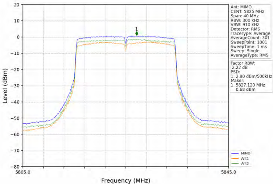
802.11ax(HE20)_HCH_5825MHz_RU242_Left_MIMO_NTNV
