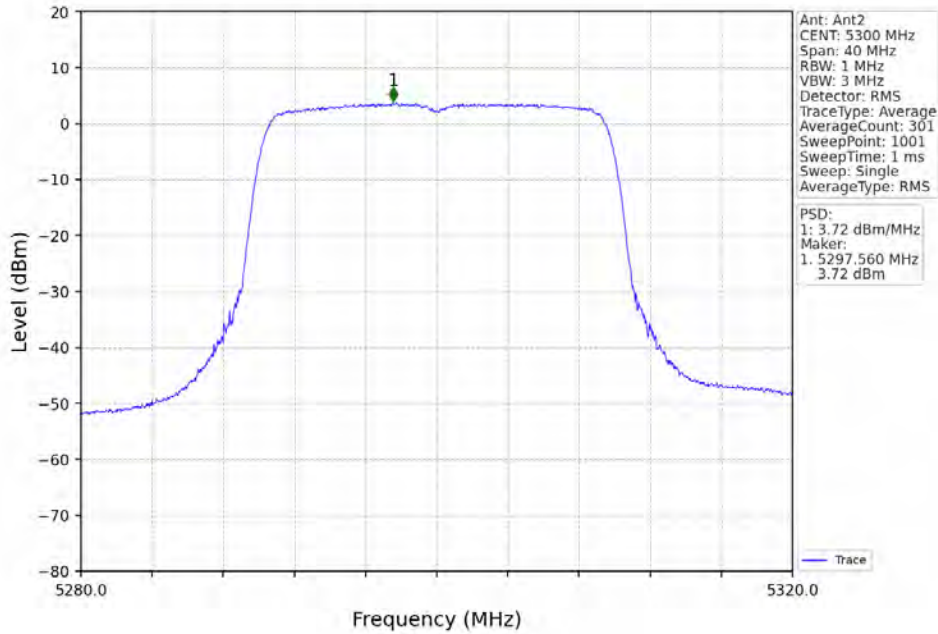
802.11ax(HE20)_MCH_5300MHz_RU242_Left_MIMO_NTNV
