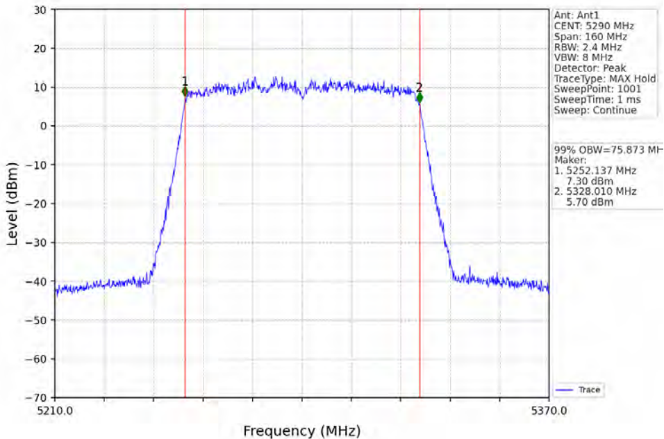
802.11ac(VHT80)_MCH_5290MHz_Ant1_NTNV
