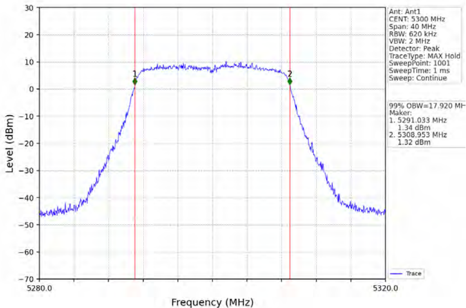
802.11n(HT20)_MCH_5300MHz_Ant1_NTNV
