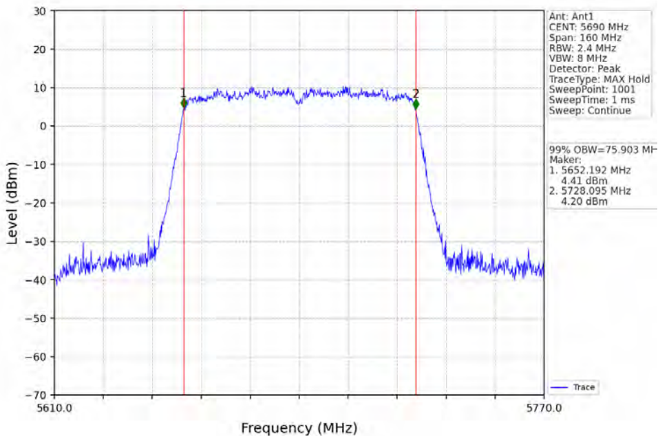
802.11ac(VHT80)_HCH_5690MHz_Ant1_NTNV
