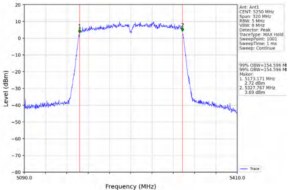
802.11ac(VHT160)_MCH_5250MHz_Ant1_NTNV
