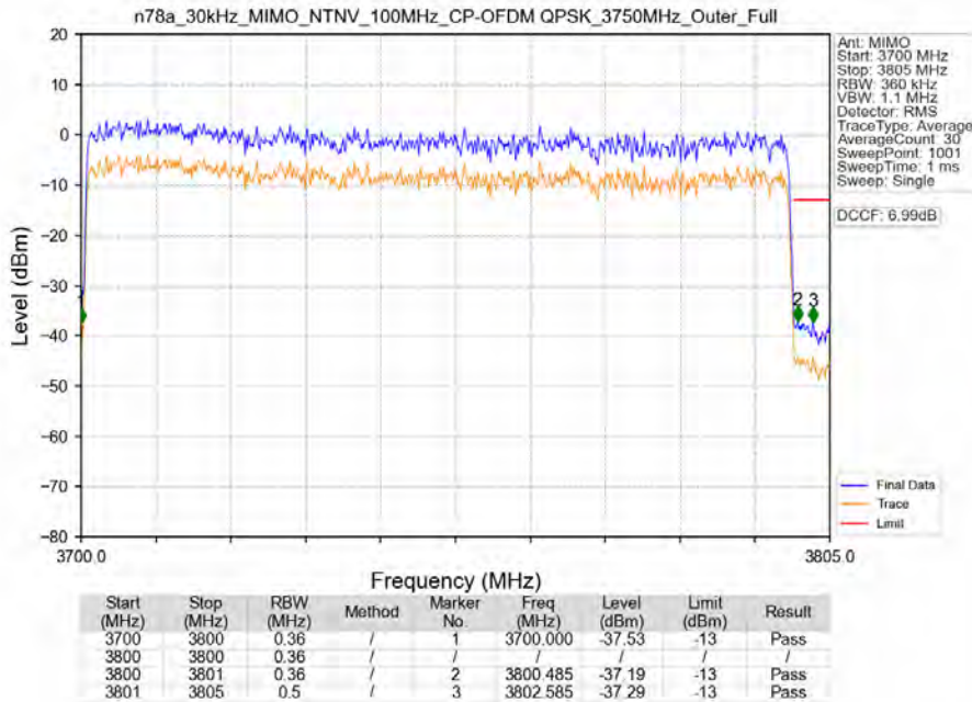
n78a_30kHz_MIMO_NTNV_100MHz_CP-OFDM_QPSK_3750MHz_Outer_Full
