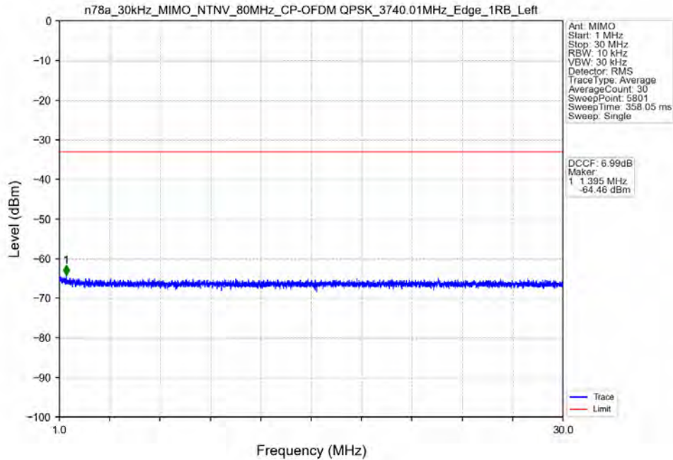
n78a_30kHz_MIMO_NTNV_80MHz_CP-OFDM QPSK_3740.01MHz_Edge_1RB_Left
