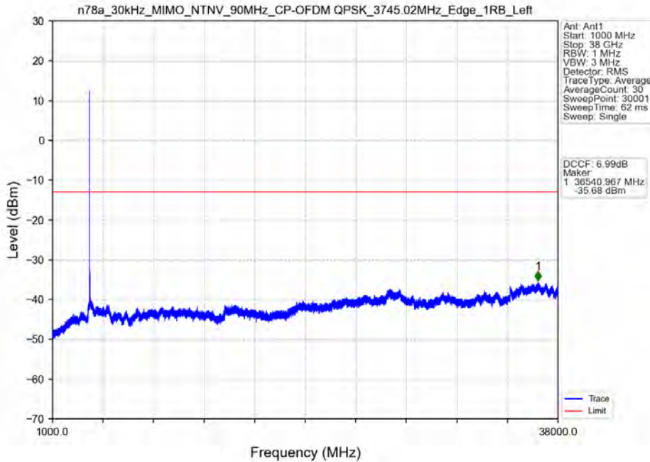
n78a_30kHz_MIMO_NTNV_90MHz_CP-OFDM QPSK_3745.02MHz_Edge_1RB_Left
