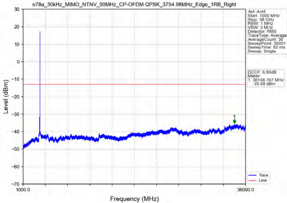
n78a_30kHz_MIMO_NTNV_90MHz_CP-OFDM QPSK_3754.98MHz_Edge_1RB_Right
