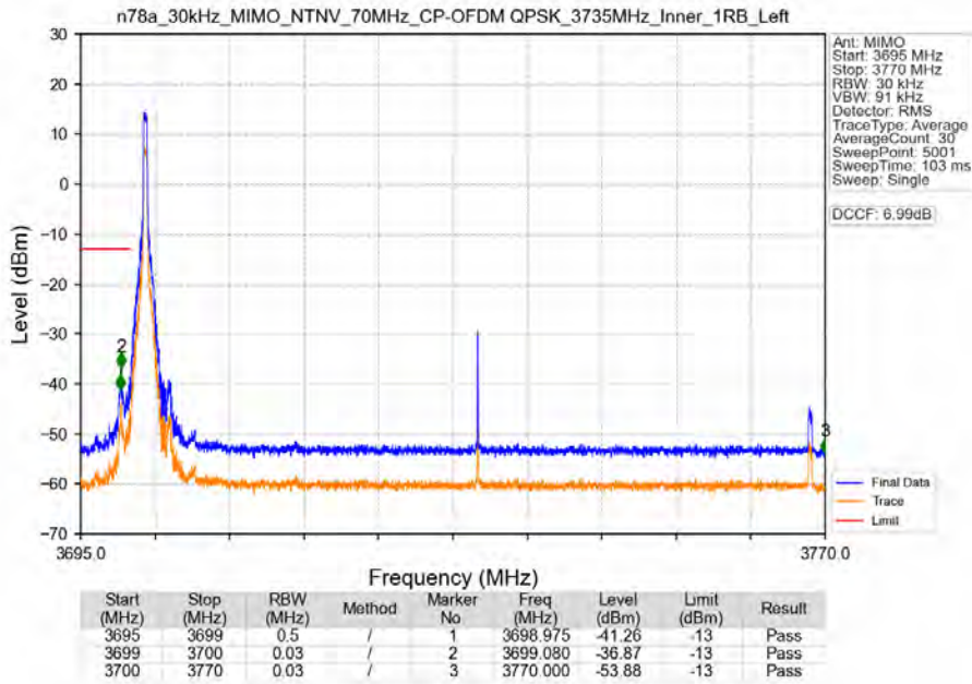
n78a_30kHz_MIMO_NTNV_70MHz_CP-OFDM QPSK_3735MHz_Inner_1RB_Left
