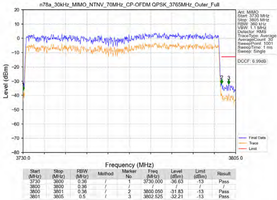
n78a_30kHz_MIMO_NTNV_70MHz_CP-OFDM QPSK_3765MHz_Outer_Full
