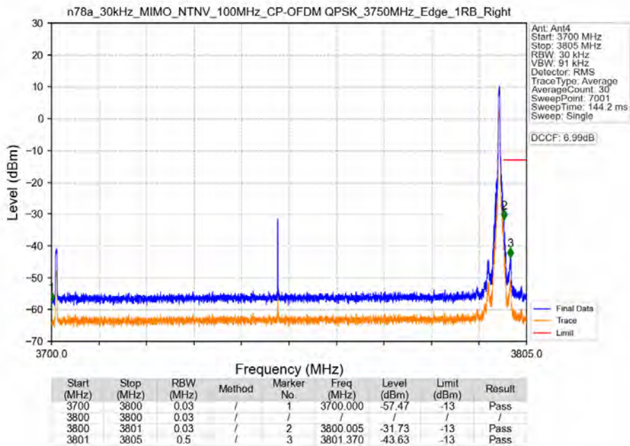
n78a_30kHz_MIMO_NTNV_100MHz_CP-OFDM QPSK_3750MHz_Edge_1RB_Right
