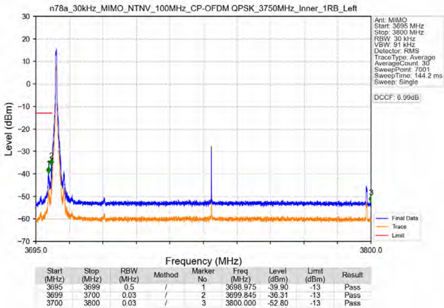
n78a_30kHz_MIMO_NTNV_100MHz_CP-OFDM QPSK_3750MHz_Inner_1RB_Left
