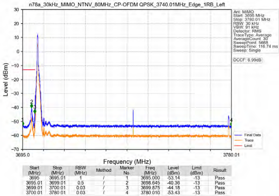
n78a_30kHz_MIMO_NTNV_80MHz_CP-OFDM QPSK_3740.01MHz_Edge_1RB_Left
