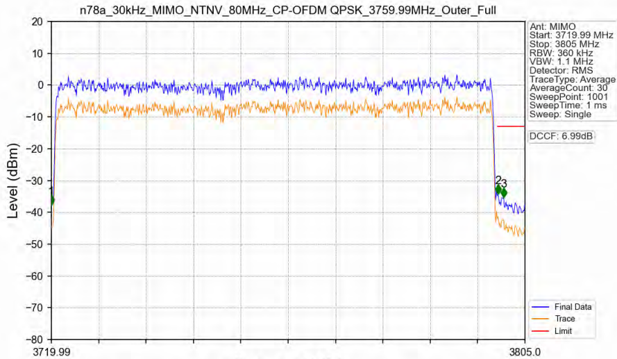
n78a_30kHz_MIMO_NTNV_80MHz_CP-OFDM QPSK_3759.99MHz_Outer_Full
