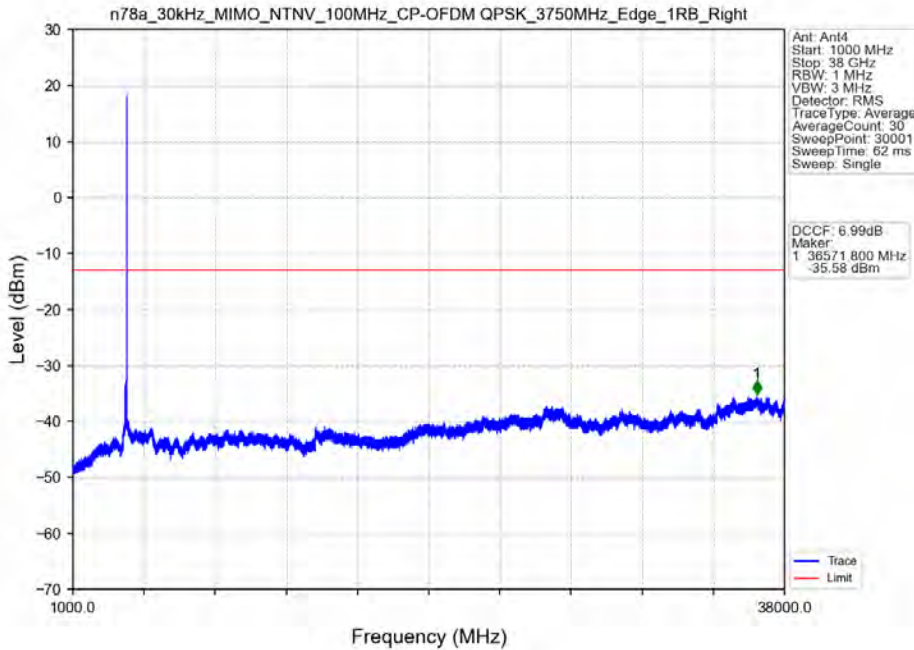
n78a_30kHz_MIMO_NTNV_100MHz_CP-OFDM QPSK_3750MHz_Edge_1RB_Right
