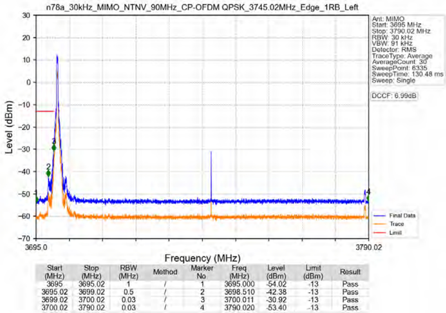
n78a_30kHz_MIMO_NTNV_90MHz_CP-OFDM QPSK_3745.02MHz_Edge_1RB_Left
