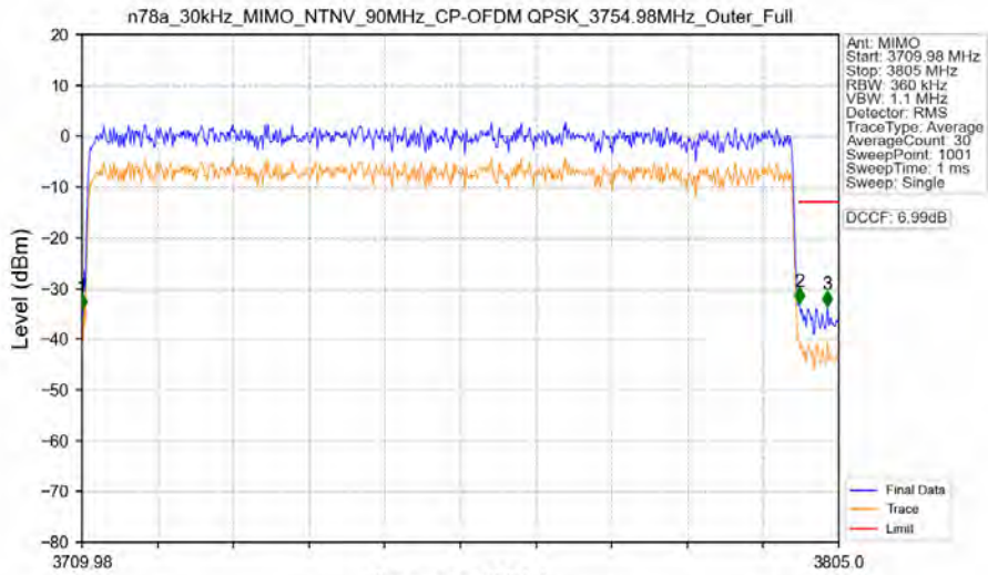
n78a_30kHz_MIMO_NTNV_90MHz_CP-OFDM QPSK_3754.98MHz_Outer_Full
