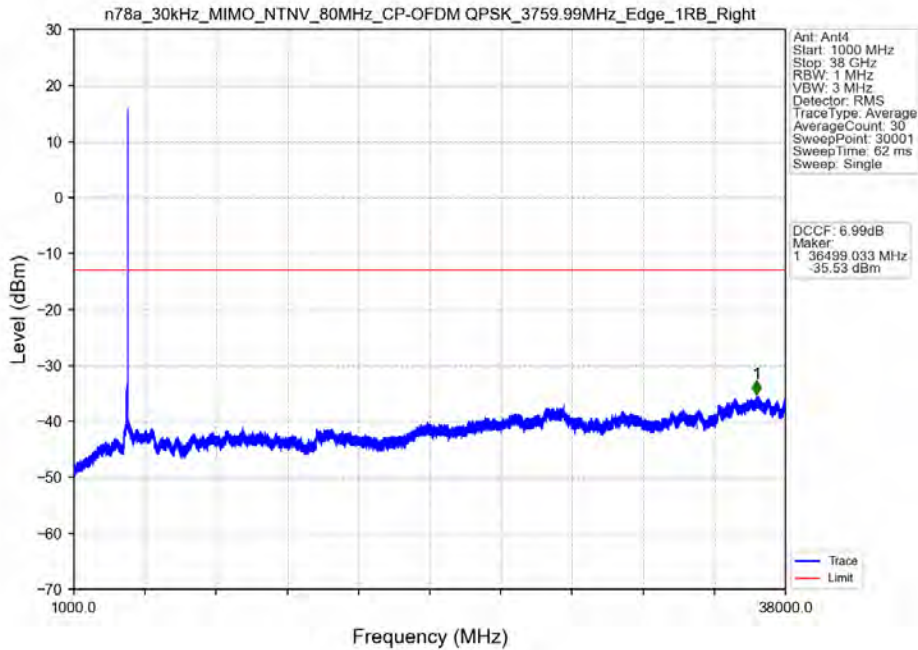
n78a_30kHz_MIMO_NTNV_80MHz_CP-OFDM QPSK_3759.99MHz_Edge_1RB_Right
