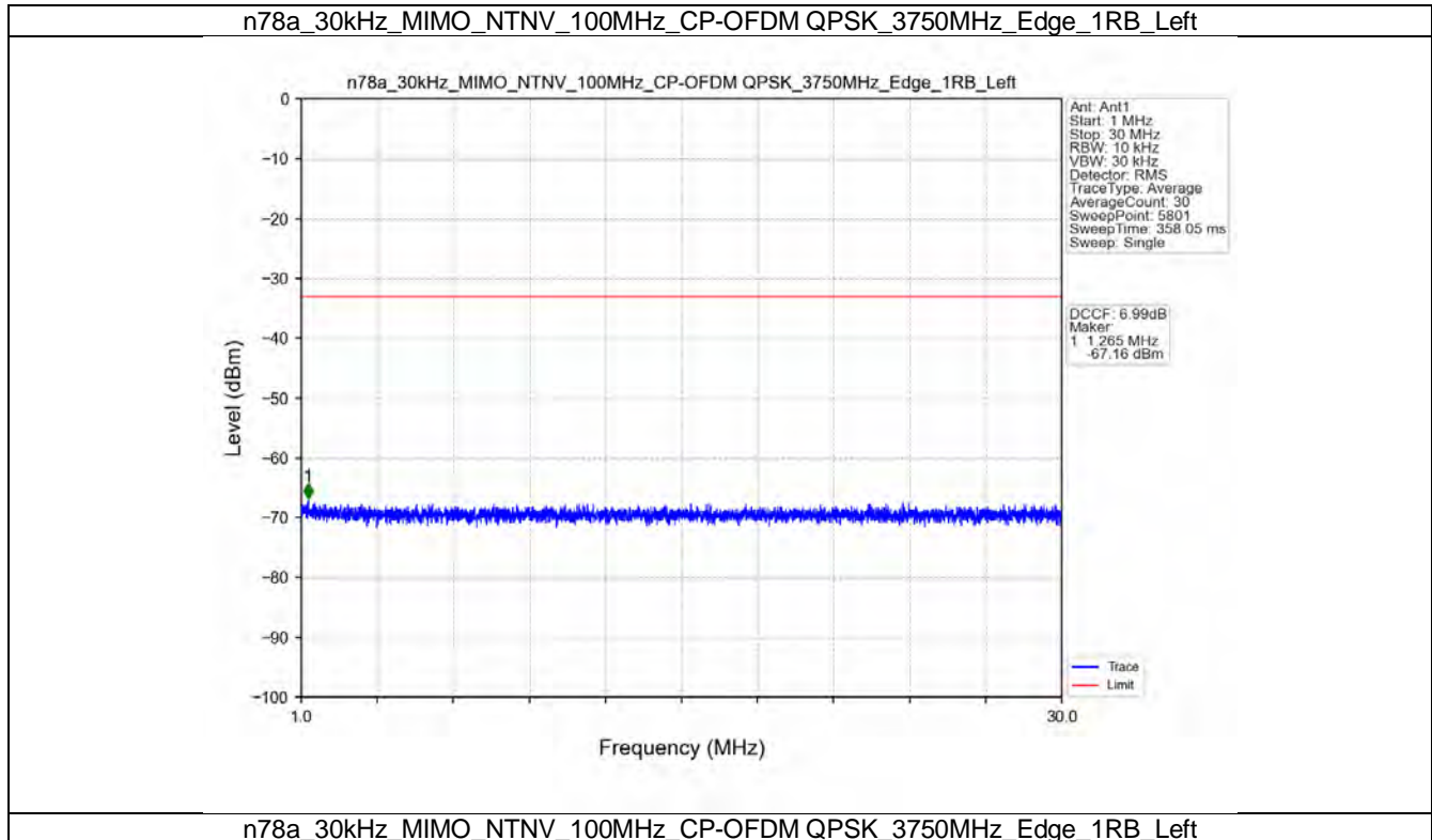
n78a_30kHz_MIMO_NTNV_100MHz_CP-OFDM QPSK_3750MHz_Edge_1RB_Left
