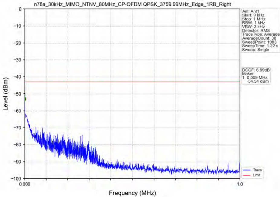
n78a_30kHz_MIMO_NTNV_80MHz_CP-OFDM QPSK_3759.99MHz_Edge_1RB_Right
