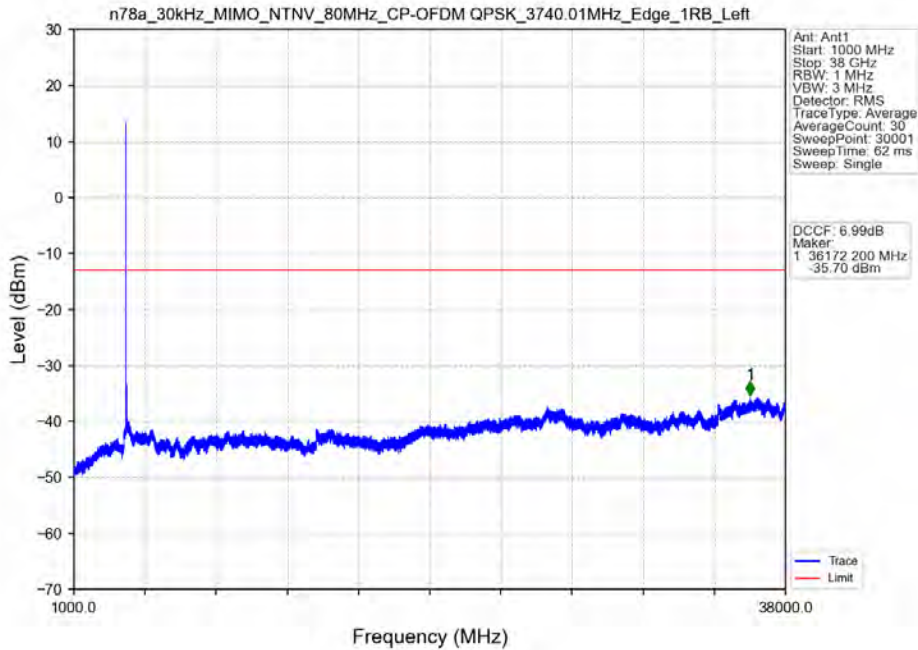
n78a_30kHz_MIMO_NTNV_80MHz_CP-OFDM QPSK_3740.01MHz_Edge_1RB_Left
