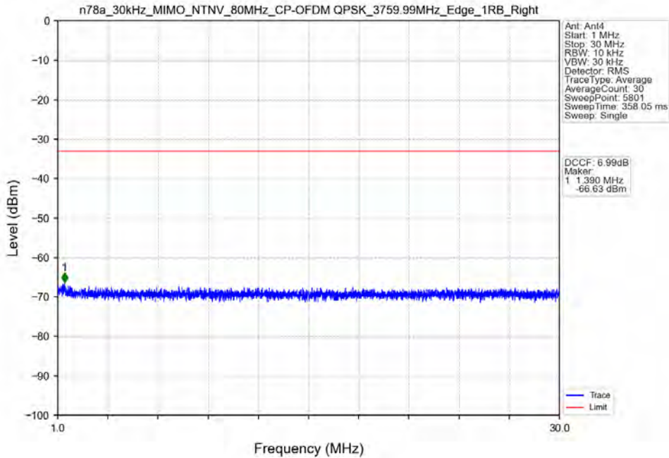
n78a_30kHz_MIMO_NTNV_80MHz_CP-OFDM QPSK_3759.99MHz_Edge_1RB_Right
