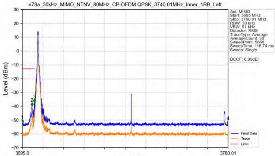
n78a_30kHz_MIMO_NTNV_80MHz_CP-OFDM QPSK_3740.01MHz_Inner_1RB_Left
