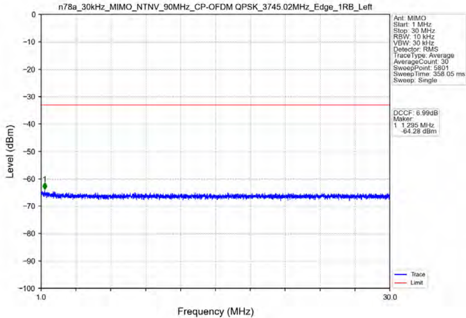
n78a_30kHz_MIMO_NTNV_90MHz_CP-OFDM QPSK_3745.02MHz_Edge_1RB_Left
