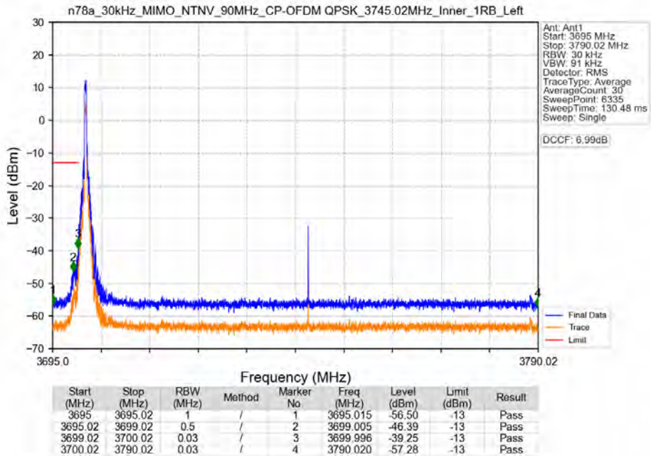
n78a_30kHz_MIMO_NTNV_90MHz_CP-OFDM QPSK_3745.02MHz_Inner_1RB_Left
