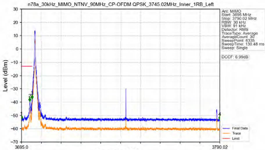
n78a_30kHz_MIMO_NTNV_90MHz_CP-OFDM QPSK_3745.02MHz_Inner_1RB_Left
