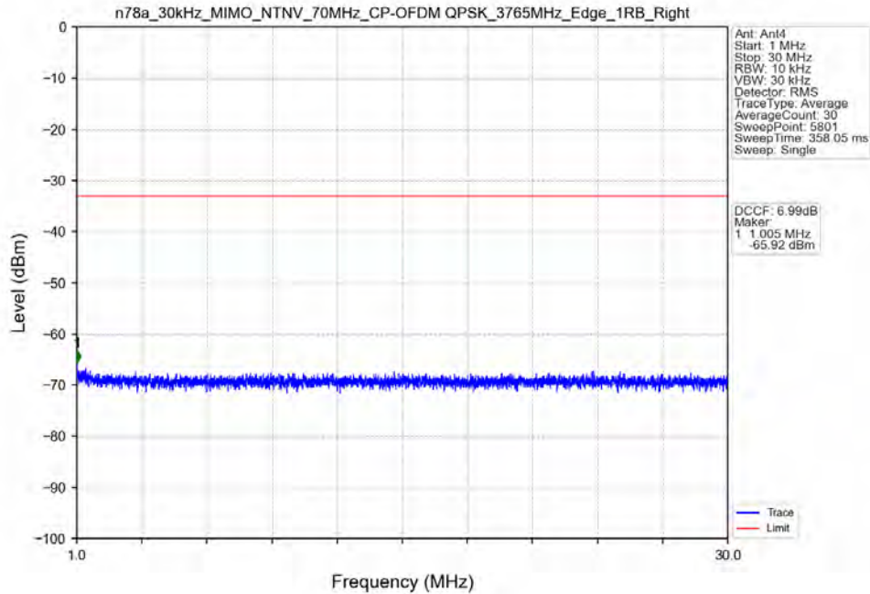
n78a_30kHz_MIMO_NTNV_70MHz_CP-OFDM QPSK_3765MHz_Edge_1RB_Right
