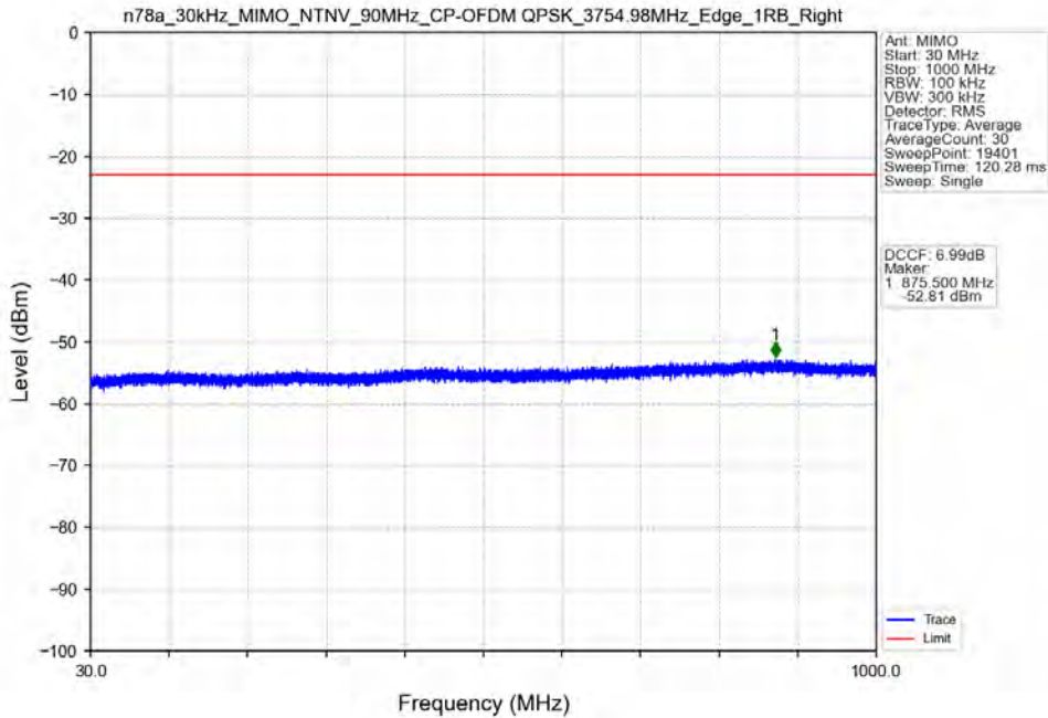
n78a_30kHz_MIMO_NTNV_90MHz_CP-OFDM QPSK_3754.98MHz_Edge_1RB_Right
