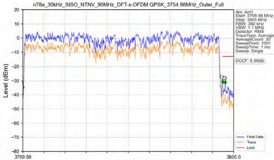
n78a_30kHz_SISO_NTNV_90MHz_DFT-s-OFDM QPSK_3754.98MHz_Outer_Full
