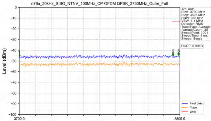
n78a_30kHz_SISO_NTNV_100MHz_CP-OFDM QPSK_3750MHz_Outer_Full
