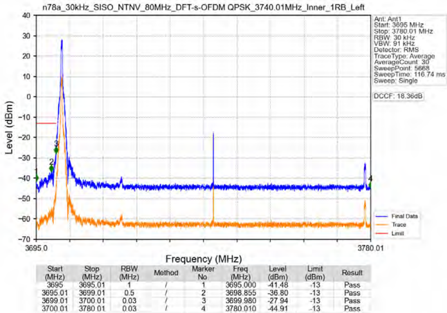
n78a_30kHz_SISO_NTNV_80MHz_DFT-s-OFDM_QPSK_3740.01MHz_Inner_1RB_Left
