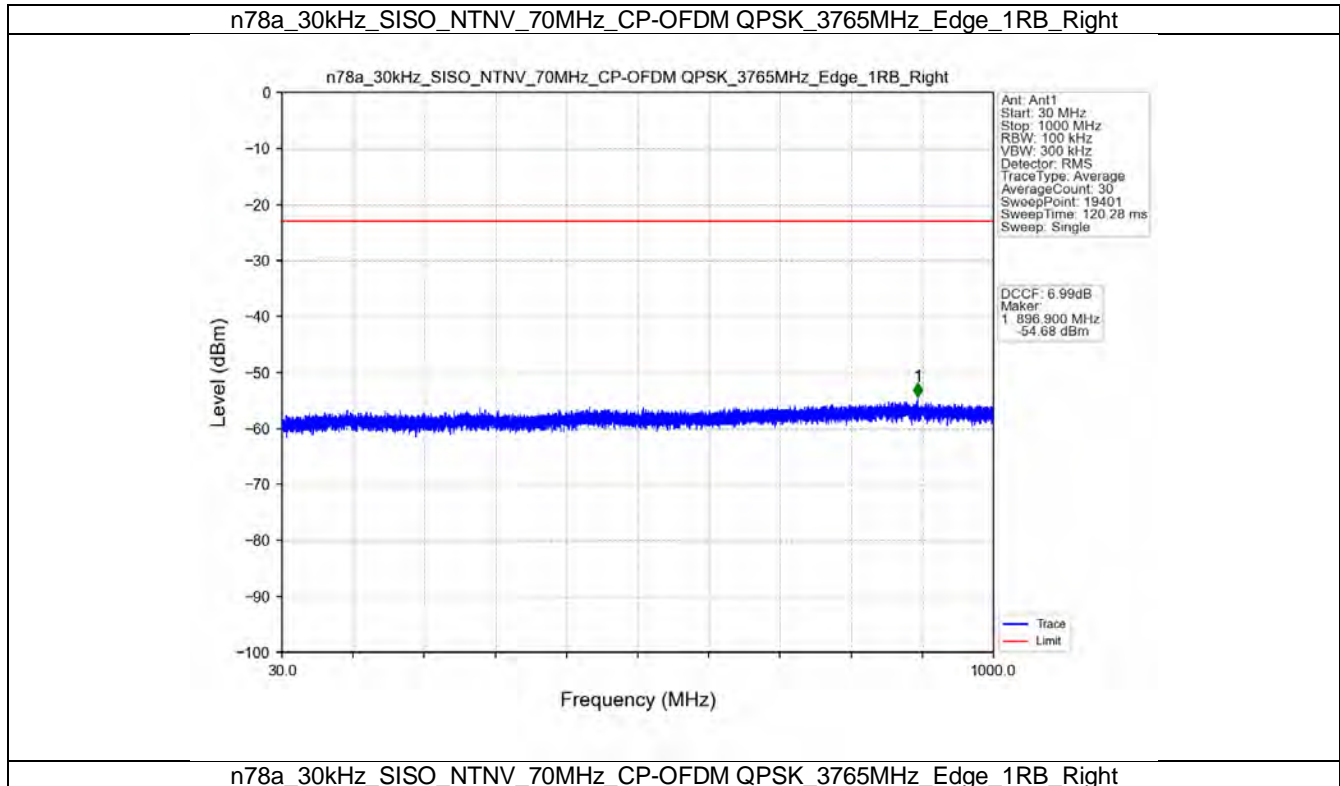
n78a_30kHz_SISO_NTNV_70MHz_CP-OFDM_QPSK_3765MHz_Edge_1RB_Right
