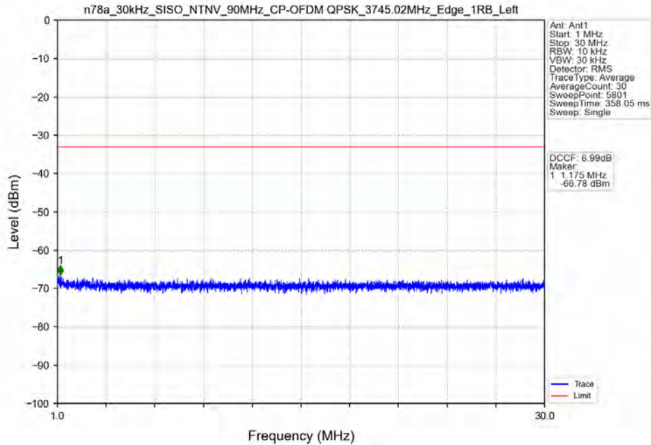
n78a_30kHz_SISO_NTNV_90MHz_CP-OFDM QPSK_3745.02MHz_Edge_1RB_Left
