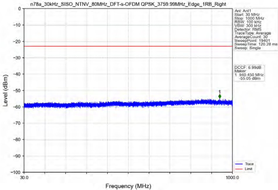
n78a_30kHz_SISO_NTNV_80MHz_DFT-s-OFDM QPSK_3759.99MHz_Edge_1RB_Right
