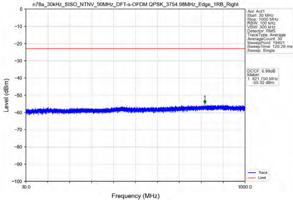
n78a_30kHz_SISO_NTNV_90MHz_DFT-s-OFDM QPSK_3754.98MHz_Edge_1RB_Right
