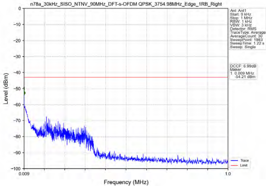
n78a_30kHz_SISO_NTNV_90MHz_DFT-s-OFDM QPSK_3754.98MHz_Edge_1RB_Right
