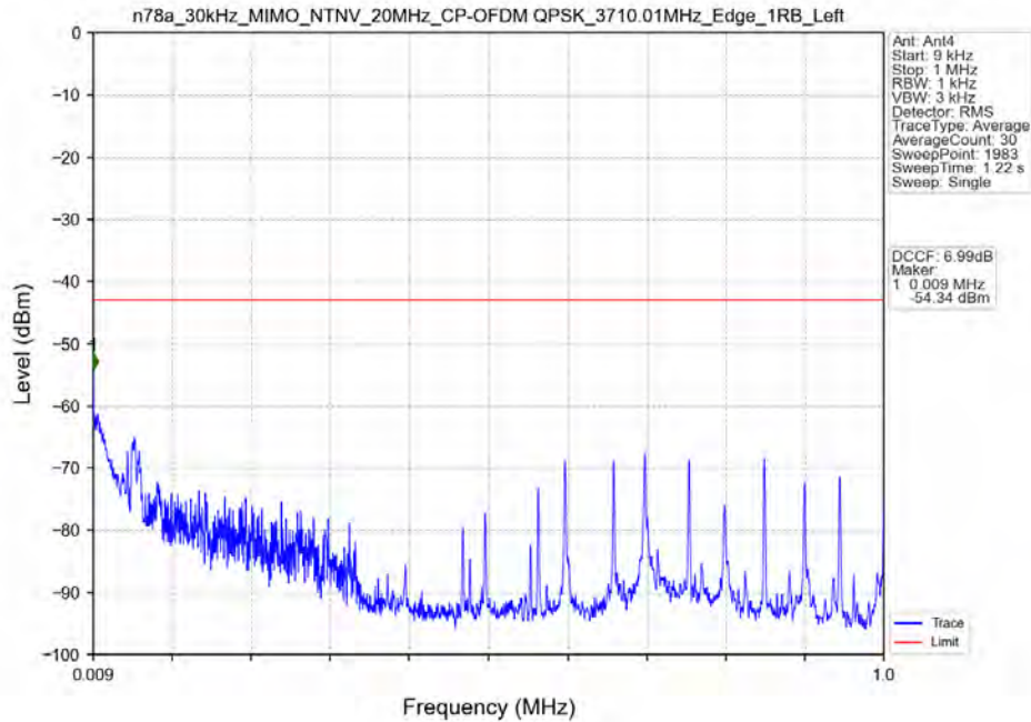
n78a_30kHz_MIMO_NTNV_20MHz_CP-OFDM QPSK_3710.01MHz_Edge_1RB_Left
