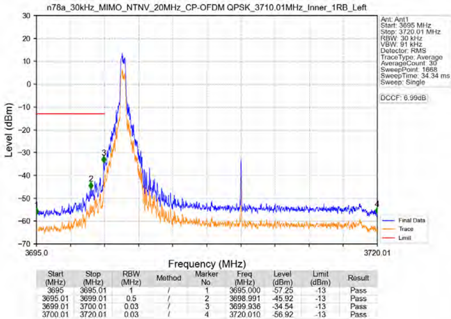
n78a_30kHz_MIMO_NTNV_20MHz_CP-OFDM QPSK_3710.01MHz_Inner_1RB_Left
