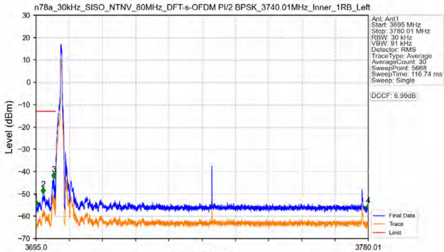
n78a_30kHz_SISO_NTNV_80MHz_DFT-s-OFDM PI/2 BPSK_3740.01MHz_Inner_1RB_Left
