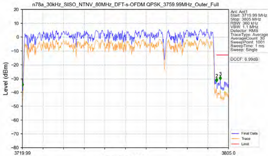
n78a_30kHz_SISO_NTNV_80MHz_DFT-s-OFDM QPSK_3759.99MHz_Outer_Full
