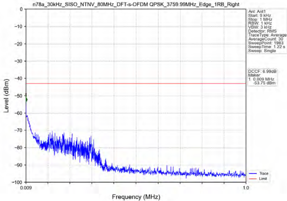
n78a_30kHz_SISO_NTNV_80MHz_DFT-s-OFDM QPSK_3759.99MHz_Edge_1RB_Right
