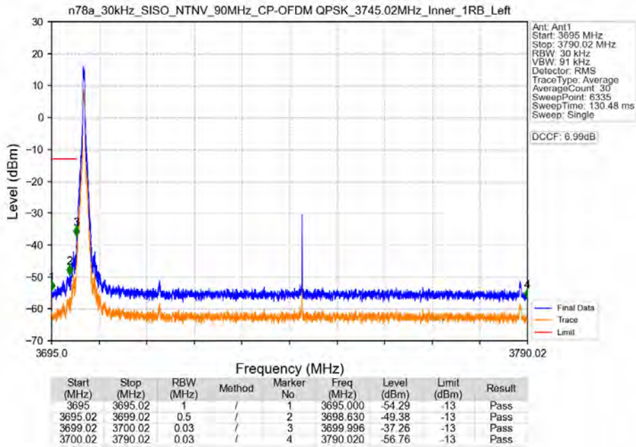
n78a_30kHz_SISO_NTNV_90MHz_CP-OFDM QPSK_3745.02MHz_Inner_1RB_Left
