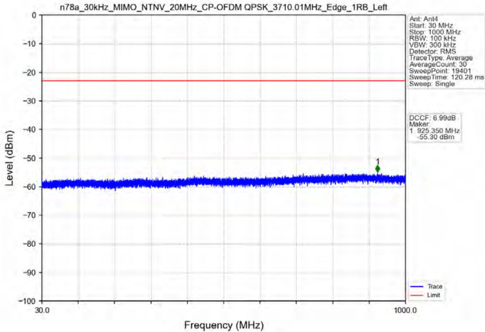
n78a_30kHz_MIMO_NTNV_20MHz_CP-OFDM QPSK_3710.01MHz_Edge_1RB_Left
