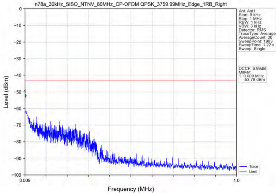
n78a_30kHz_SISO_NTNV_80MHz_CP-OFDM QPSK_3759.99MHz_Edge_1RB_Right
