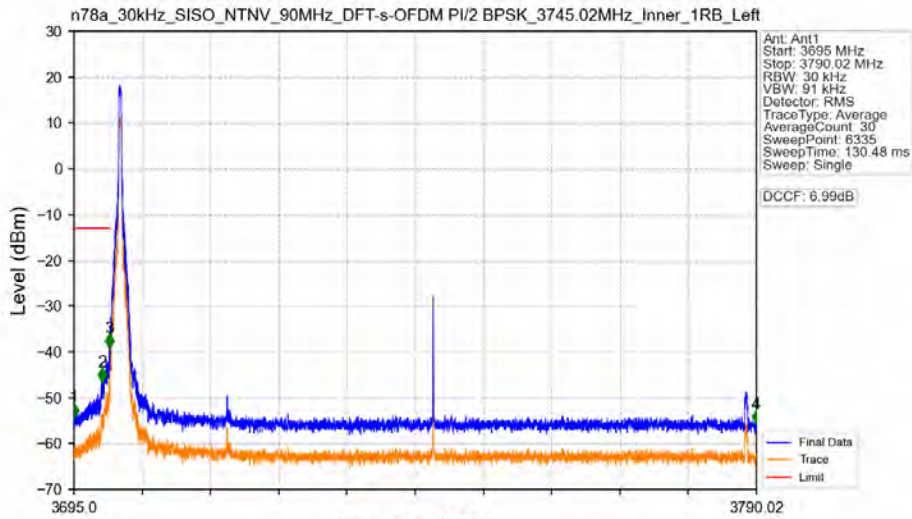
n78a_30kHz_SISO_NTNV_90MHz_DFT-s-OFDM PI/2 BPSK_3745.02MHz_Inner_1RB_Left
