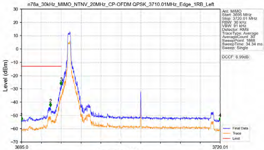
n78a_30kHz_MIMO_NTNV_20MHz_CP-OFDM QPSK_3710.01MHz_Edge_1RB_Left
