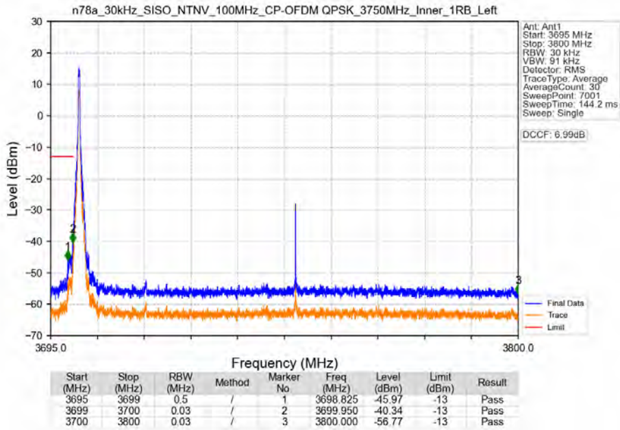
n78a_30kHz_SISO_NTNV_100MHz_CP-OFDM QPSK_3750MHz_Inner_1RB_Left
