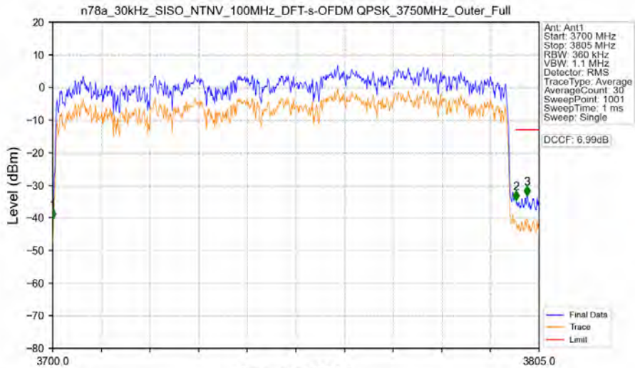
n78a_30kHz_SISO_NTNV_100MHz_DFT-s-OFDM QPSK_3750MHz_Outer_Full
