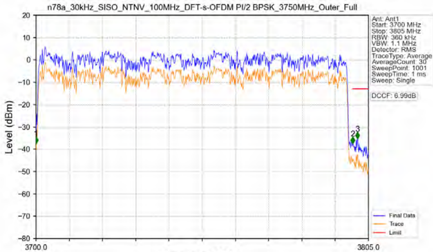
n78a_30kHz_SISO_NTNV_100MHz_DFT-s-OFDM PI/2 BPSK_3750MHz_Outer_Full
