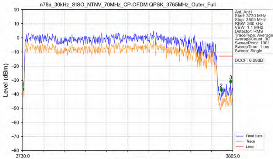
n78a_30kHz_SISO_NTNV_70MHz_CP-OFDM QPSK_3765MHz_Outer_Full
