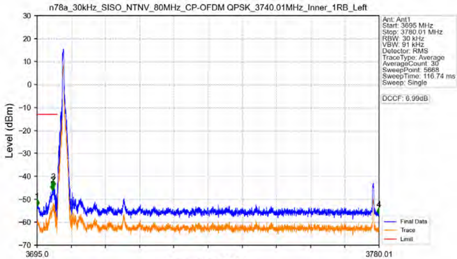
n78a_30kHz_SISO_NTNV_80MHz_CP-OFDM QPSK_3740.01MHz_Inner_1RB_Left
