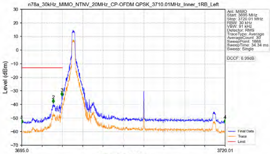
n78a_30kHz_MIMO_NTNV_20MHz_CP-OFDM QPSK_3710.01MHz_Inner_1RB_Left
