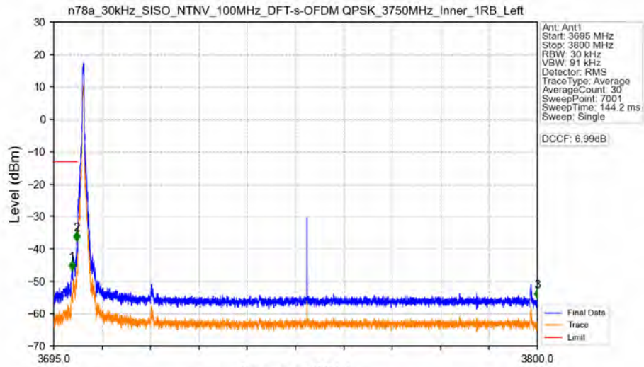
n78a_30kHz_SISO_NTNV_100MHz_DFT-s-OFDM_QPSK_3750MHz_Inner_1RB_Left
