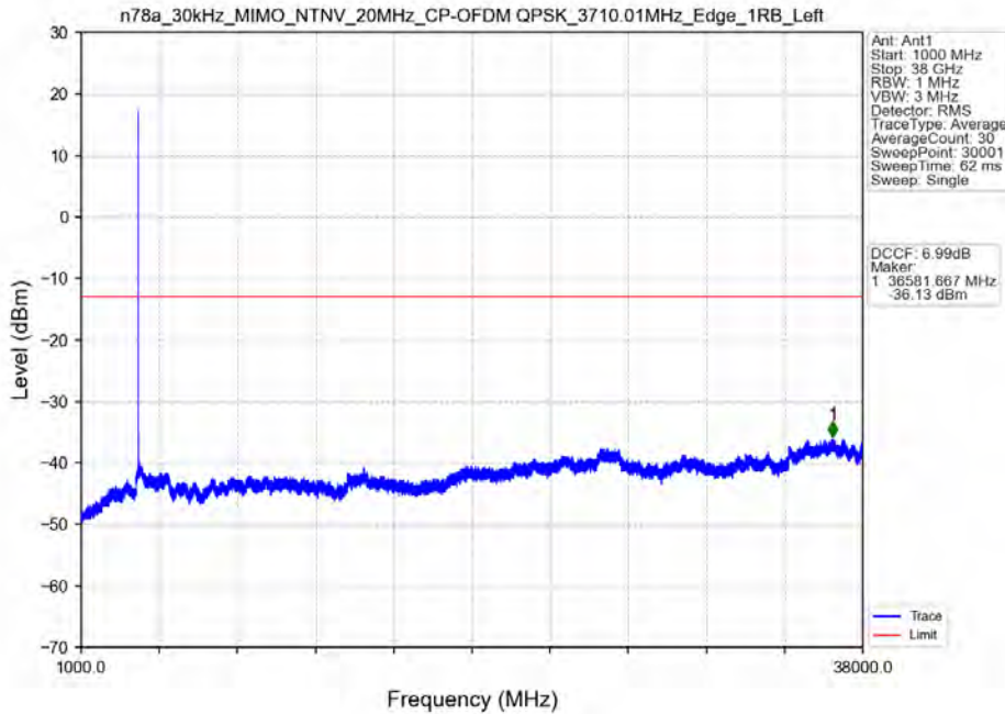
n78a_30kHz_MIMO_NTNV_20MHz_CP-OFDM QPSK_3710.01MHz_Edge_1RB_Left
