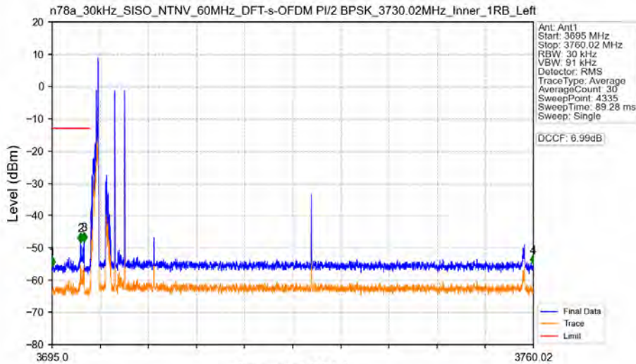
n78a_30kHz_SISO_NTNV_60MHz_DFT-s-OFDM PI/2 BPSK_3730.02MHz_Inner_1RB_Left
