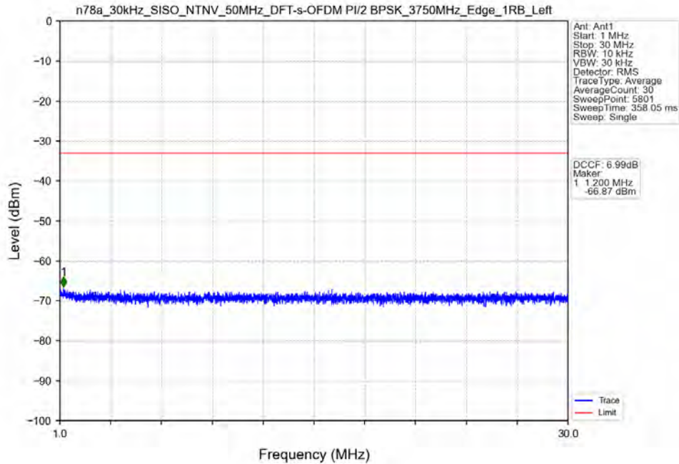
n78a_30kHz_SISO_NTNV_50MHz_DFT-s-OFDM PI/2 BPSK_3750MHz_Edge_1RB_Left
