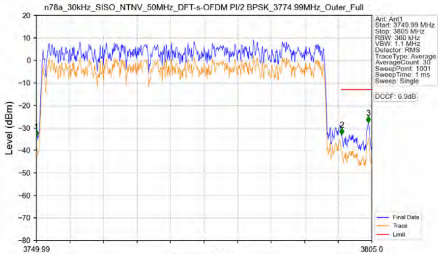
n78a_30kHz_SISO_NTNV_50MHz_DFT-s-OFDM PI/2 BPSK_3774.99MHz_Outer_Full
