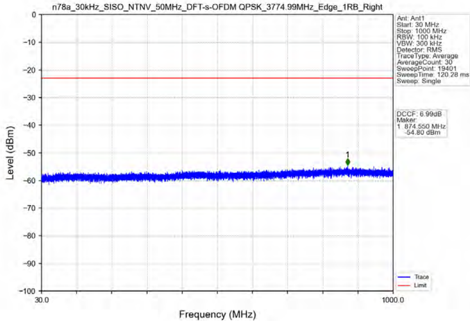
n78a_30kHz_SISO_NTNV_50MHz_DFT-s-OFDM QPSK_3774.99MHz_Edge_1RB_Right
