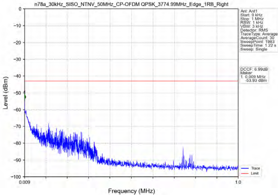
n78a_30kHz_SISO_NTNV_50MHz_CP-OFDM QPSK_3774.99MHz_Edge_1RB_Right
