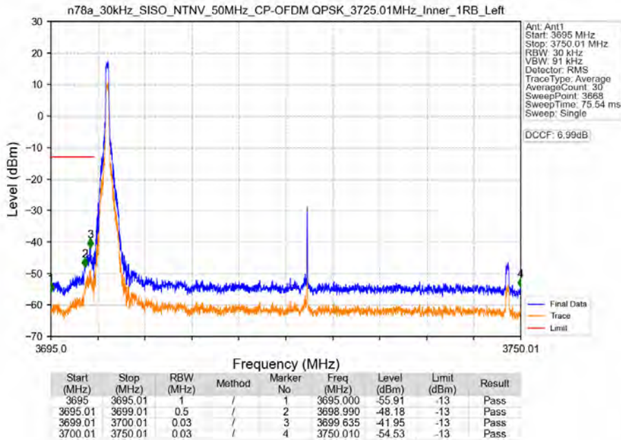
n78a_30kHz_SISO_NTNV_50MHz_CP-OFDM QPSK_3725.01MHz_Inner_1RB_Left
