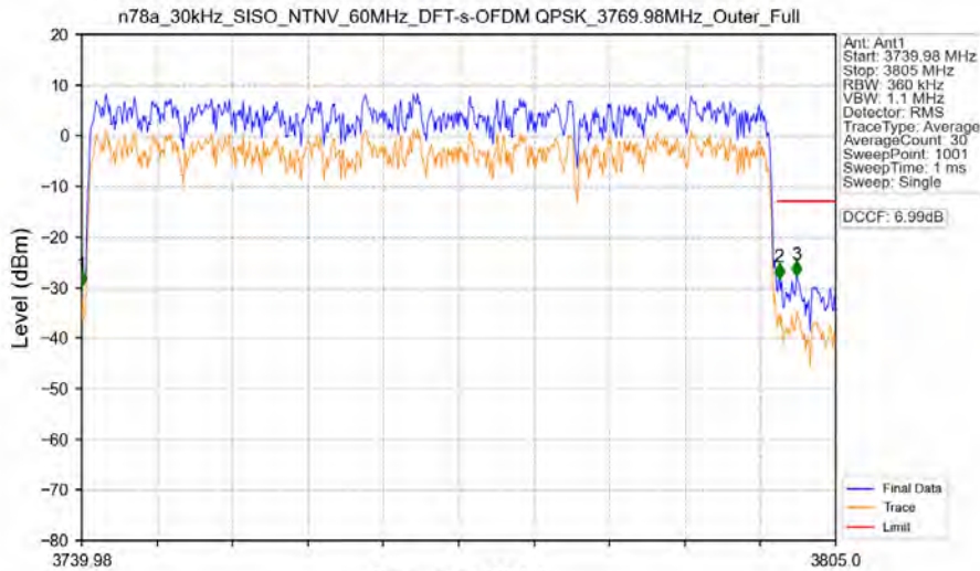
n78a_30kHz_SISO_NTNV_60MHz_DFT-s-OFDM QPSK_3769.98MHz_Outer_Full
