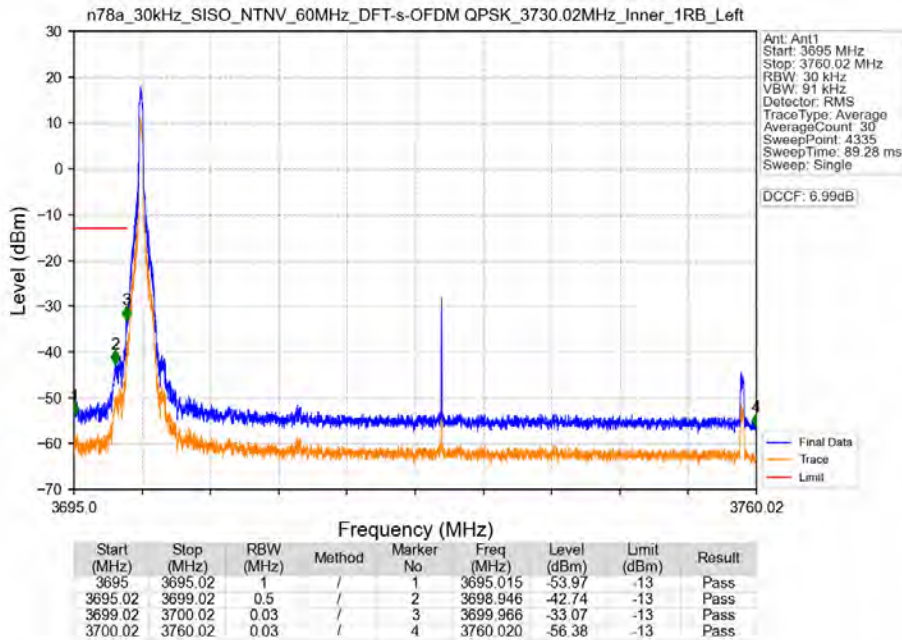
n78a_30kHz_SISO_NTNV_60MHz_DFT-s-OFDM_QPSK_3730.02MHz_Inner_1RB_Left
