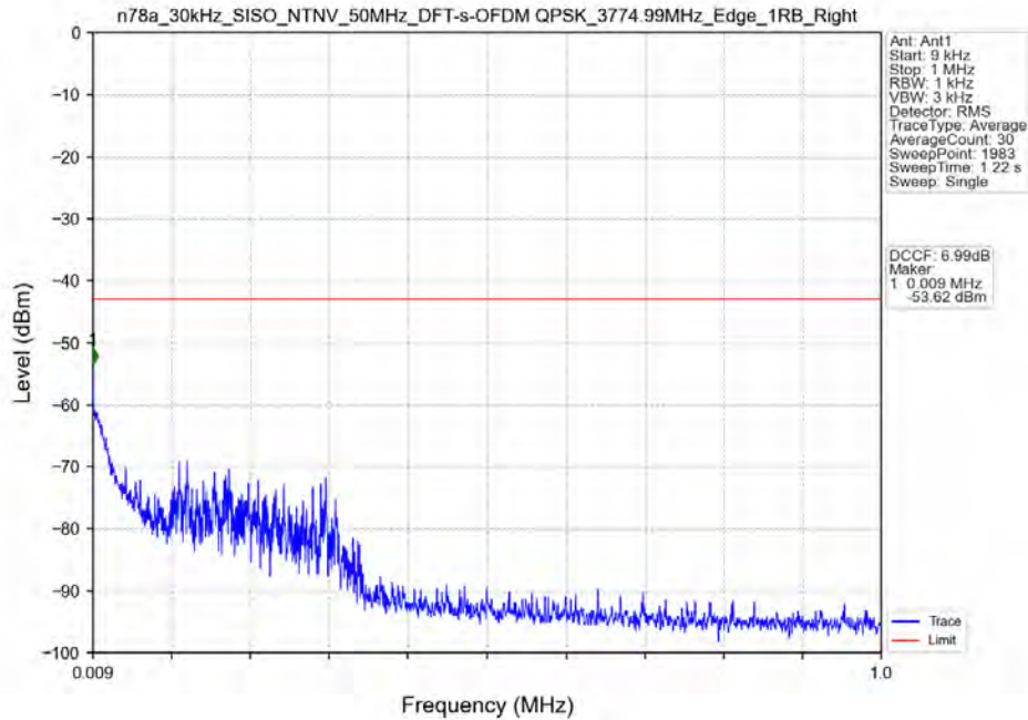
n78a_30kHz_SISO_NTNV_50MHz_DFT-s-OFDM QPSK_3774.99MHz_Edge_1RB_Right
