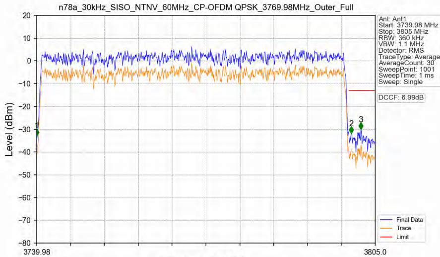
n78a_30kHz_SISO_NTNV_60MHz_CP-OFDM QPSK_3769.98MHz_Outer_Full
