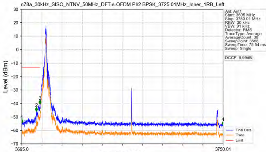
n78a_30kHz_SISO_NTNV_50MHz_DFT-s-OFDM PI/2 BPSK_3725.01MHz_Inner_1RB_Left
