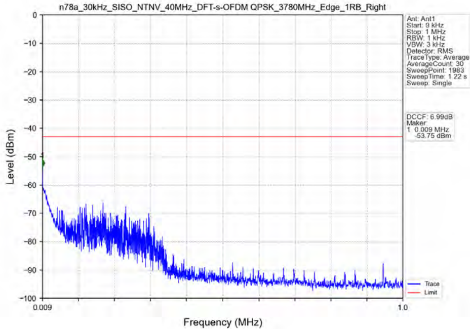
n78a_30kHz_SISO_NTNV_40MHz_DFT-s-OFDM_QPSK_3780MHz_Edge_1RB_Right
