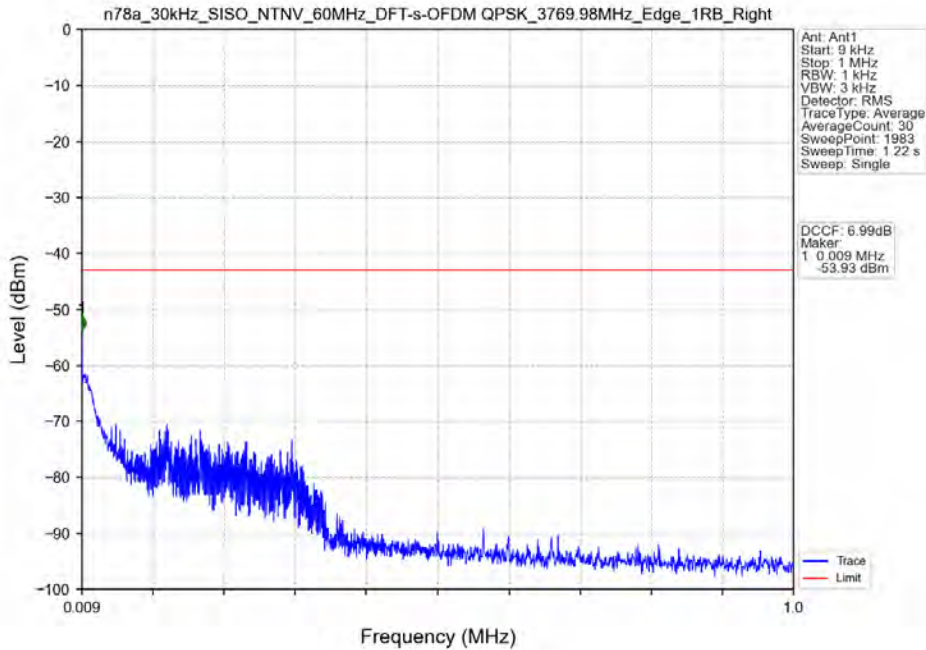
n78a_30kHz_SISO_NTNV_60MHz_DFT-s-OFDM QPSK_3769.98MHz_Edge_1RB_Right
