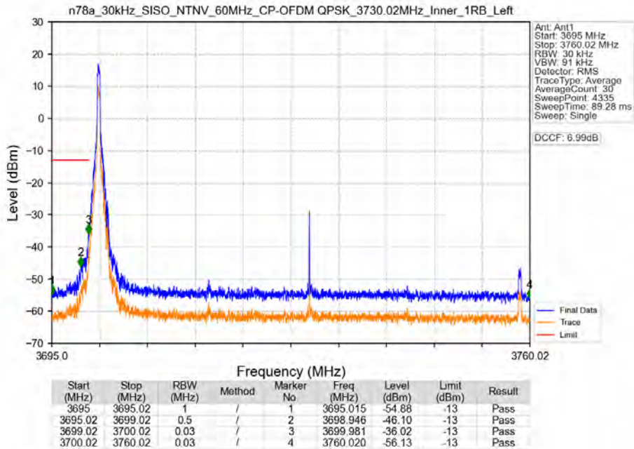
n78a_30kHz_SISO_NTNV_60MHz_CP-OFDM QPSK_3730.02MHz_Inner_1RB_Left
