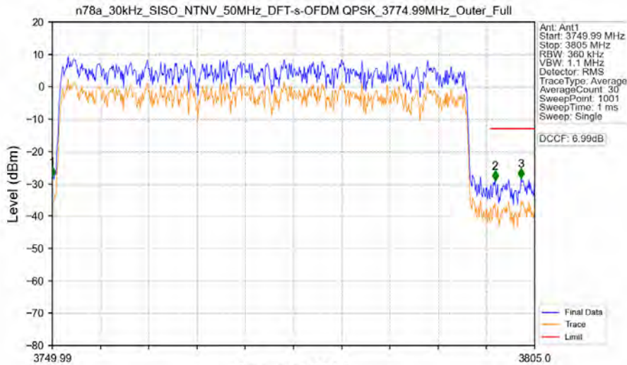
n78a_30kHz_SISO_NTNV_50MHz_DFT-s-OFDM QPSK_3774.99MHz_Outer_Full
