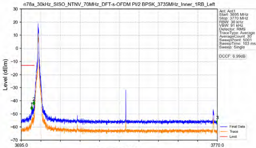
n78a_30kHz_SISO_NTNV_70MHz_DFT-s-OFDM PI/2 BPSK_3735MHz_Inner_1RB_Left
