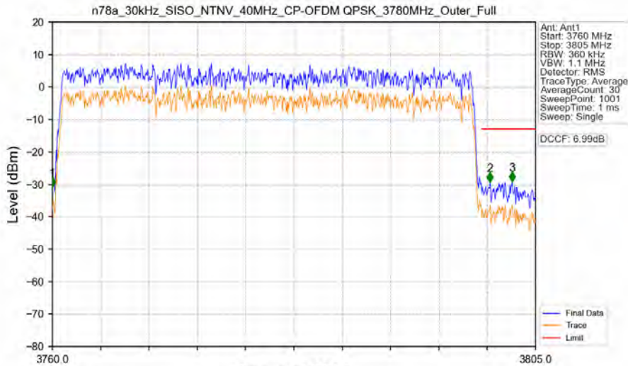
n78a_30kHz_SISO_NTNV_40MHz_CP-OFDM QPSK_3780MHz_Outer_Full
