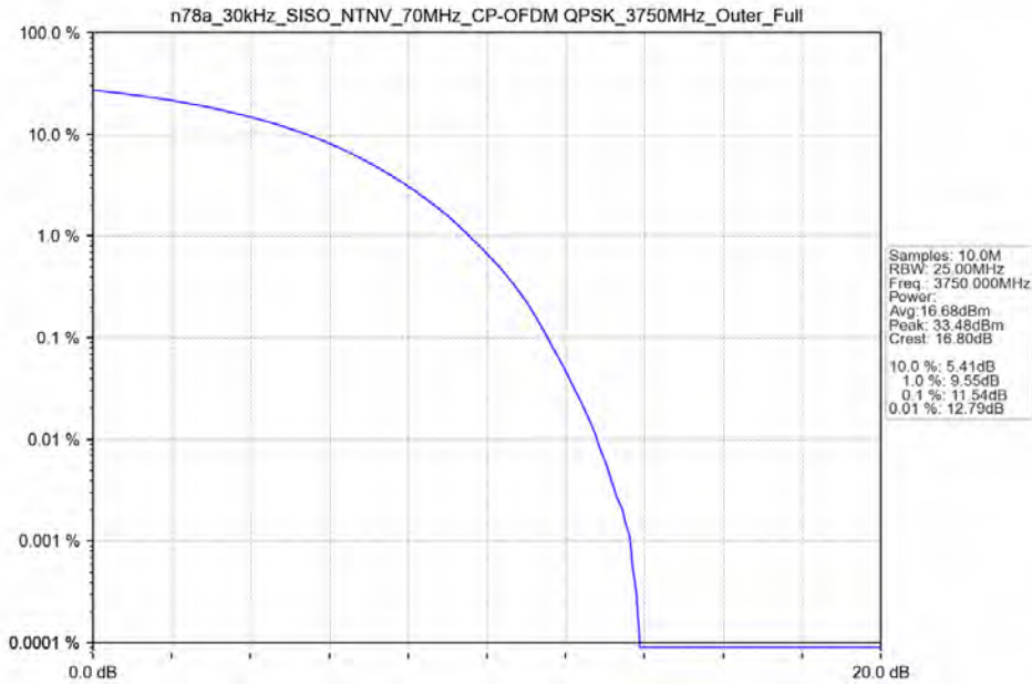
n78a_30kHz_SISO_NTNV_70MHz_CP-OFDM QPSK_3750MHz_Outer_Full
