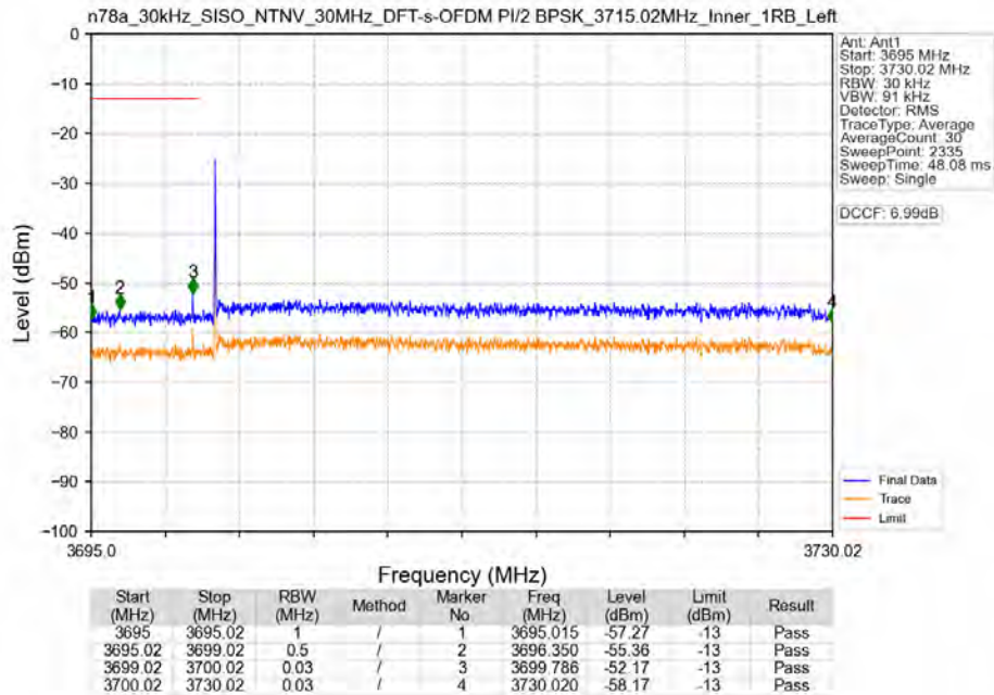
n78a_30kHz_SISO_NTNV_30MHz_DFT-s-OFDM PI/2 BPSK_3715.02MHz_Inner_1RB_Left
