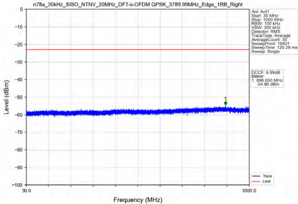
n78a_30kHz_SISO_NTNV_20MHz_DFT-s-OFDM QPSK_3789.99MHz_Edge_1RB_Right
