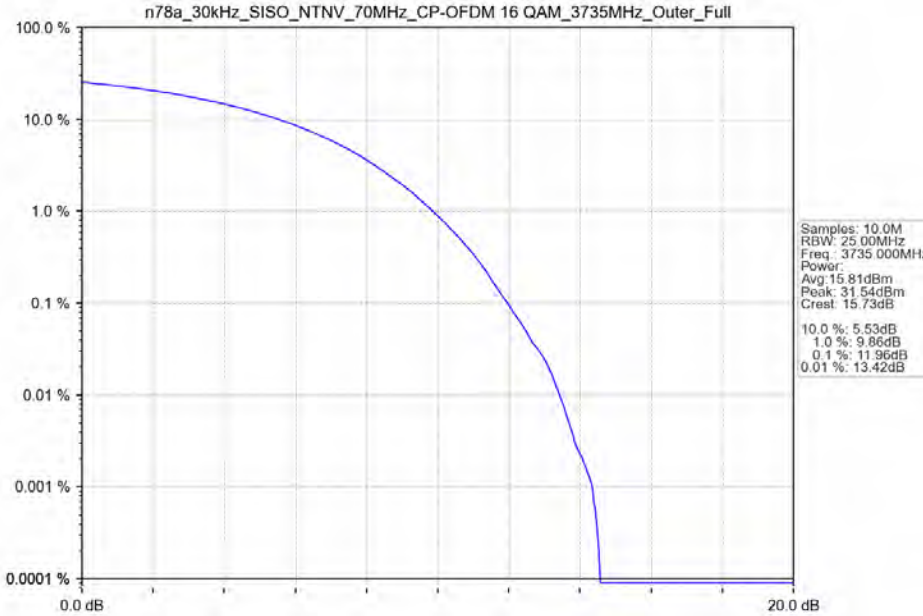
n78a_30kHz_SISO_NTNV_70MHz_CP-OFDM_16_QAM_3735MHz_Outer_Full
