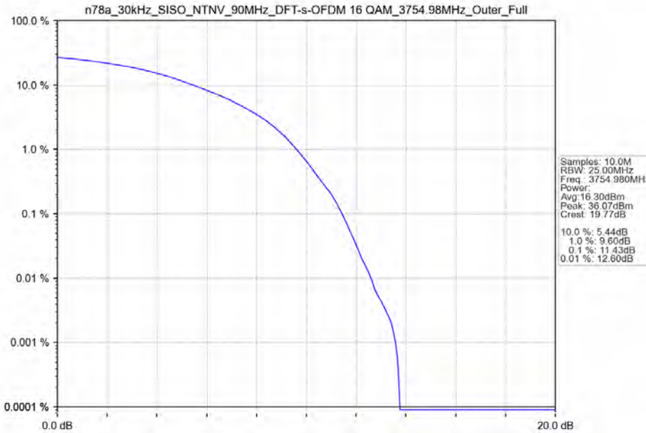
n78a_30kHz_SISO_NTNV_90MHz_DFT-s-OFDM 16 QAM_3754.98MHz_Outer_Full
