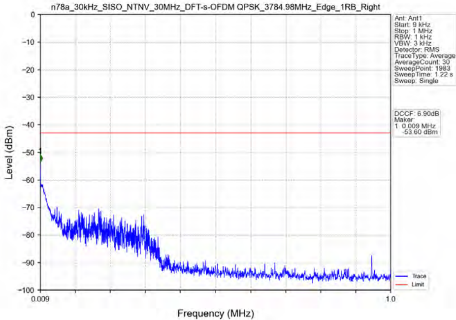
n78a_30kHz_SISO_NTNV_30MHz_DFT-s-OFDM QPSK_3784.98MHz_Edge_1RB_Right
