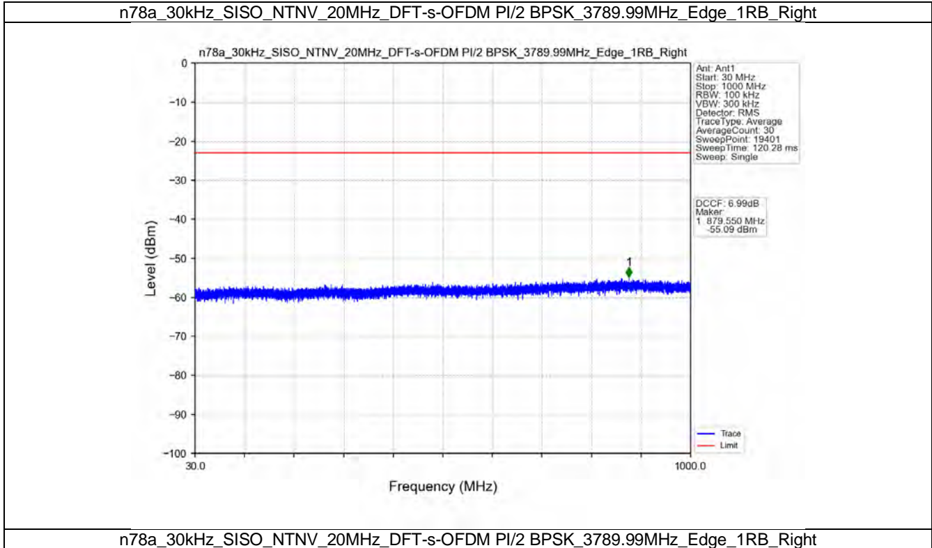
n78a_30kHz_SISO_NTNV_20MHz_DFT-s-OFDM PI/2 BPSK_3789.99MHz_Edge_1RB_Right
