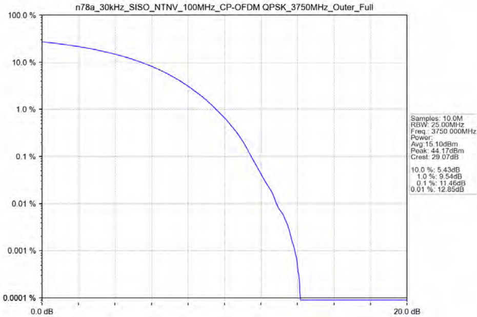
n78a_30kHz_SISO_NTNV_100MHz_CP-OFDM QPSK_3750MHz_Outer_Full
