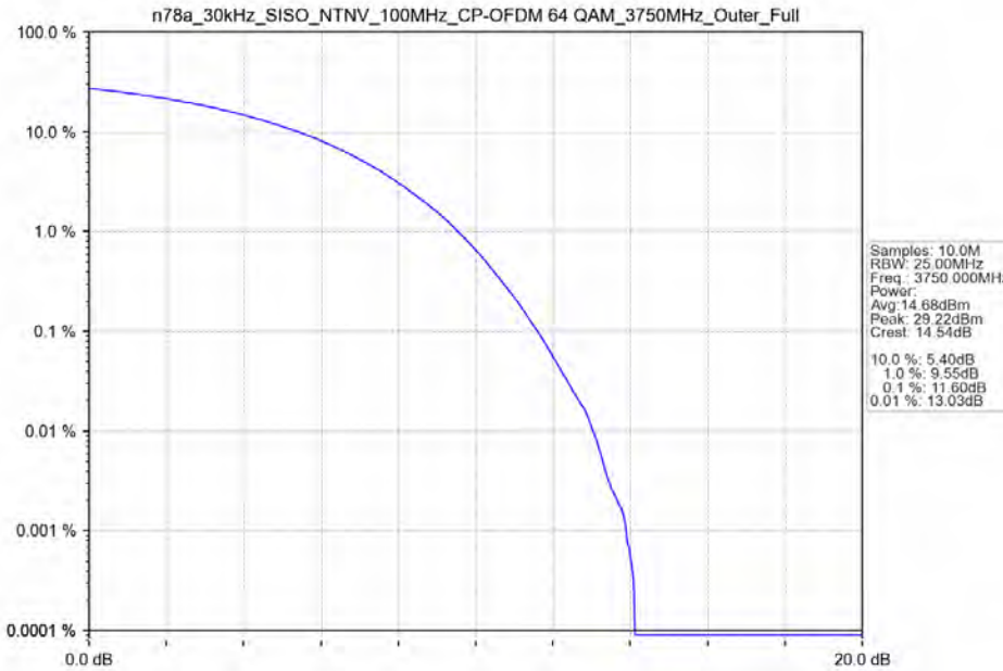
n78a_30kHz_SISO_NTNV_100MHz_CP-OFDM 64 QAM_3750MHz_Outer_Full
