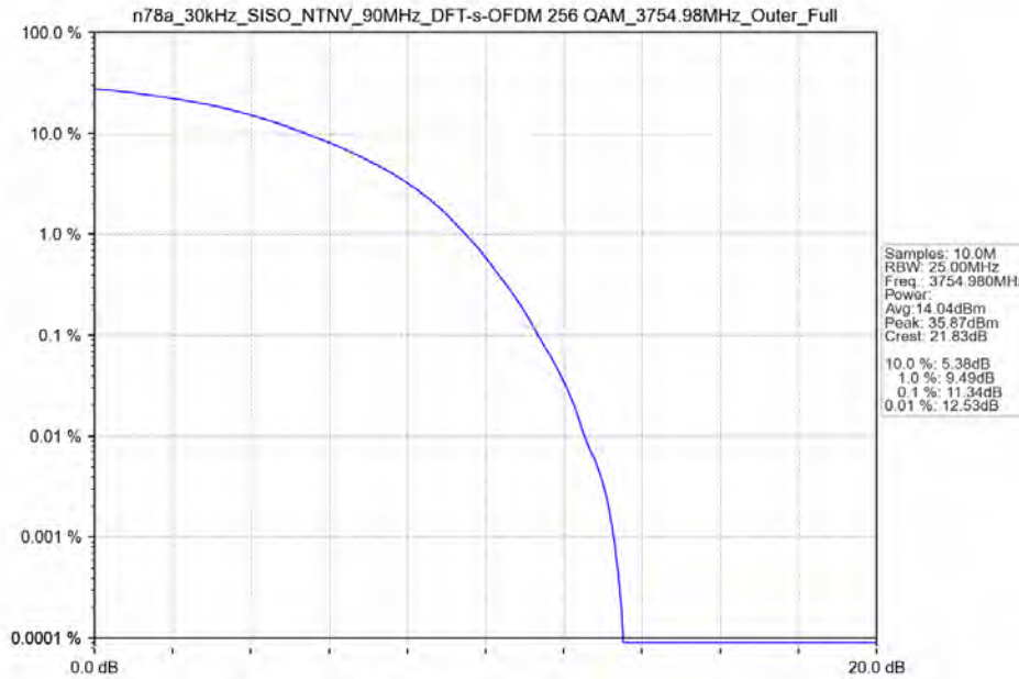
n78a_30kHz_SISO_NTNV_90MHz_DFT-s-OFDM 256 QAM_3754.98MHz_Outer_Full
