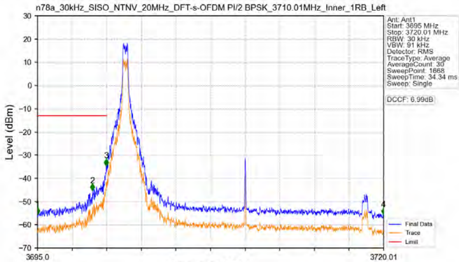
n78a_30kHz_SISO_NTNV_20MHz_DFT-s-OFDM PI/2 BPSK_3710.01MHz_Inner_1RB_Left
