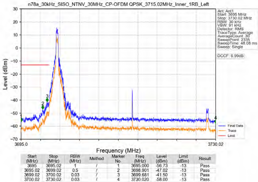
n78a_30kHz_SISO_NTNV_30MHz_CP-OFDM QPSK_3715.02MHz_Inner_1RB_Left
