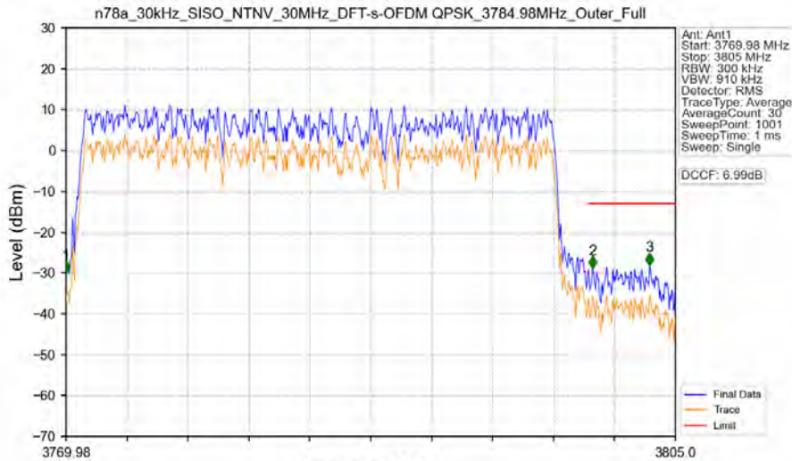
n78a_30kHz_SISO_NTNV_30MHz_DFT-s-OFDM QPSK_3784.98MHz_Outer_Full
