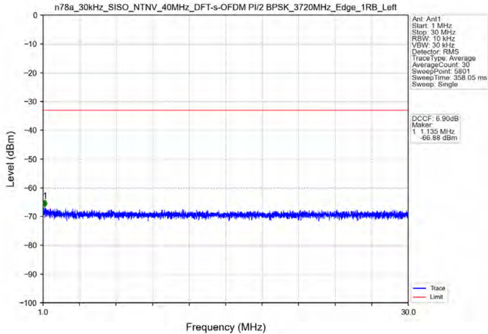
n78a_30kHz_SISO_NTNV_40MHz_DFT-s-OFDM PI/2 BPSK_3720MHz_Edge_1RB_Left
