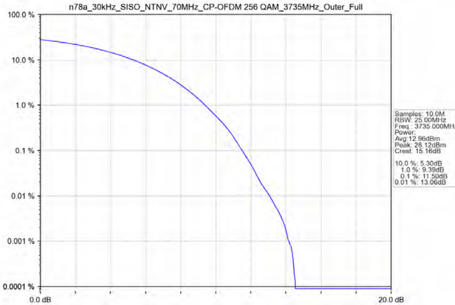
n78a_30kHz_SISO_NTNV_70MHz_CP-OFDM 256 QAM_3735MHz_Outer_Full
