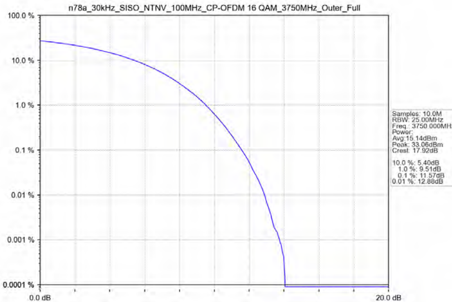
n78a_30kHz_SISO_NTNV_100MHz_CP-OFDM 16 QAM_3750MHz_Outer_Full
