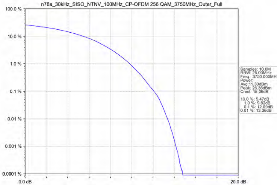
n78a_30kHz_SISO_NTNV_100MHz_CP-OFDM 256 QAM_3750MHz_Outer_Full
