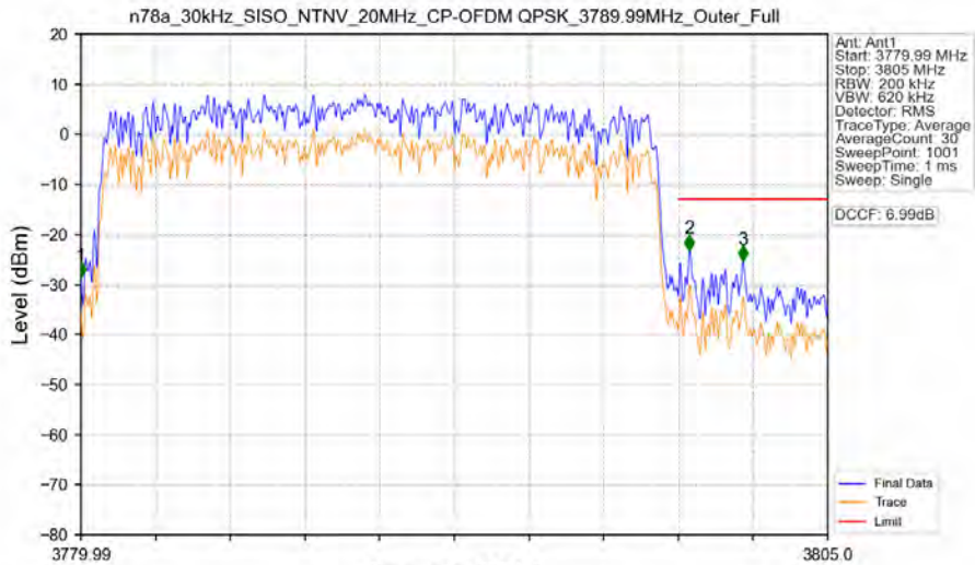
n78a_30kHz_SISO_NTNV_20MHz_CP-OFDM QPSK_3789.99MHz_Outer_Full
