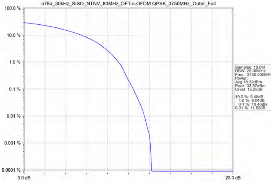
n78a_30kHz_SISO_NTNV_80MHz_DFT-s-OFDM QPSK_3750MHz_Outer_Full
