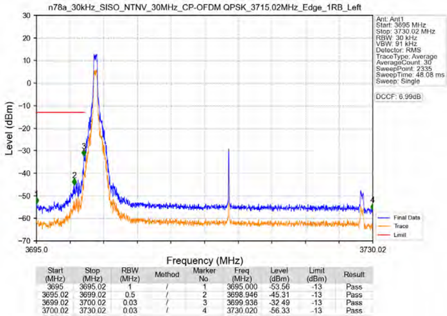
n78a_30kHz_SISO_NTNV_30MHz_CP-OFDM QPSK_3715.02MHz_Edge_1RB_Left
