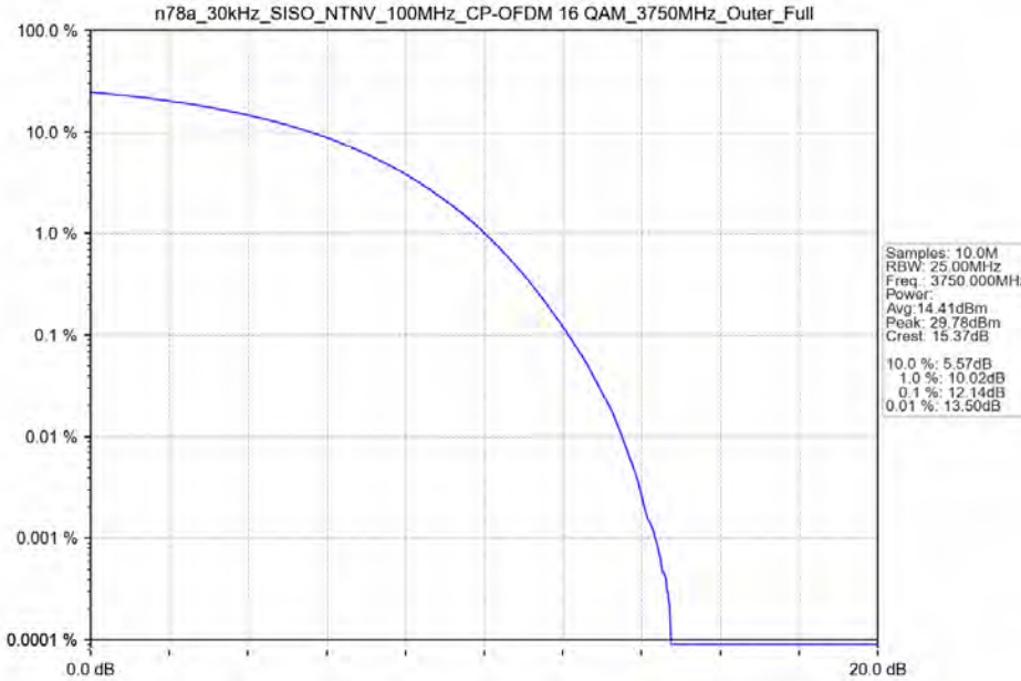
n78a_30kHz_SISO_NTNV_100MHz_CP-OFDM 16 QAM_3750MHz_Outer_Full
