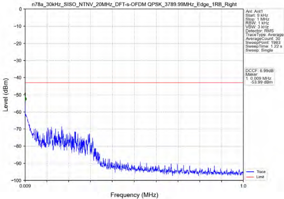
n78a_30kHz_SISO_NTNV_20MHz_DFT-s-OFDM_QPSK_3789.99MHz_Edge_1RB_Right
