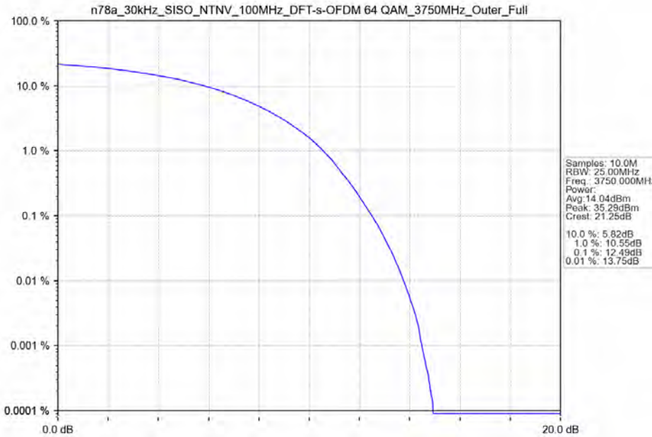
n78a_30kHz_SISO_NTNV_100MHz_DFT-s-OFDM 64 QAM_3750MHz_Outer_Full
