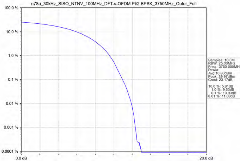
n78a_30kHz_SISO_NTNV_100MHz_DFT-s-OFDM PI/2 BPSK_3750MHz_Outer_Full
