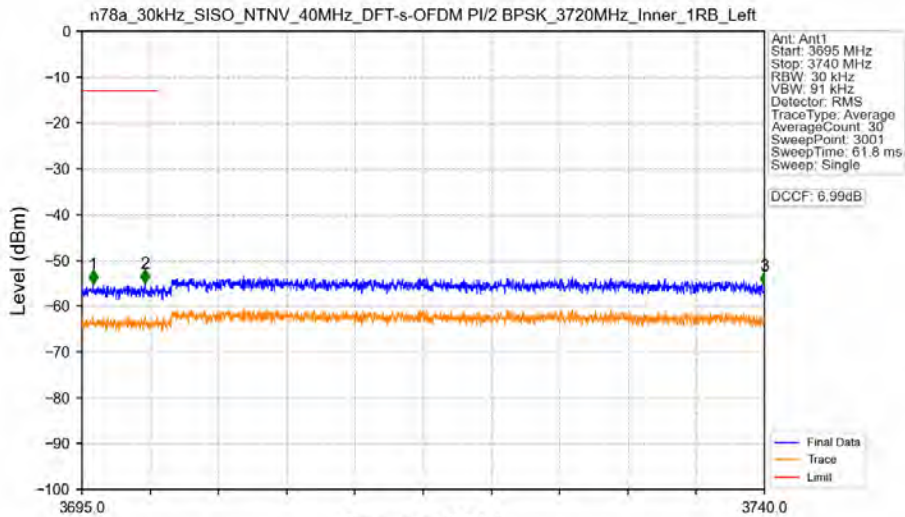
n78a_30kHz_SISO_NTNV_40MHz_DFT-s-OFDM PI/2 BPSK_3720MHz_Inner_1RB_Left
