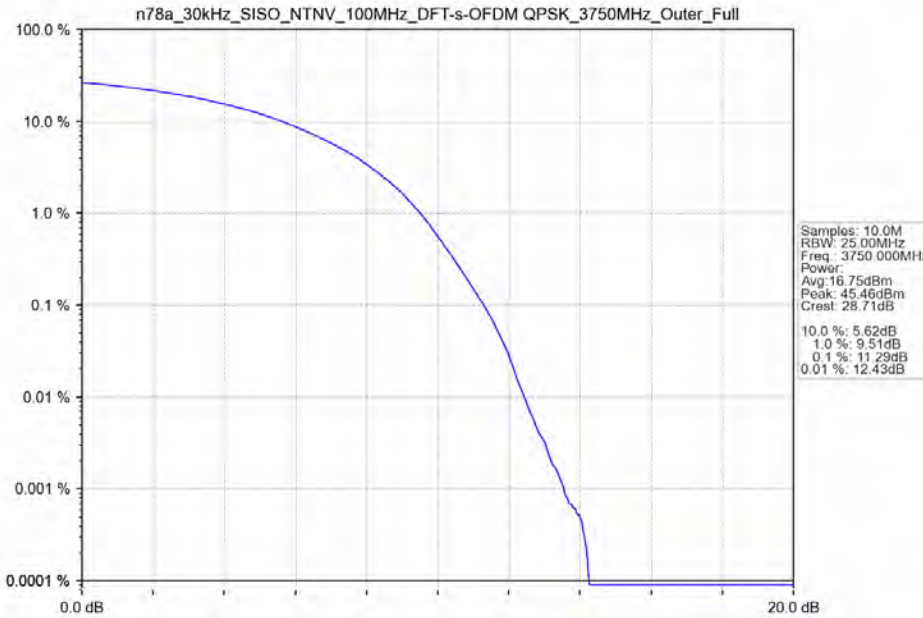
n78a_30kHz_SISO_NTNV_100MHz_DFT-s-OFDM QPSK_3750MHz_Outer_Full
