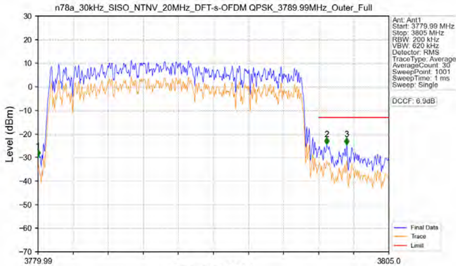
n78a_30kHz_SISO_NTNV_20MHz_DFT-s-OFDM QPSK_3789.99MHz_Outer_Full
