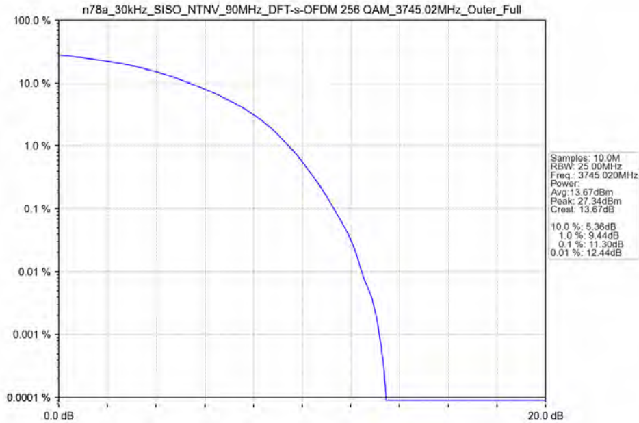
n78a_30kHz_SISO_NTNV_90MHz_DFT-s-OFDM 256 QAM_3745.02MHz_Outer_Full
