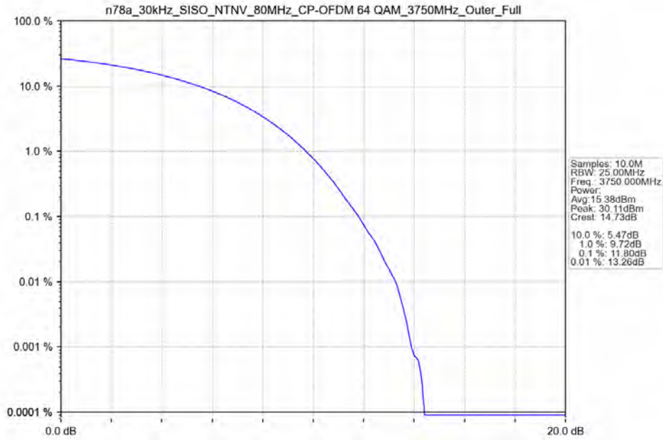
n78a_30kHz_SISO_NTNV_80MHz_CP-OFDM 64 QAM_3750MHz_Outer_Full
