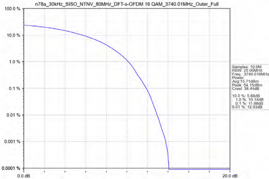
n78a_30kHz_SISO_NTNV_80MHz_DFT-s-OFDM_16_QAM_3740.01MHz_Outer_Full
