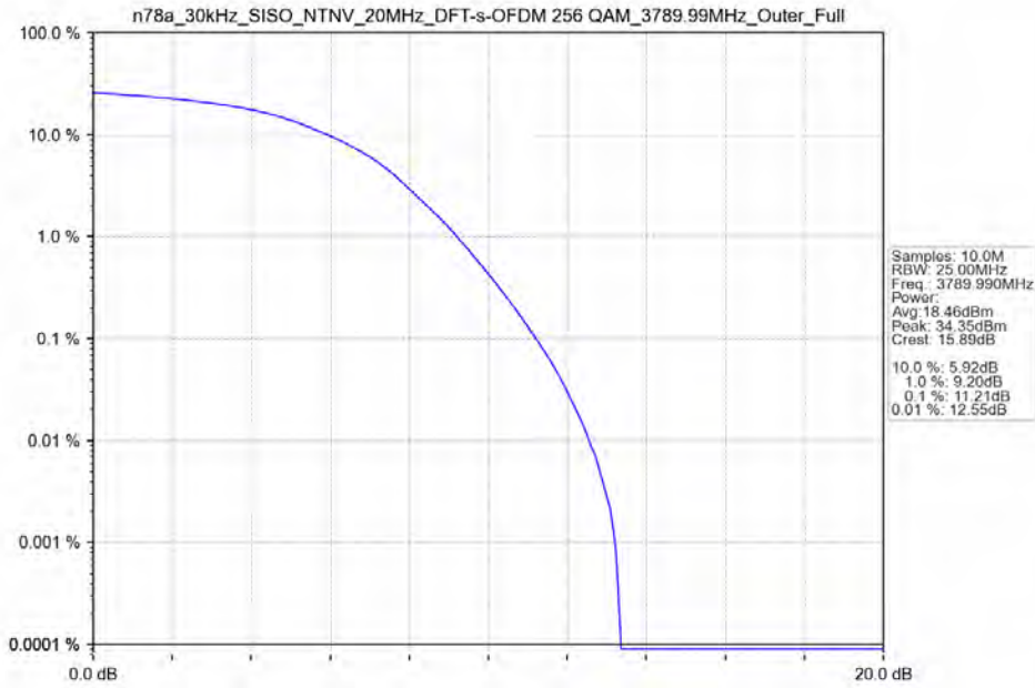
n78a_30kHz_SISO_NTNV_20MHz_DFT-s-OFDM 256 QAM_3789.99MHz_Outer_Full
