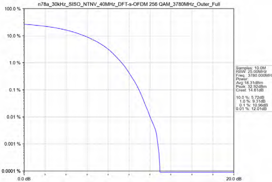
n78a_30kHz_SISO_NTNV_40MHz_DFT-s-OFDM 256 QAM_3780MHz_Outer_Full
