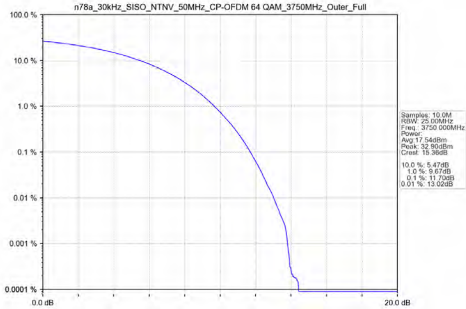
n78a_30kHz_SISO_NTNV_50MHz_CP-OFDM 64 QAM_3750MHz_Outer_Full
