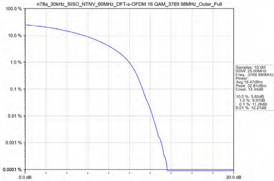
n78a_30kHz_SISO_NTNV_60MHz_DFT-s-OFDM 16 QAM_3769.98MHz_Outer_Full
