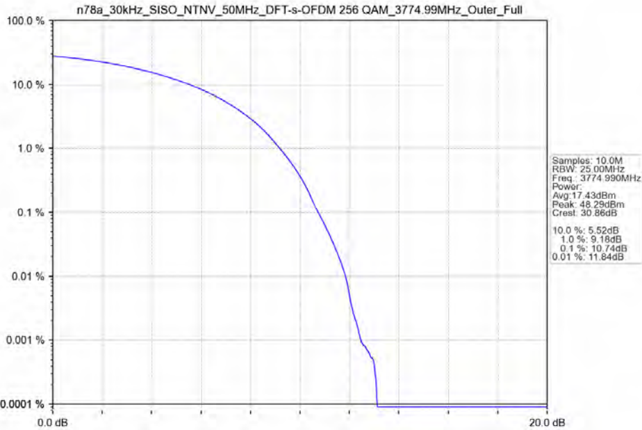
n78a_30kHz_SISO_NTNV_50MHz_DFT-s-OFDM 256 QAM_3774.99MHz_Outer_Full
