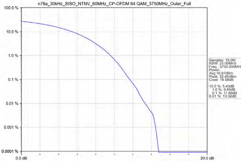
n78a_30kHz_SISO_NTNV_60MHz_CP-OFDM 64 QAM_3750MHz_Outer_Full
