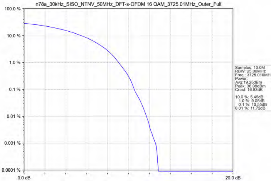
n78a_30kHz_SISO_NTNV_50MHz_DFT-s-OFDM_16_QAM_3725.01MHz_Outer_Full
