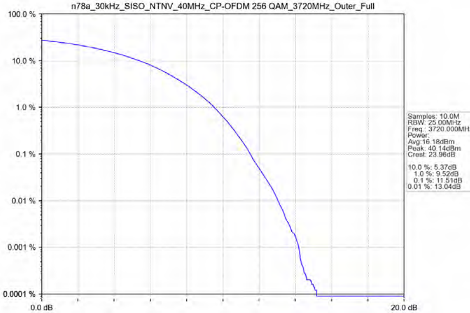
n78a_30kHz_SISO_NTNV_40MHz_CP-OFDM 256 QAM_3720MHz_Outer_Full
