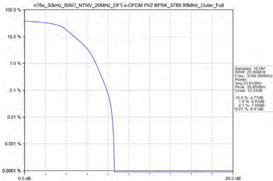
n78a_30kHz_SISO_NTNV_20MHz_DFT-s-OFDM PI/2 BPSK_3789.99MHz_Outer_Full
