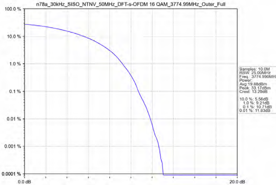
n78a_30kHz_SISO_NTNV_50MHz_DFT-s-OFDM 16 QAM_3774.99MHz_Outer_Full
