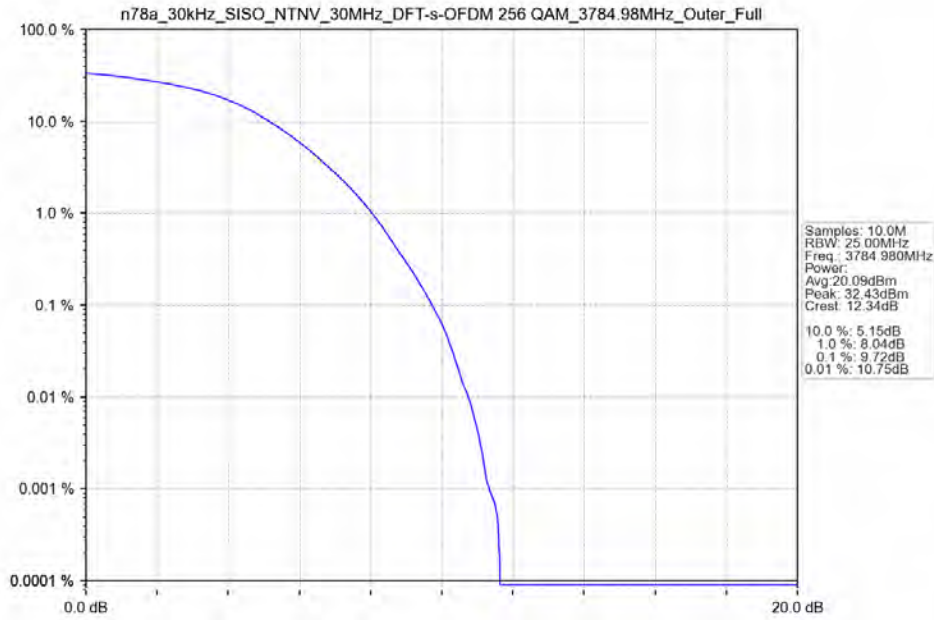
n78a_30kHz_SISO_NTNV_30MHz_DFT-s-OFDM 256 QAM_3784.98MHz_Outer_Full
