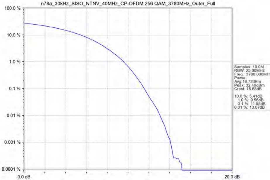
n78a_30kHz_SISO_NTNV_40MHz_CP-OFDM 256 QAM_3780MHz_Outer_Full
