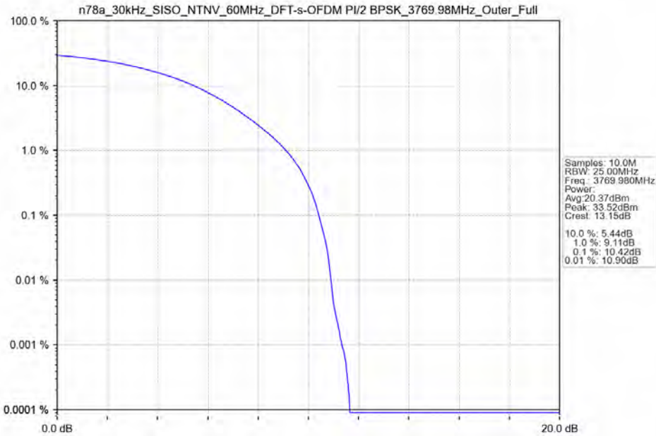
n78a_30kHz_SISO_NTNV_60MHz_DFT-s-OFDM PI/2 BPSK_3769.98MHz_Outer_Full
