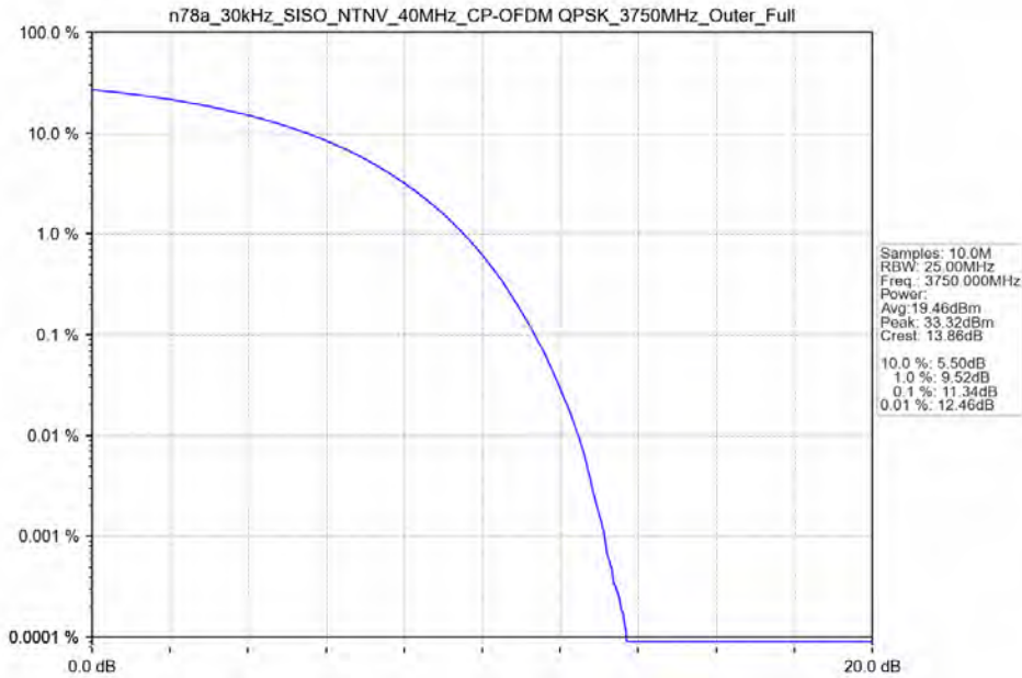
n78a_30kHz_SISO_NTNV_40MHz_CP-OFDM QPSK_3750MHz_Outer_Full
