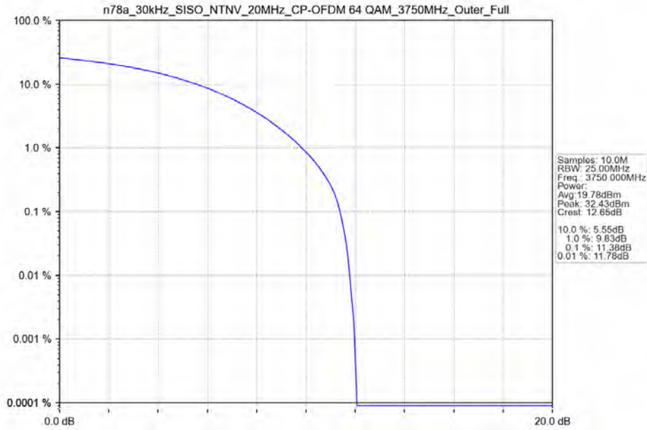
n78a_30kHz_SISO_NTNV_20MHz_CP-OFDM 64 QAM_3750MHz_Outer_Full
