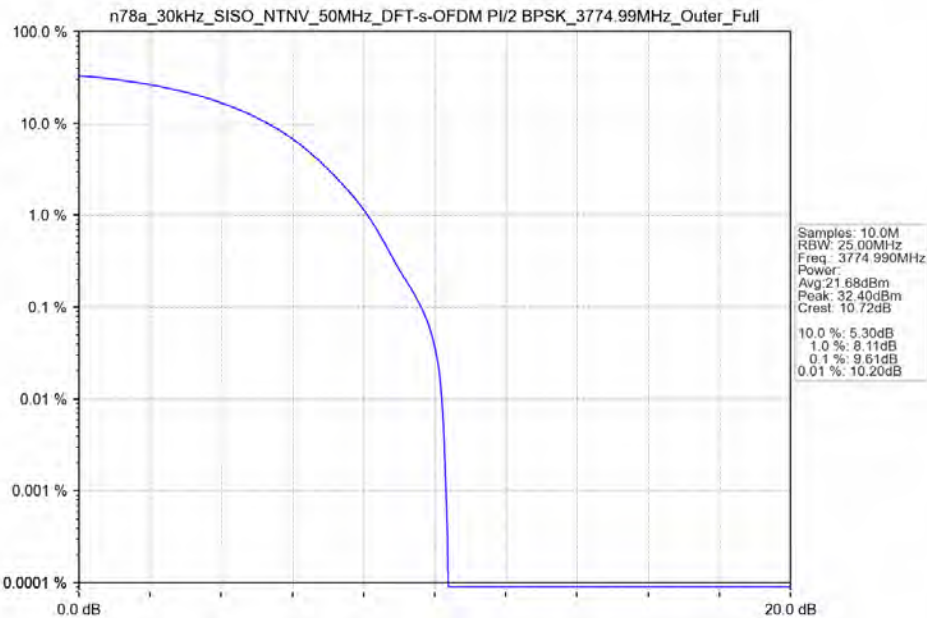
n78a_30kHz_SISO_NTNV_50MHz_DFT-s-OFDM PI/2 BPSK_3774.99MHz_Outer_Full
