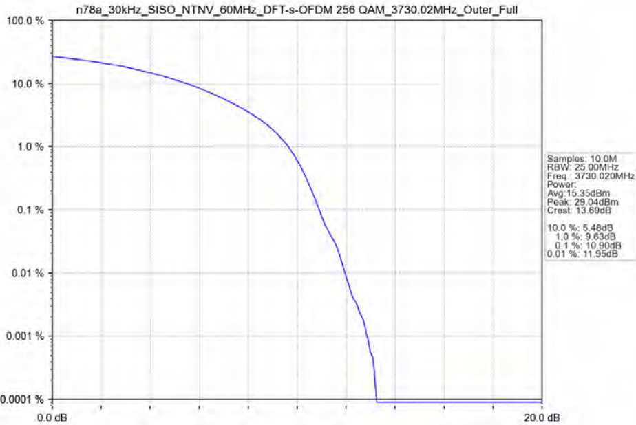
n78a_30kHz_SISO_NTNV_60MHz_DFT-s-OFDM 256 QAM_3730.02MHz_Outer_Full
