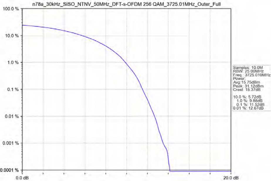
n78a_30kHz_SISO_NTNV_50MHz_DFT-s-OFDM 256 QAM_3725.01MHz_Outer_Full
