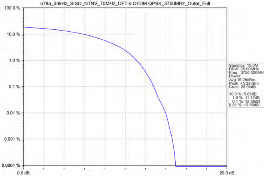
n78a_30kHz_SISO_NTNV_70MHz_DFT-s-OFDM QPSK_3750MHz_Outer_Full
