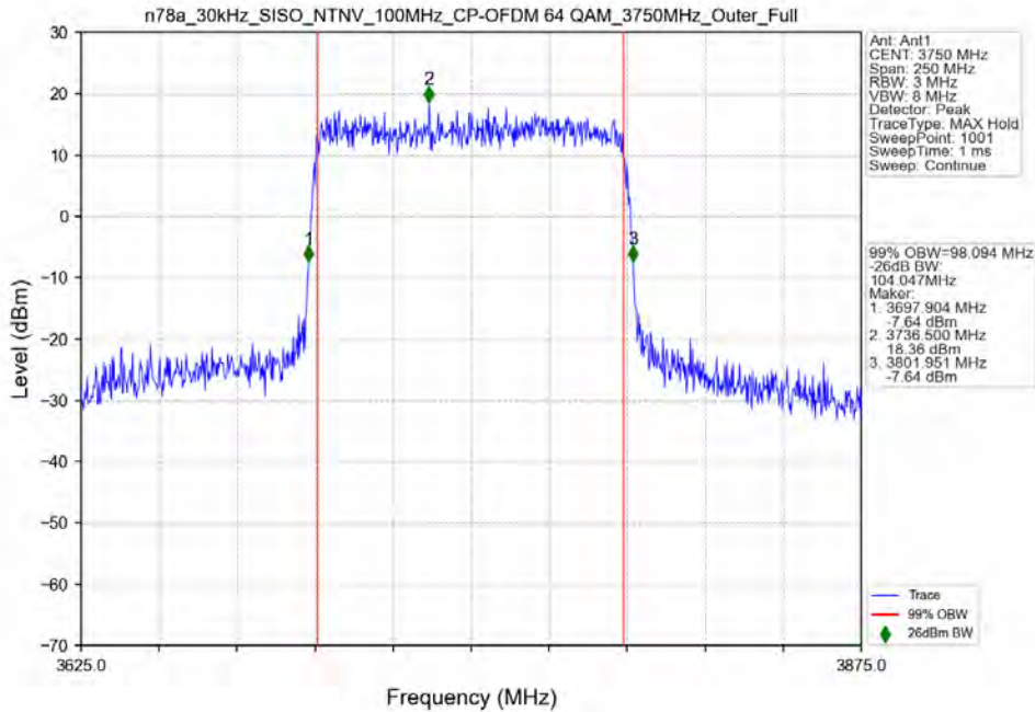
n78a_30kHz_SISO_NTNV_100MHz_CP-OFDM 64 QAM_3750MHz_Outer_Full
