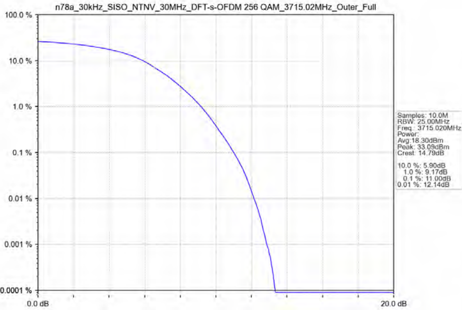
n78a_30kHz_SISO_NTNV_30MHz_DFT-s-OFDM 256 QAM_3715.02MHz_Outer_Full
