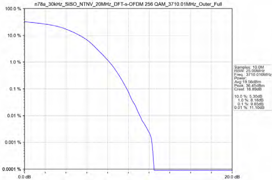
n78a_30kHz_SISO_NTNV_20MHz_DFT-s-OFDM 256 QAM_3710.01MHz_Outer_Full
