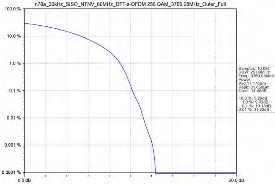
n78a_30kHz_SISO_NTNV_60MHz_DFT-s-OFDM 256 QAM_3769.98MHz_Outer_Full
