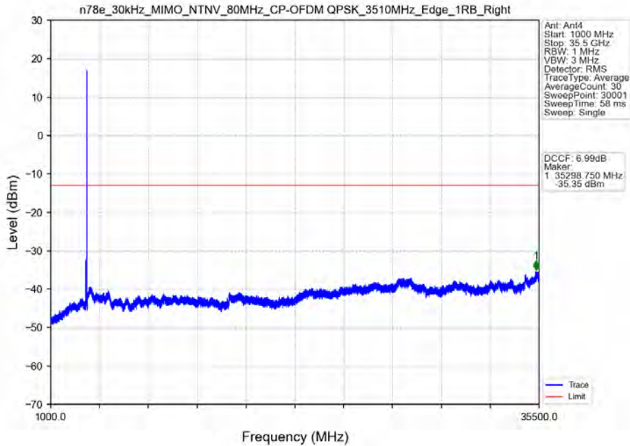
n78e_30kHz_MIMO_NTNV_80MHz_CP-OFDM QPSK_3510MHz_Edge_1RB_Right
