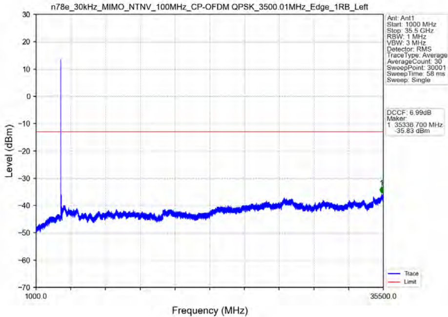
n78e_30kHz_MIMO_NTNV_100MHz_CP-OFDM QPSK_3500.01MHz_Edge_1RB_Left
