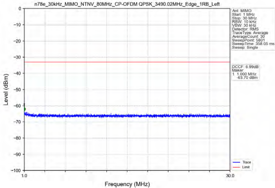
n78e_30kHz_MIMO_NTNV_80MHz_CP-OFDM QPSK_3490.02MHz_Edge_1RB_Left
