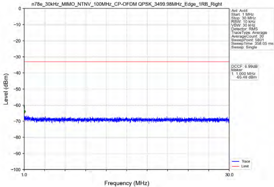
n78e_30kHz_MIMO_NTNV_100MHz_CP-OFDM QPSK_3499.98MHz_Edge_1RB_Right
