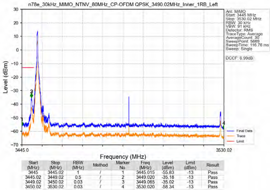
n78e_30kHz_MIMO_NTNV_80MHz_CP-OFDM QPSK_3490.02MHz_Inner_1RB_Left
