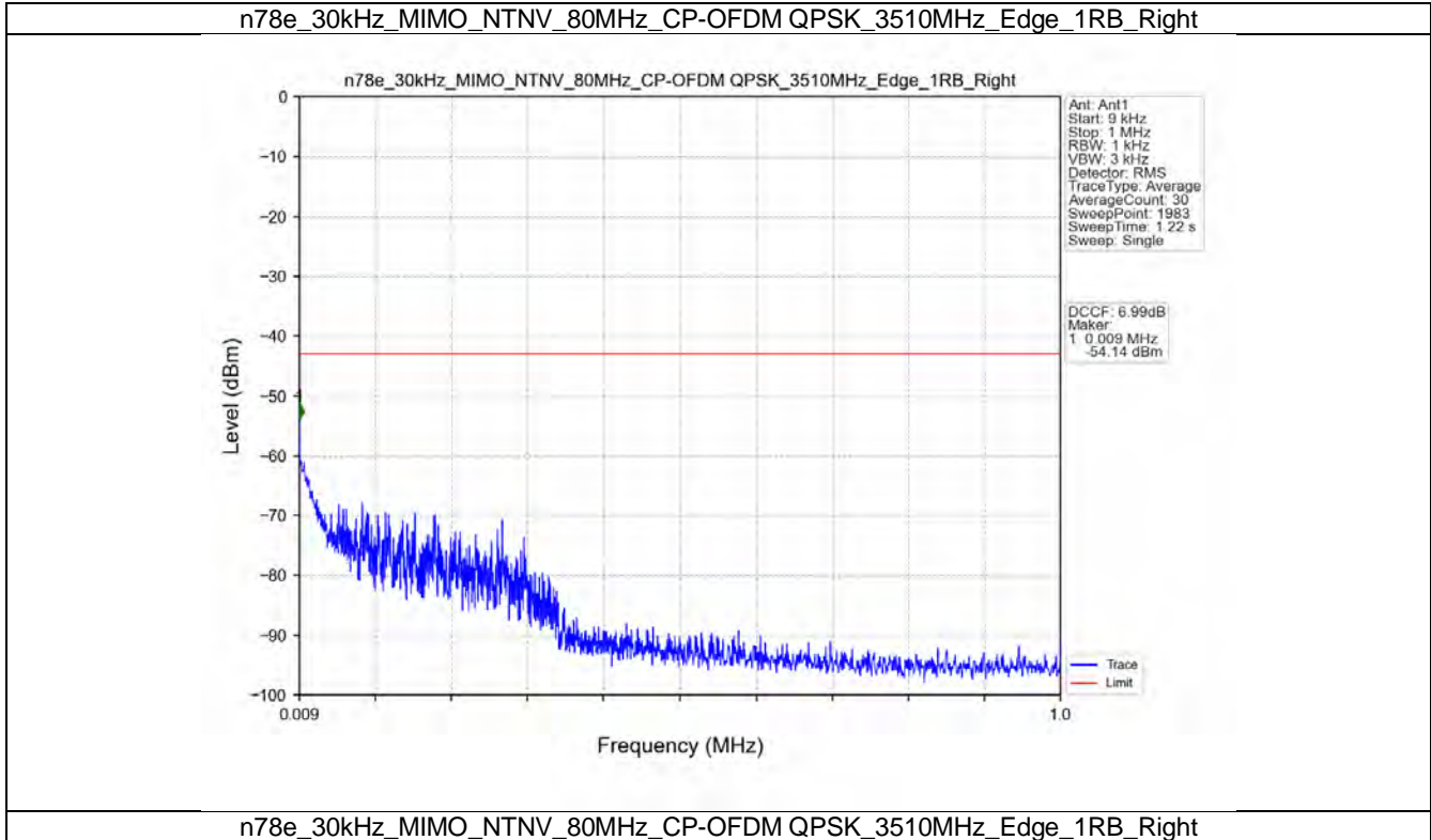
n78e_30kHz_MIMO_NTNV_80MHz_CP-OFDM_QPSK_3510MHz_Edge_1RB_Right
