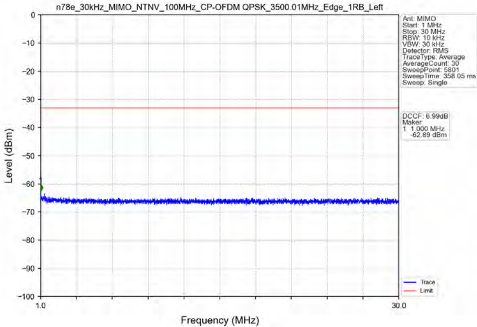
n78e_30kHz_MIMO_NTNV_100MHz_CP-OFDM QPSK_3500.01MHz_Edge_1RB_Left
