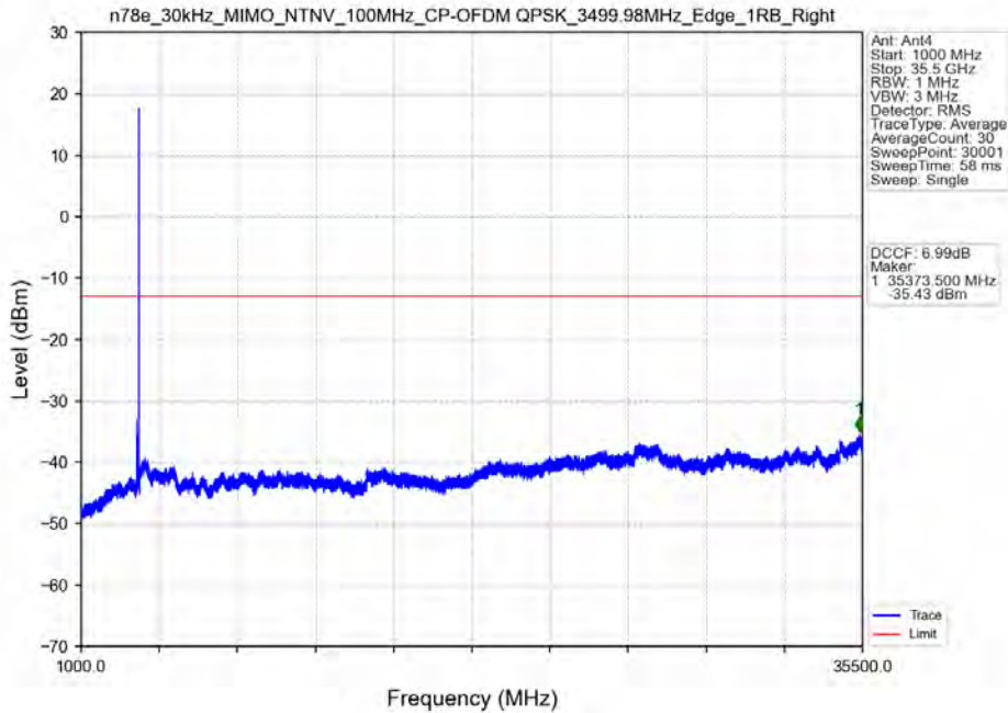
n78e_30kHz_MIMO_NTNV_100MHz_CP-OFDM QPSK_3499.98MHz_Edge_1RB_Right
