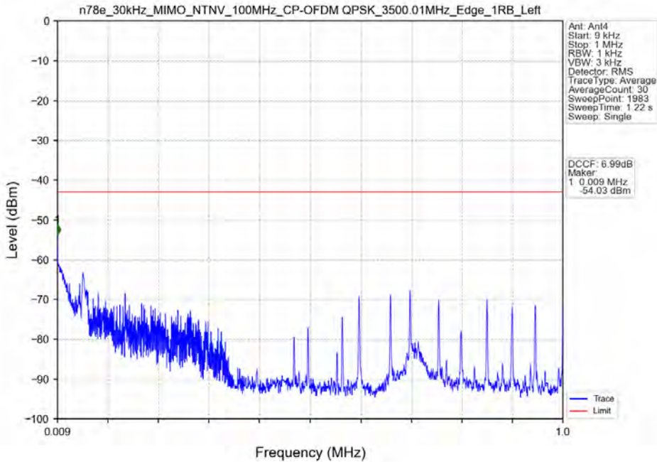
n78e_30kHz_MIMO_NTNV_100MHz_CP-OFDM QPSK_3500.01MHz_Edge_1RB_Left
