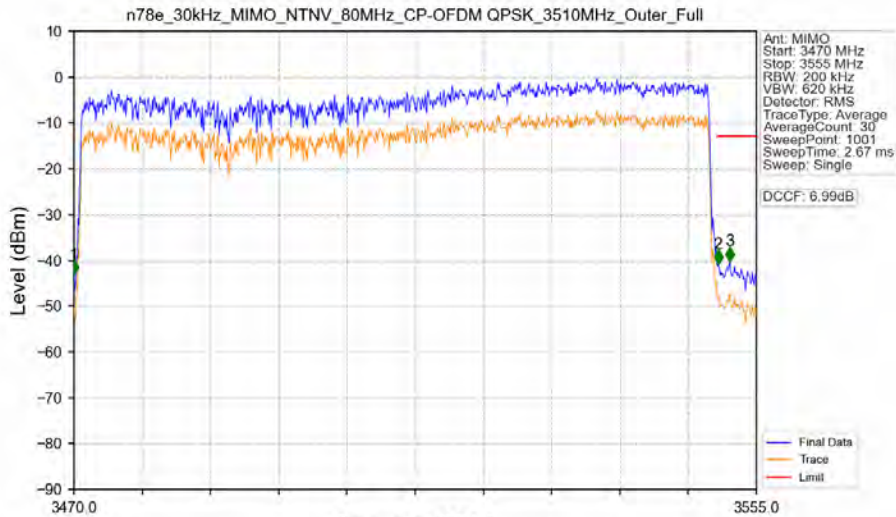
n78e_30kHz_MIMO_NTNV_80MHz_CP-OFDM_QPSK_3510MHz_Outer_Full
