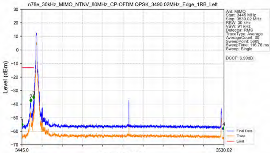
n78e_30kHz_MIMO_NTNV_80MHz_CP-OFDM QPSK_3490.02MHz_Edge_1RB_Left
