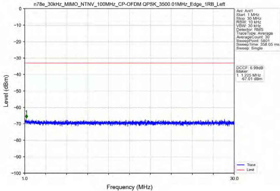
n78e_30kHz_MIMO_NTNV_100MHz_CP-OFDM QPSK_3500.01MHz_Edge_1RB_Left
