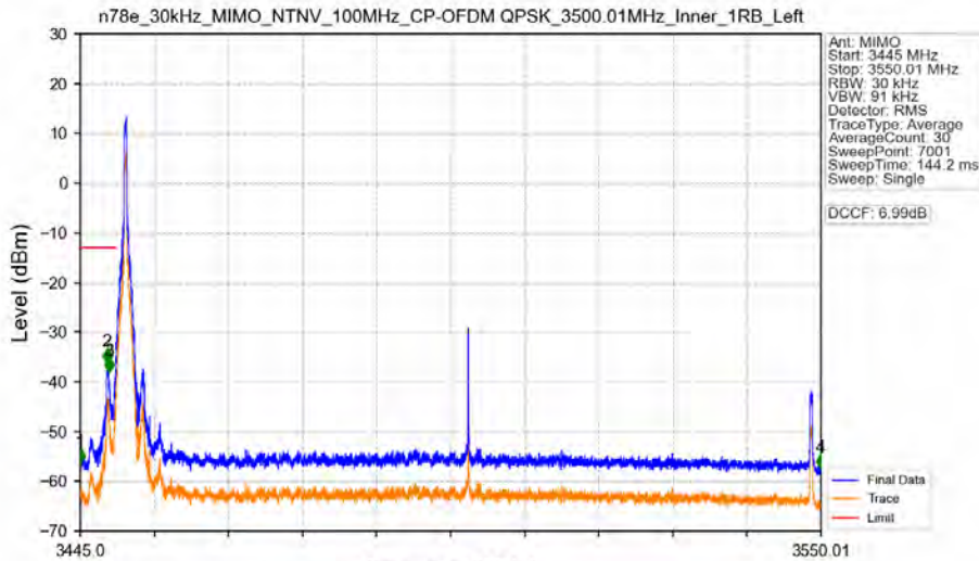
n78e_30kHz_MIMO_NTNV_100MHz_CP-OFDM QPSK_3500.01MHz_Inner_1RB_Left
