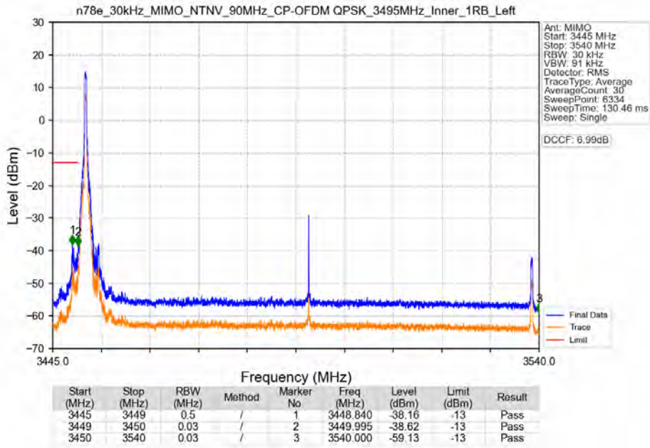
n78e_30kHz_MIMO_NTNV_90MHz_CP-OFDM QPSK_3495MHz_Inner_1RB_Left
