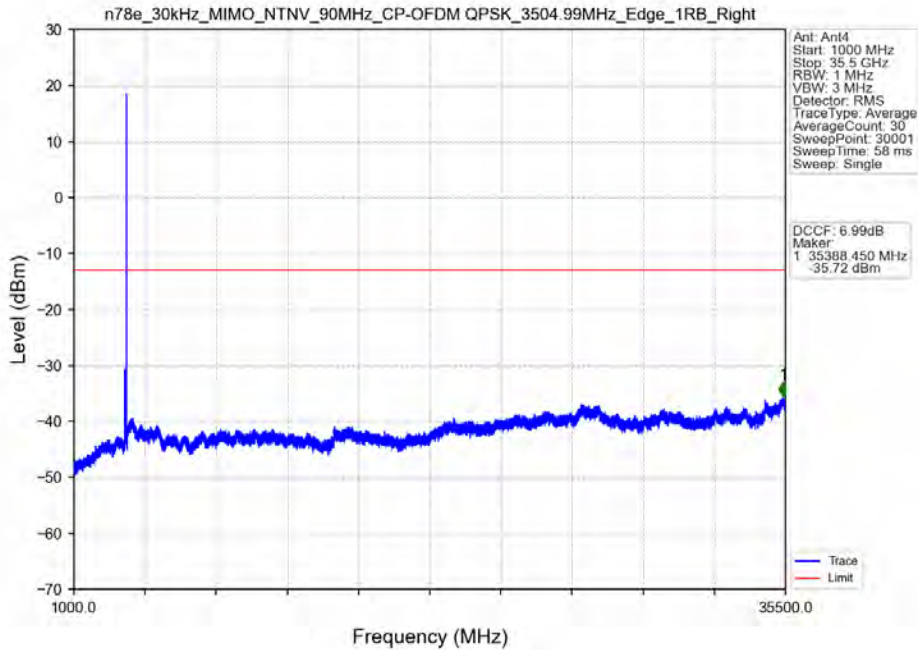
n78e_30kHz_MIMO_NTNV_90MHz_CP-OFDM QPSK_3504.99MHz_Edge_1RB_Right
